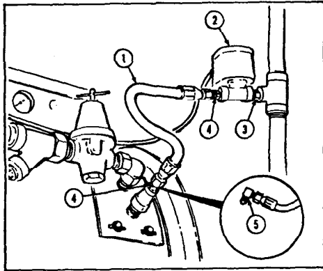
△ FIG.1- TYPICAL PARTS ARRANGEMENT FOR MODELS INDICATED BY SYMBOL
