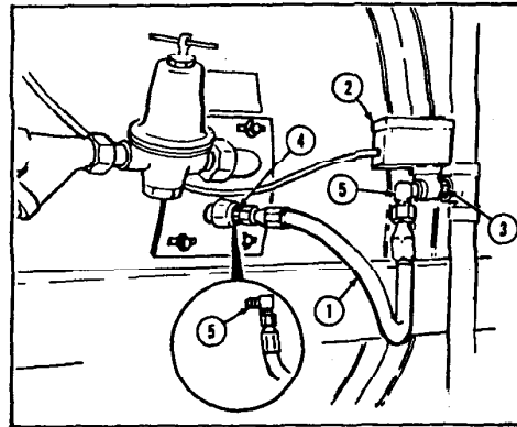
▲ FIG.2- TYPICAL PARTS ARRANGEMENT FOR MODELS INDICATED BY SYMBOL
