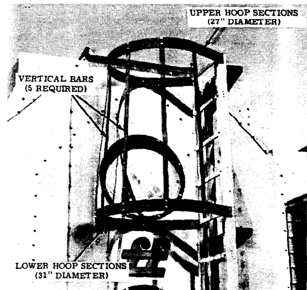
FIG. 2 - REAR SAFETY CAGE - BOTTOM MODULES
