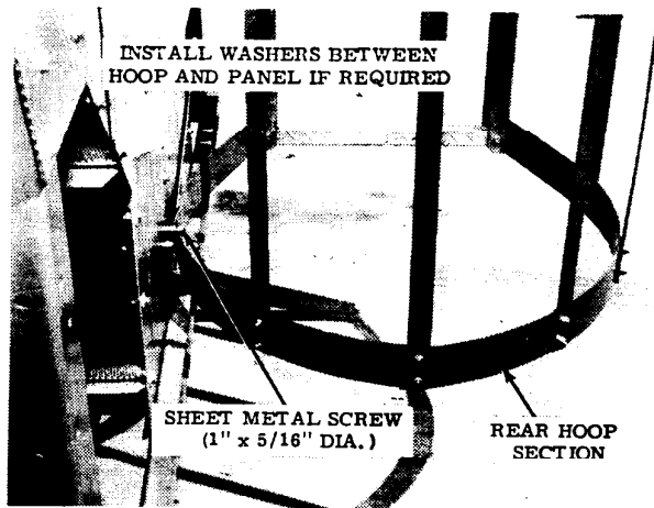
FIG. 4 - CONNECTING REAR HOOPS TO DRYER
