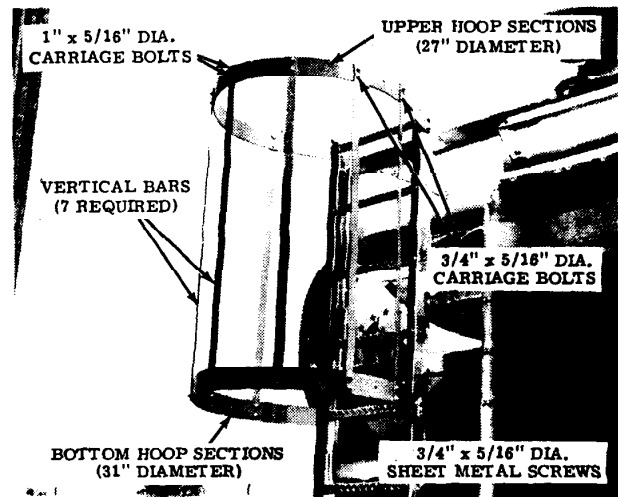
FIG. 1 - FRONT SAFETY CAGE INSTALLED
