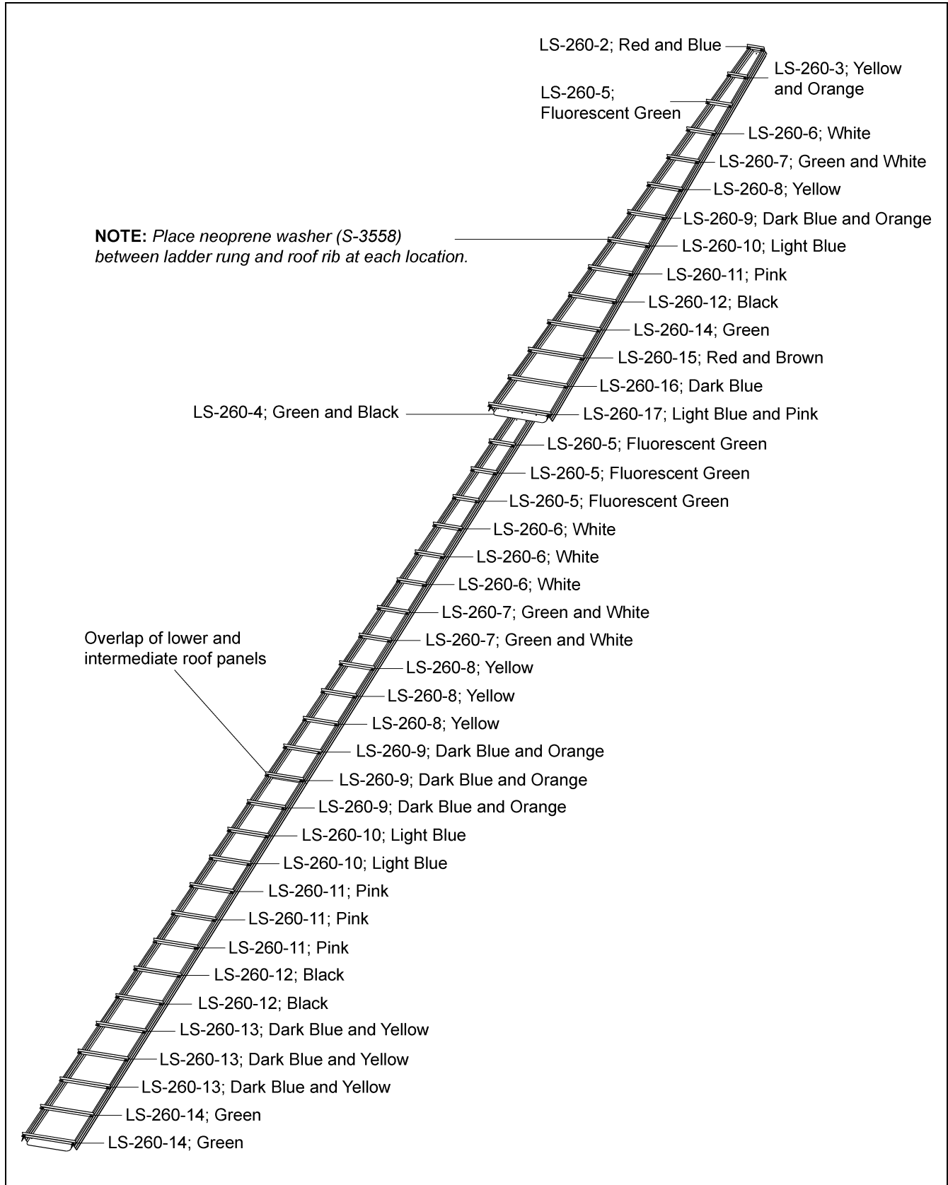
Figure 1 Roof Ladder Rung
