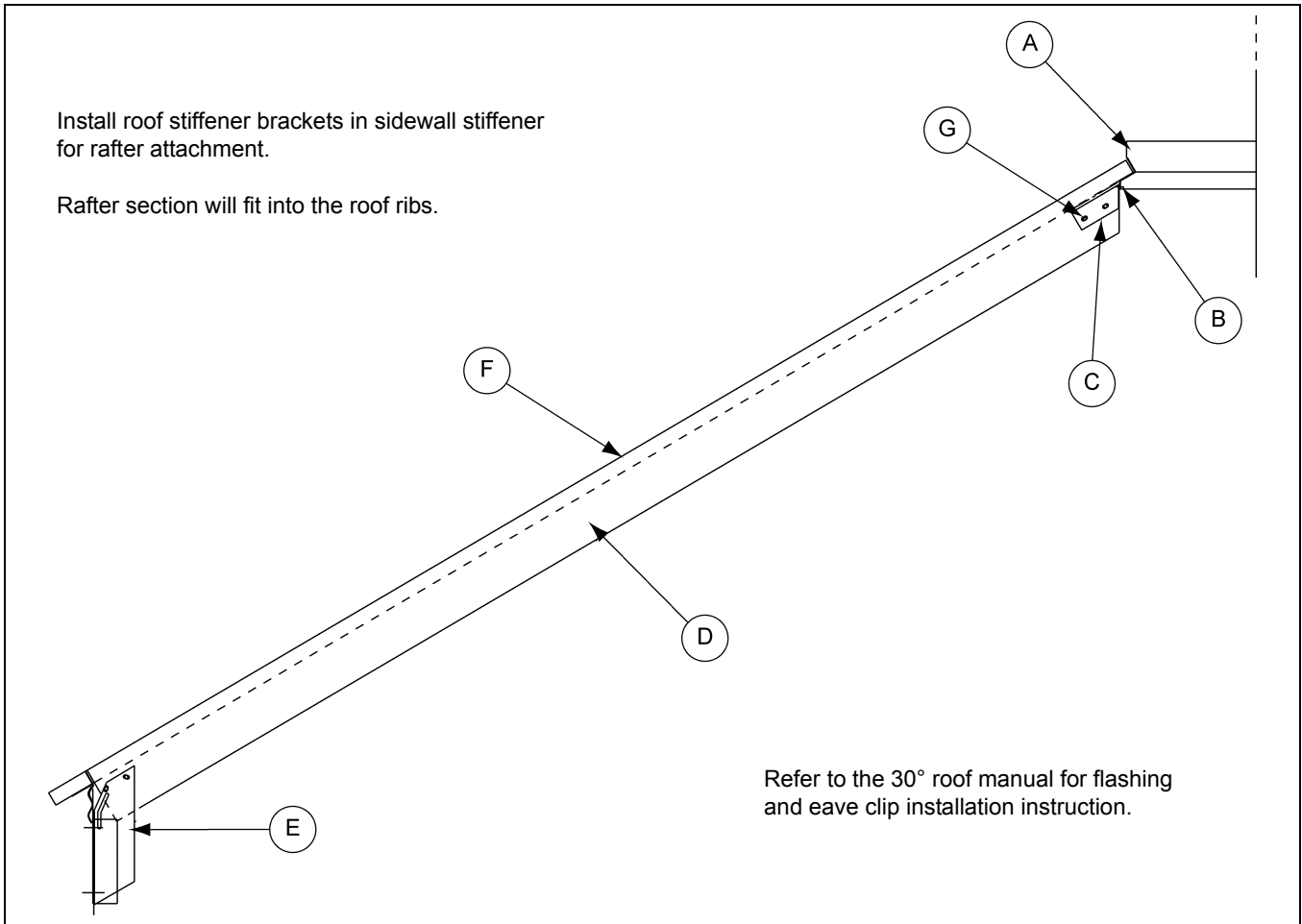
Figure 1 Specification for 15' and 18' Roof Rafter Assembly Detail
