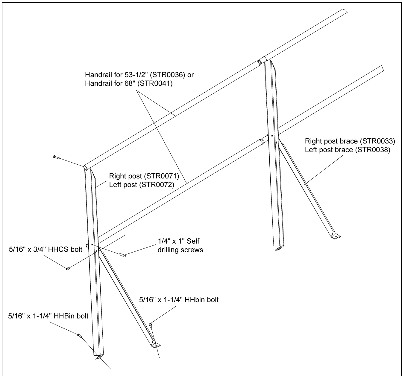
Figure 1 Bin Roof Handrail Assembly
