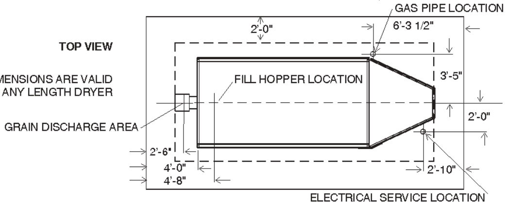
ELECTRICAL SERVICE LOCATION
