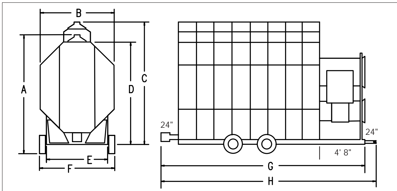
Diagram of dryer dimensions.
