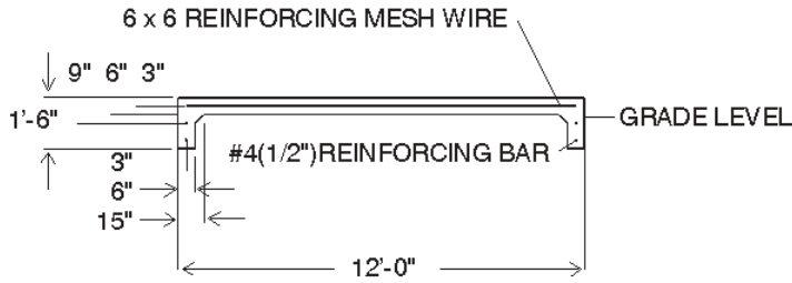
FOUNDATION CROSS SECTION
