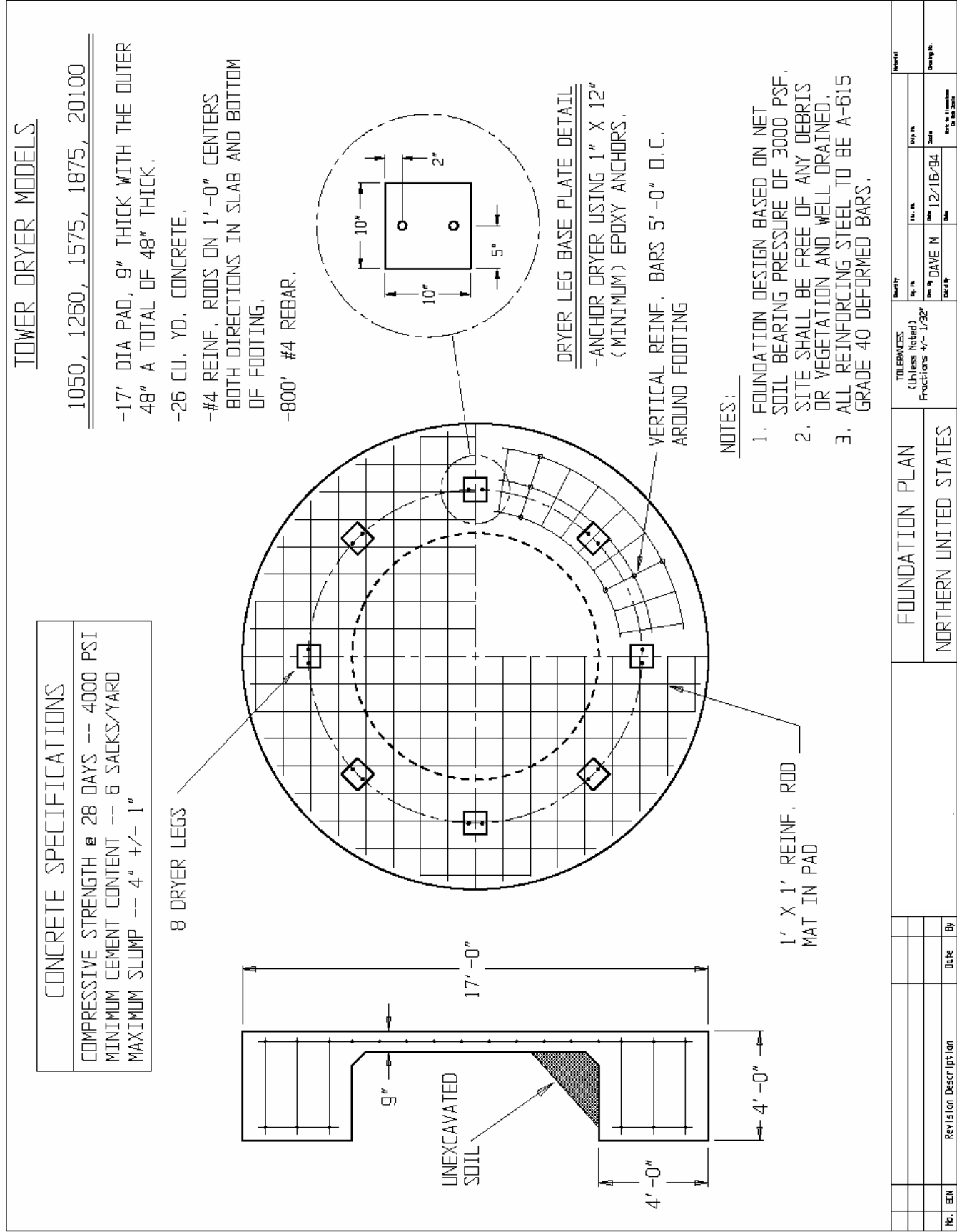
Figure 2.2 Northern United States Foundation For Dryer Sizes Up To 20100
