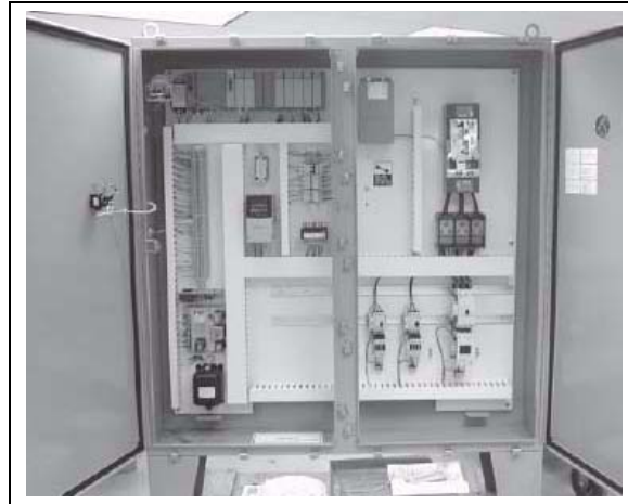
Figure 3C PLC Dryer Control Panel
