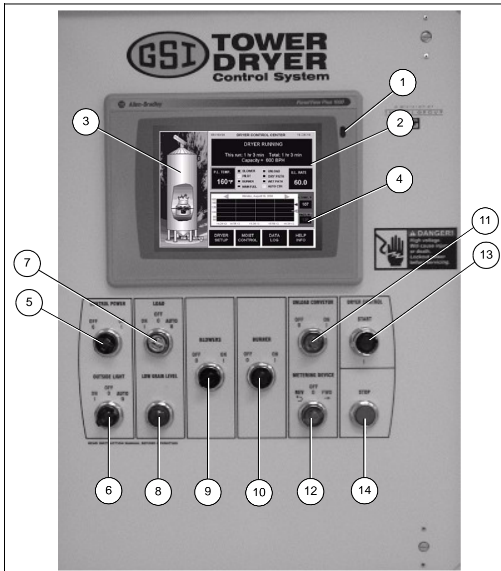
Figure 3D PLC Control Screen
