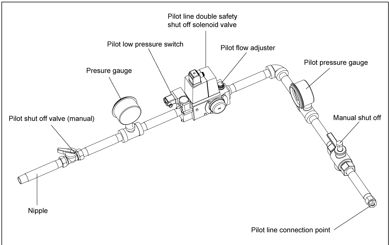
Figure 7G Pilot Section
