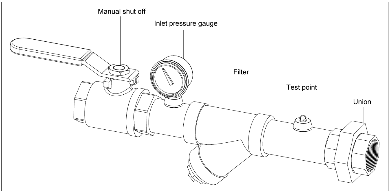
Figure 7C Inlet Section
