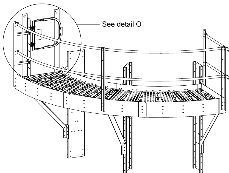
Roof hatch catwalk
