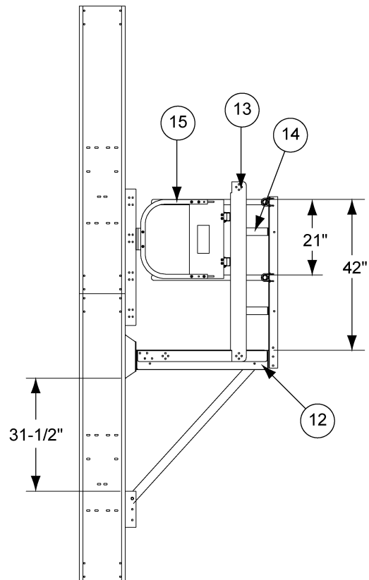
View B-B
