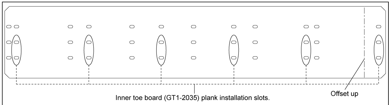
Figure 4K 18' Inner Toe Board (GT1-2035)
