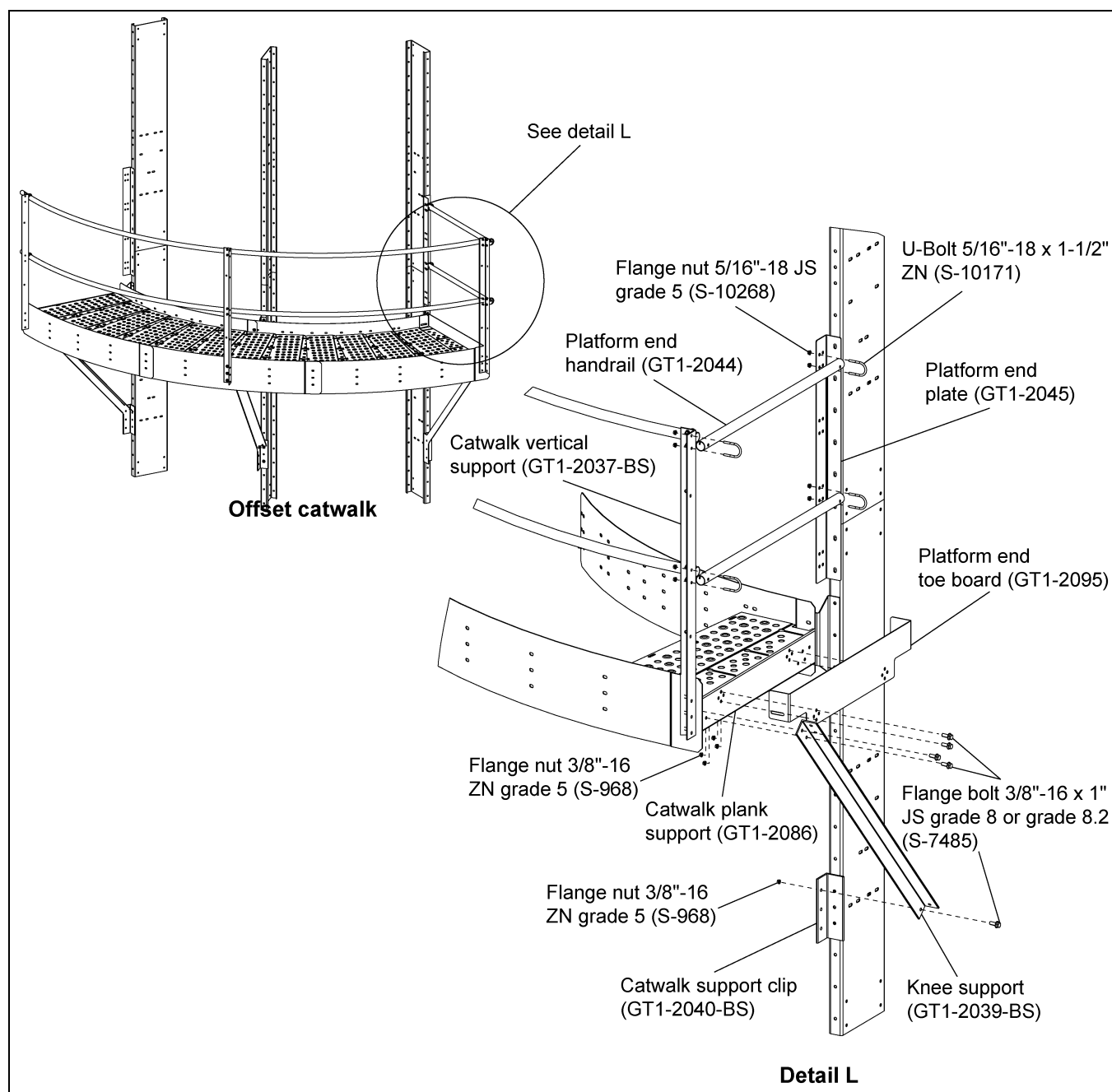
Figure 6V Offset Platform End Handrail (GT1-2044) Installation
