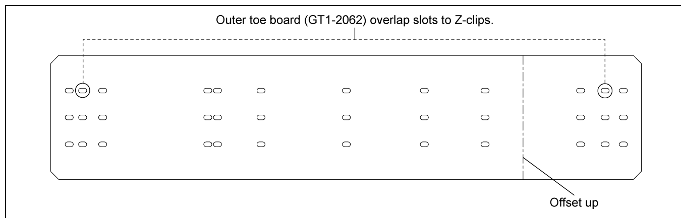
Figure 5E 18' Outer Toe Board (GT1-2062)
