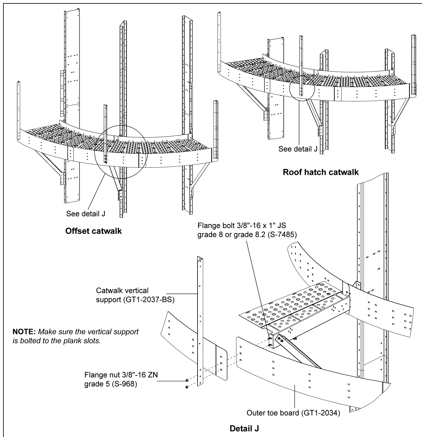
Figure 6T Outer Toe Board (GT1-2034) and Vertical Support (GT1-2037-BS) Installation for Offset and Roof Hatch Catwalks
