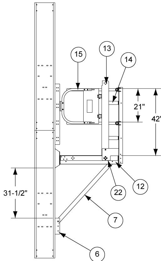
View B-B
