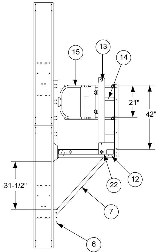
View B-B
