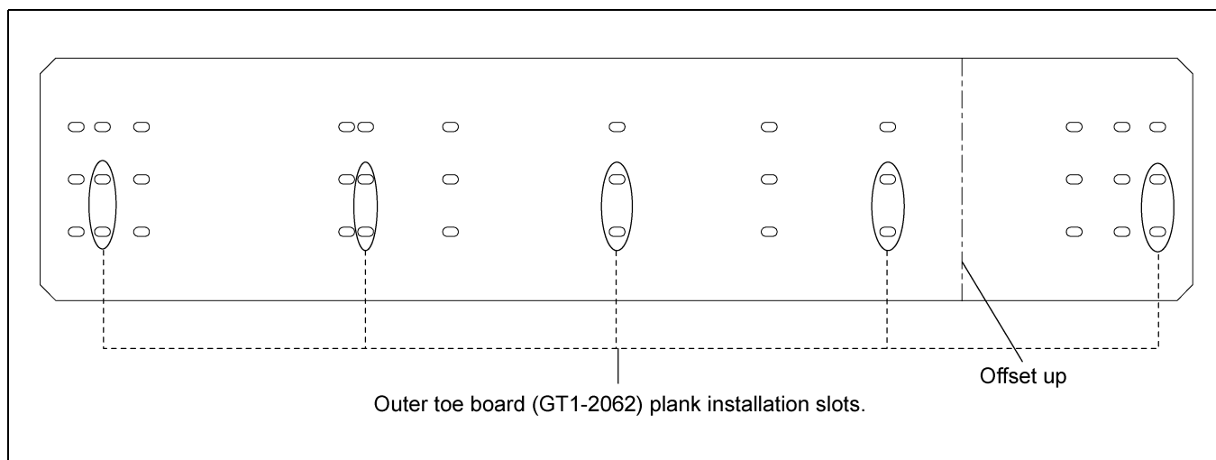
Figure 5H 24' Outer Toe Board (GT1-2062)
