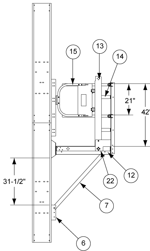
View B-B
