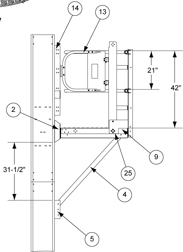
Section A
