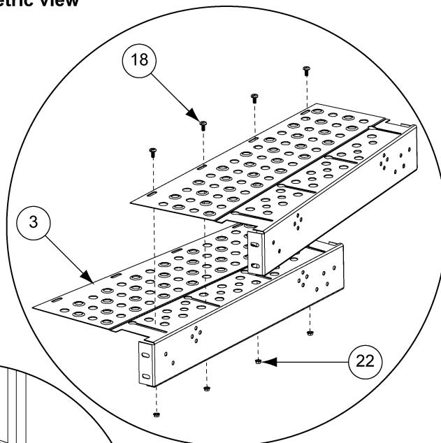
Detail D
