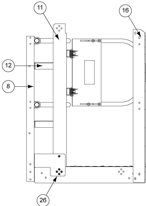
Section B
