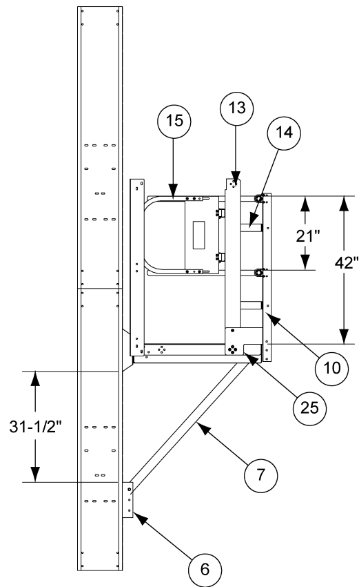
View B-B
