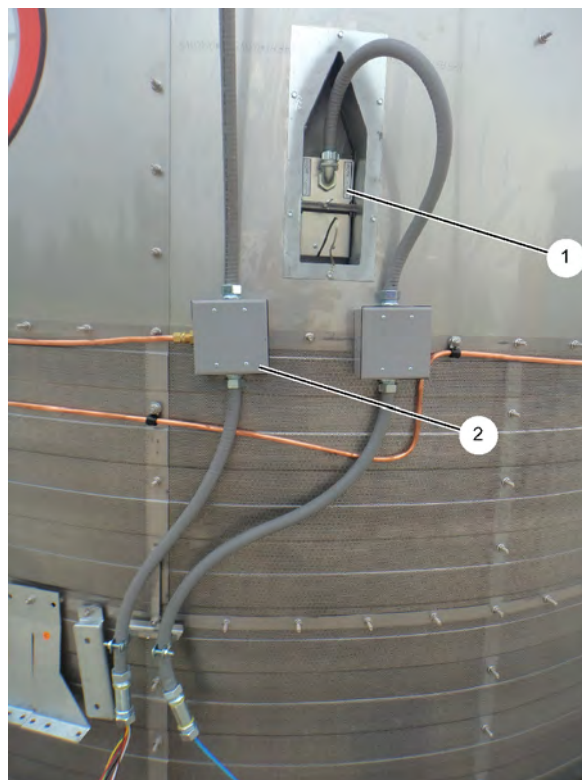
Figure 10-5 Outside Overheat Sensor (GT4-0148) and Wet Moisture Sensor (GT4-7187)
