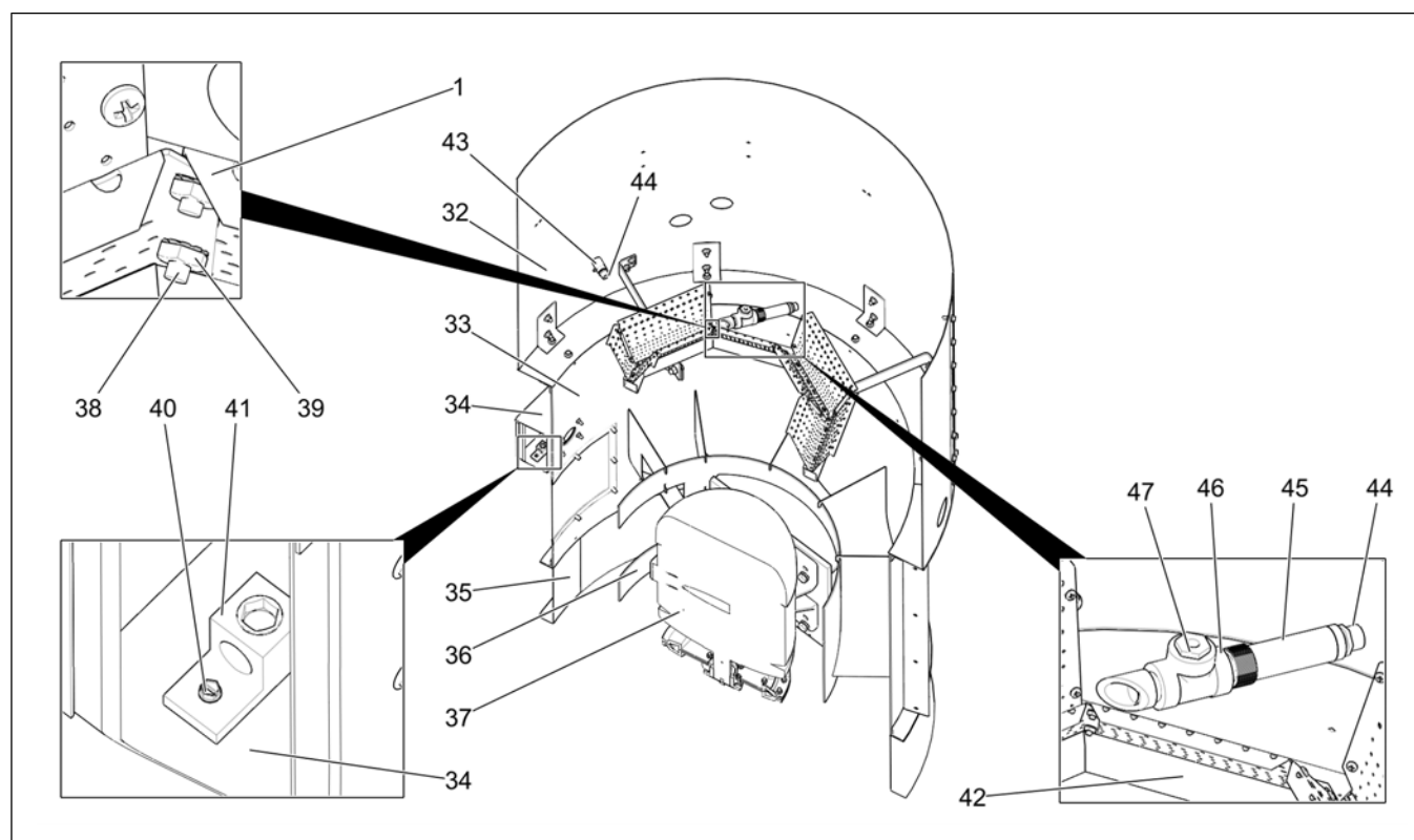
Figure 5-5 Burner Blower Assembly (GT4-9007) (Continued)
