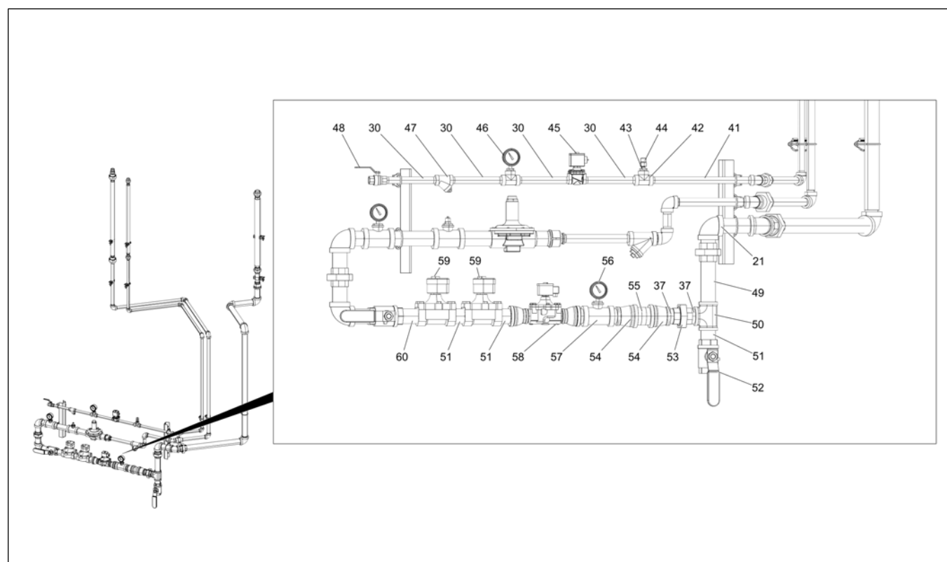
Figure 5-23 1015 Pipetrain – LP (GT4-7057) (Continued)
