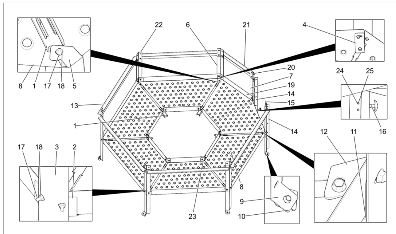
Figure 1-5 Peak Walk Around Catwalk Assembly (GT4-7202)
