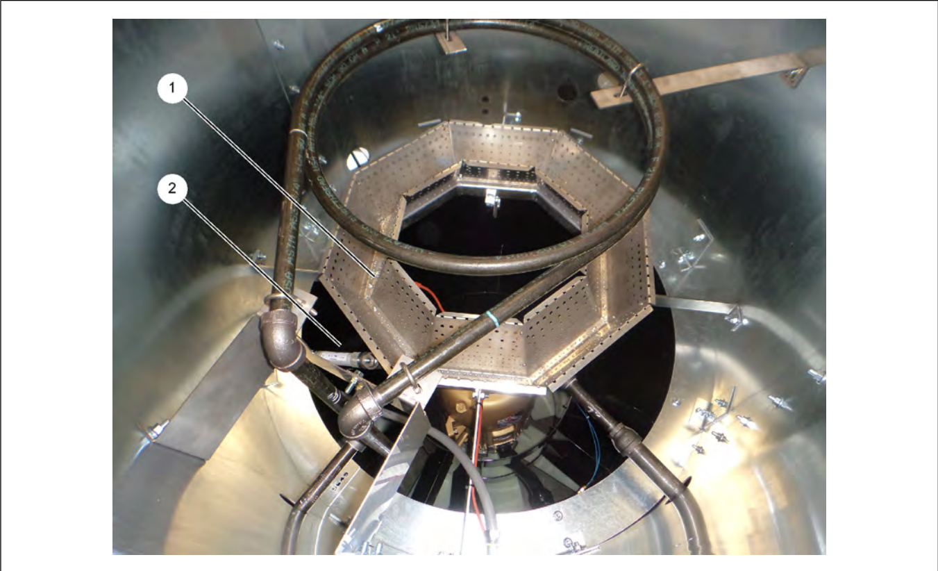
Figure 10-2 Ignitor (HH-1485) and UV Flame Sensor (GT3-1548)
