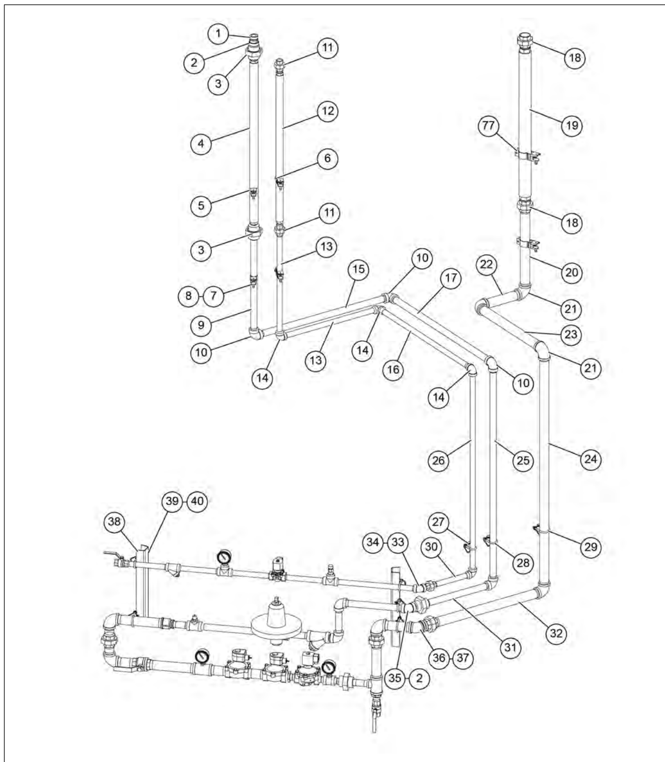
Figure 5-16 1010/1012 Pipetrain – LP (GT4-7043)
