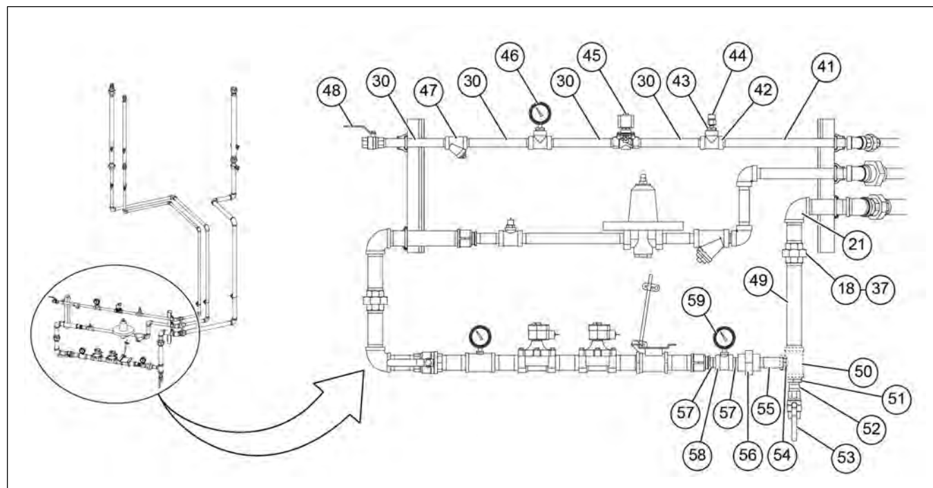
Figure 5-14 1008 Pipetrain – LP, Modulating Valve (GT4-7151) (Continued)
