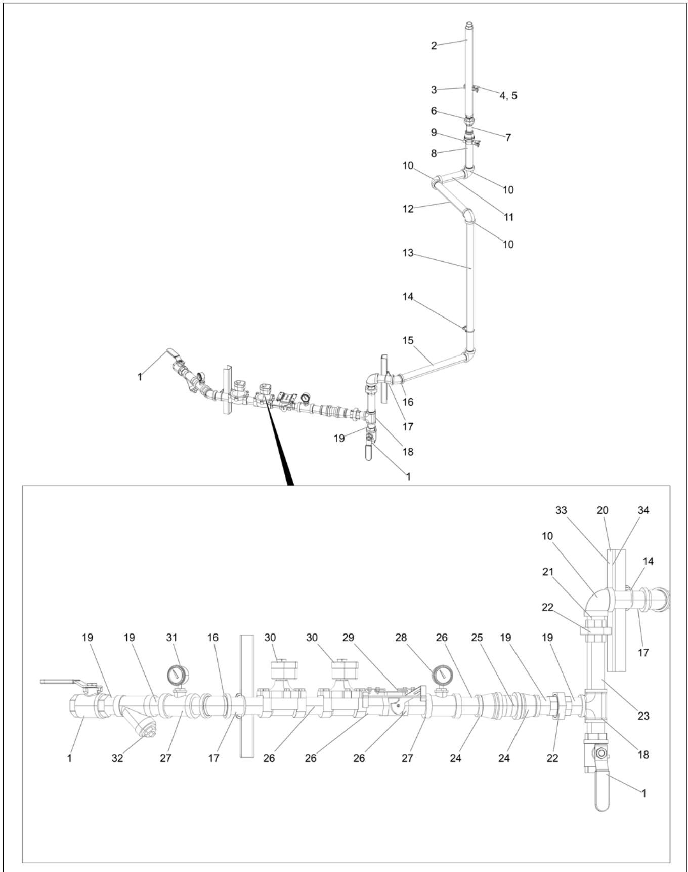
Figure 5-37 1015 Pipetrain – NG, Modulating Valve (GT4-7157)
