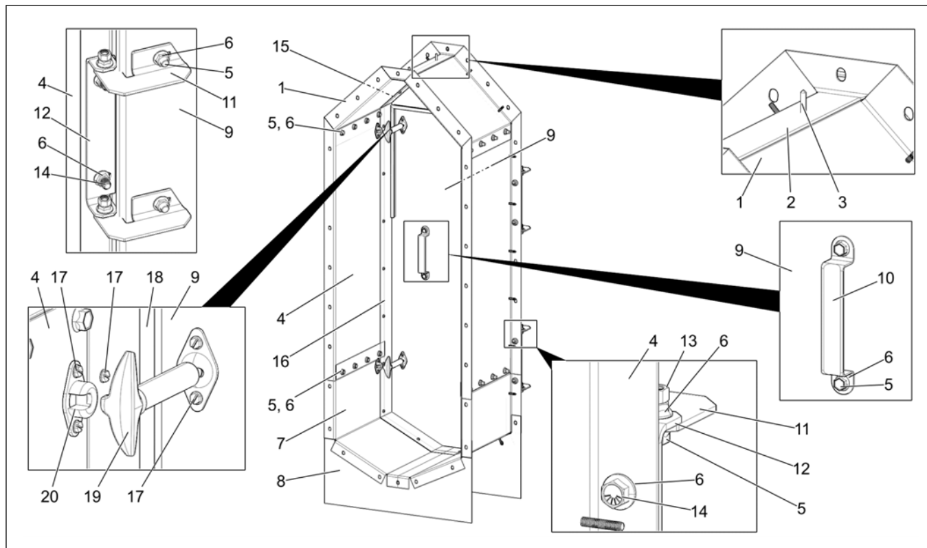
Figure 4-3 18 in. Door Kit Assembly (GT4-5653)
