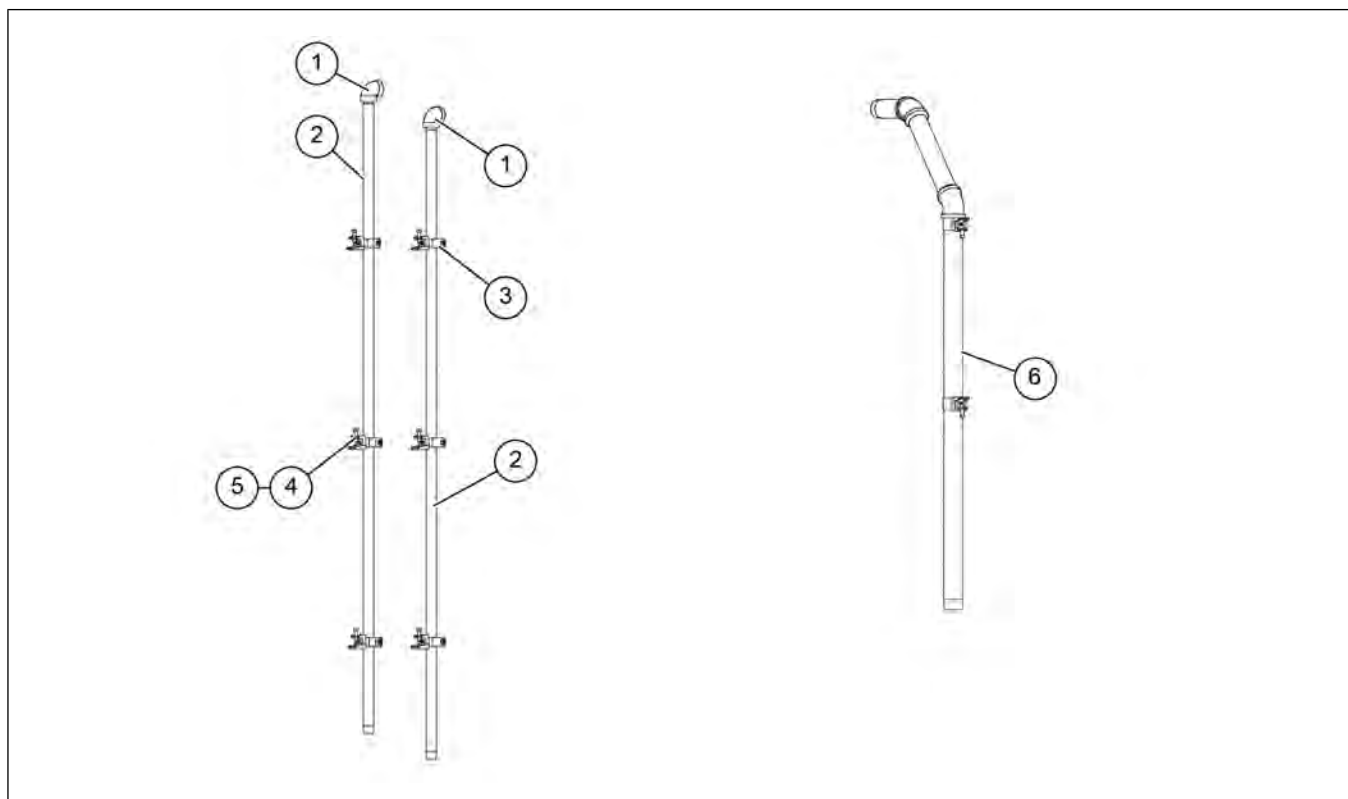
Figure 5-9 1015 Adjustable Pipetrain – LP (GT4-7195)
