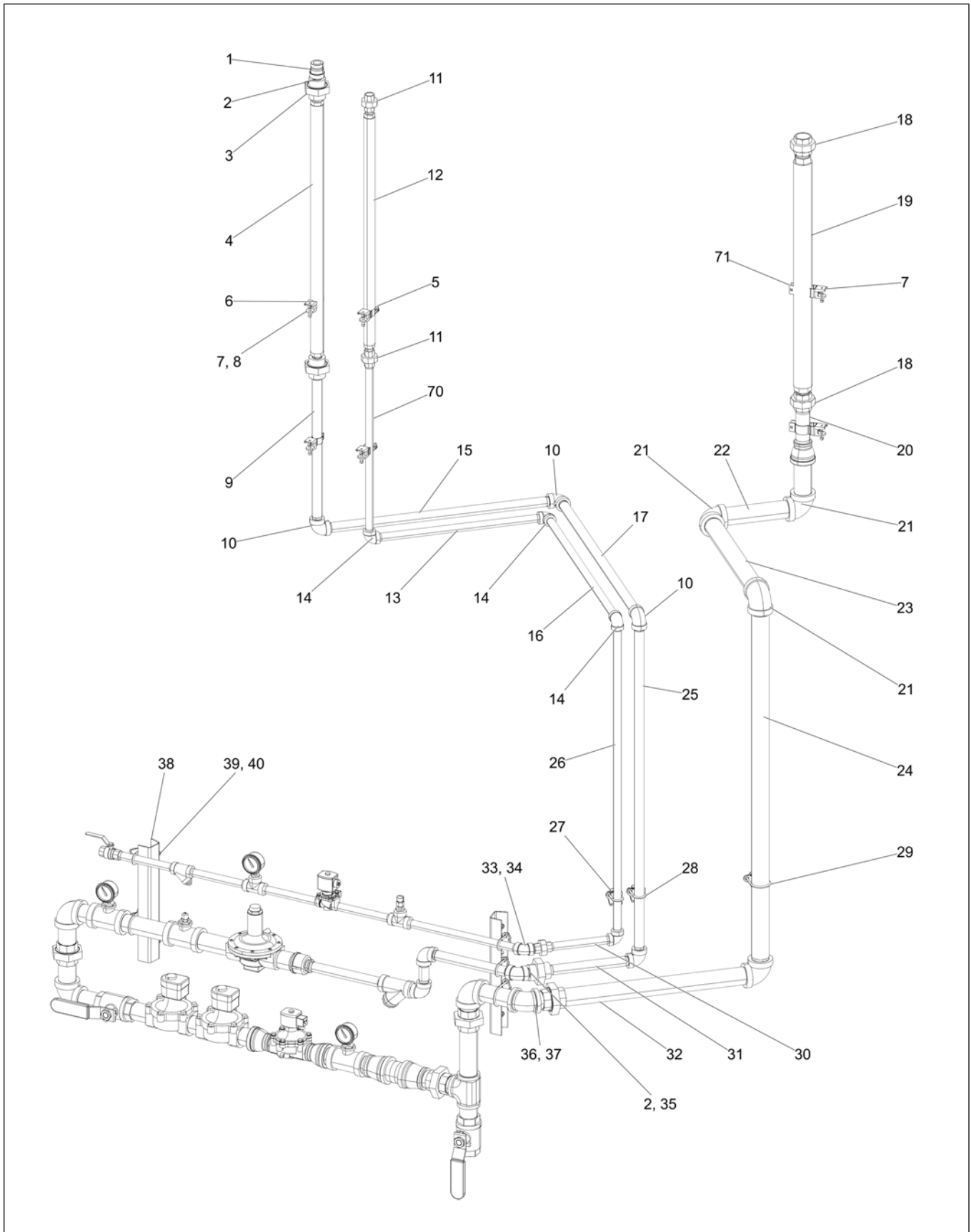
Figure 5-22 1015 Pipetrain – LP (GT4-7057)
