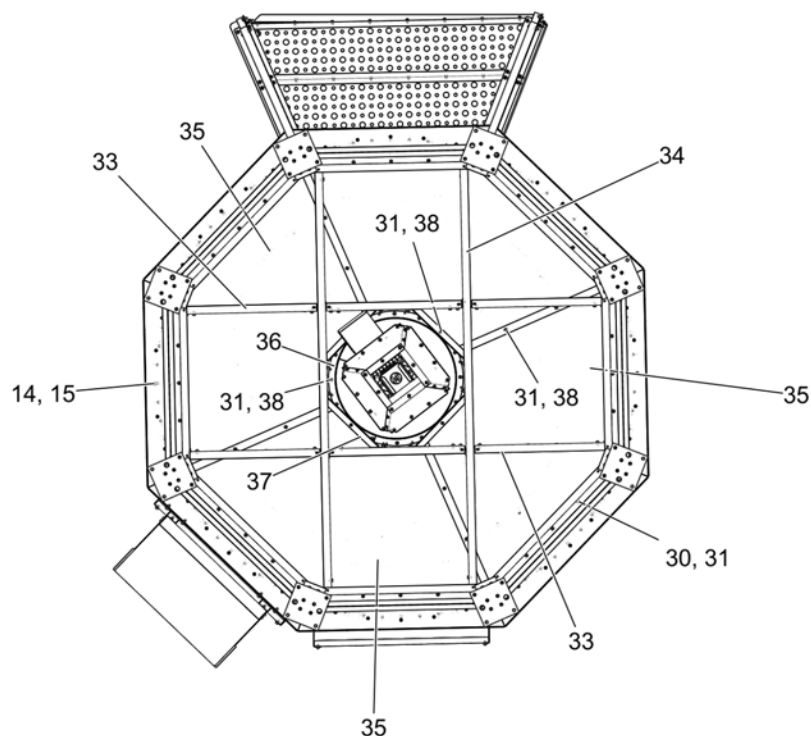
Figure 6-3 Flat Unload Section (GT4-7003-AC) (Bottom View)
