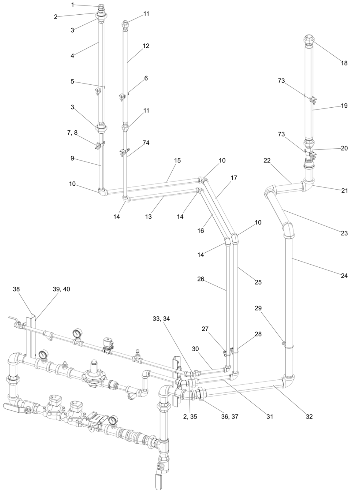
Figure 5-25 1015 Pipetrain – LP, Modulating Valve (GT4-7062)
