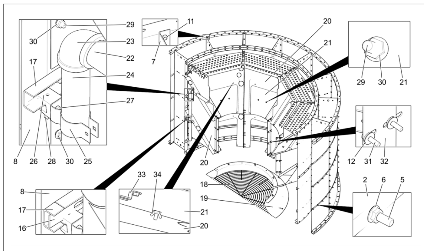
Figure 5-2 Heat Section Complete Assembly (GT4-7027) (Sectioned)
