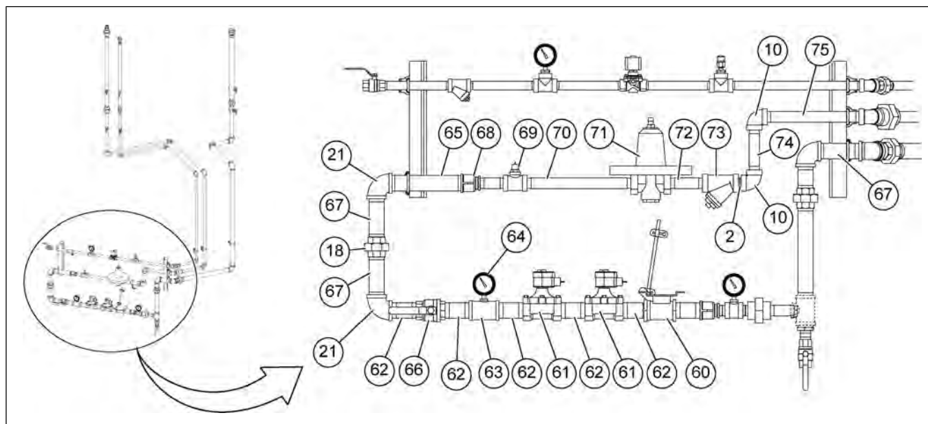
Figure 5-15 1008 Pipetrain – LP, Modulating Valve (GT4-7151) (Continued)
