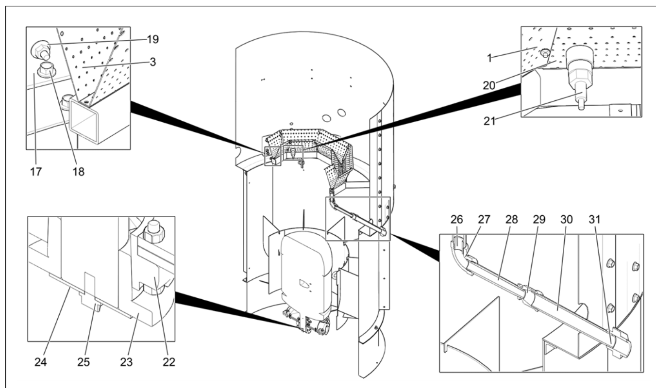
Figure 5-4 Burner Blower Assembly (GT4-9007) (Continued)
