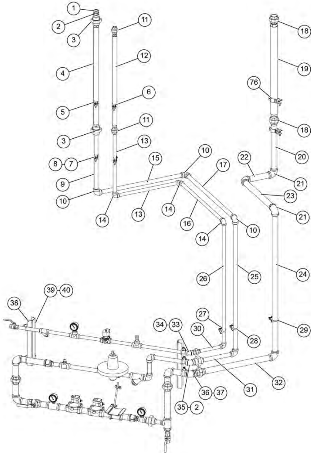
Figure 5-13 1008 Pipetrain – LP, Modulating Valve (GT4-7151)
