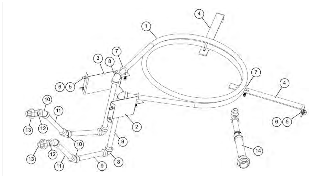
Figure 5-6 1008/1010/1012 Pipetrain – LP (GT4-7040)
