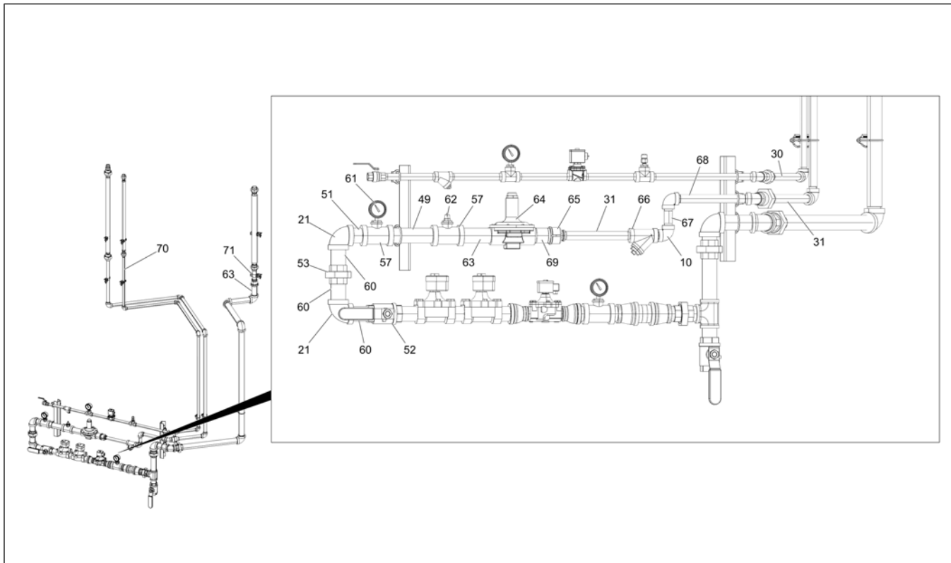
Figure 5-24 1015 Pipetrain – LP (GT4-7057) (Continued)
