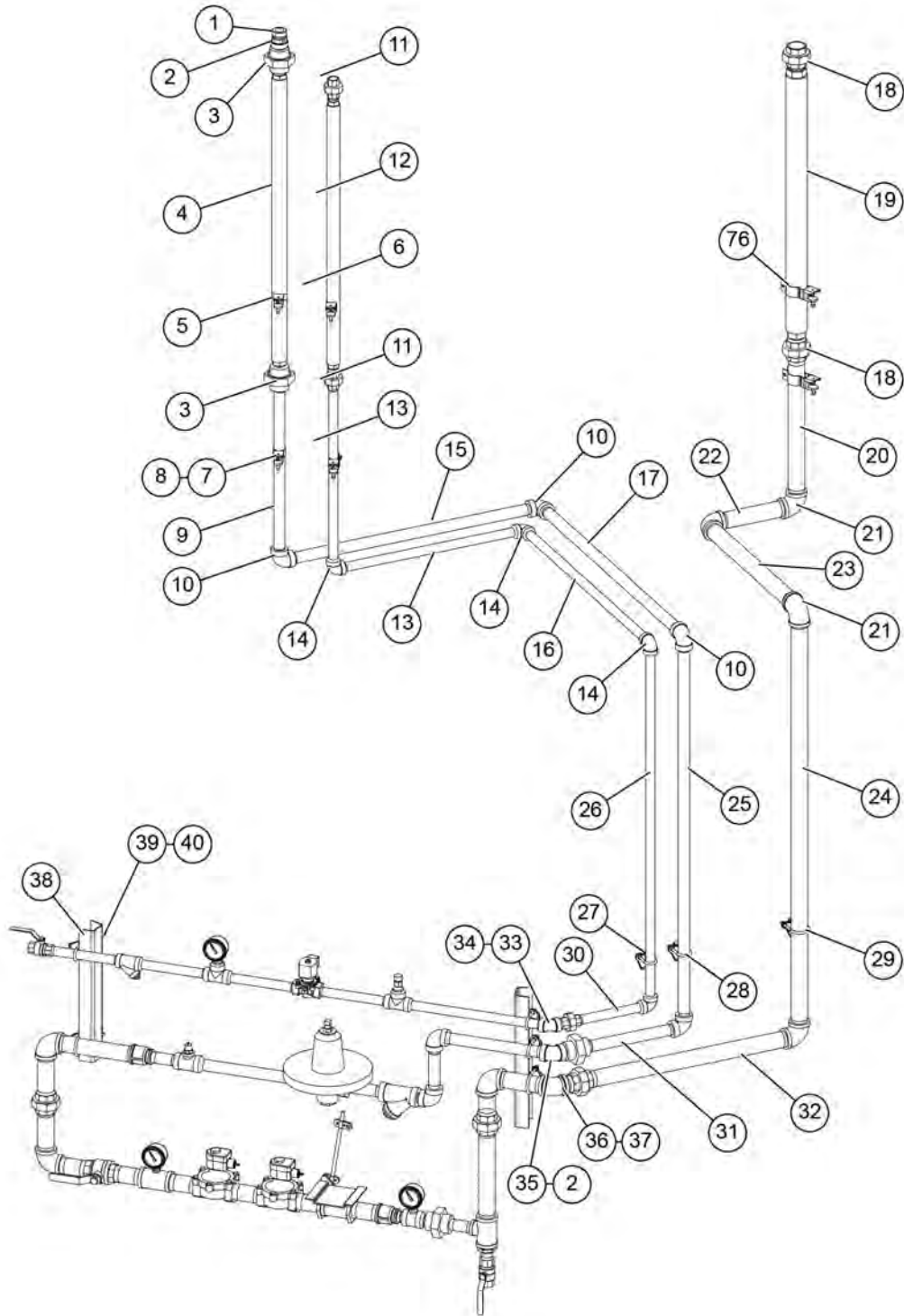
Figure 5-19 1010/1012 Pipetrain – LP, Modulating Valve (GT4-7052)
