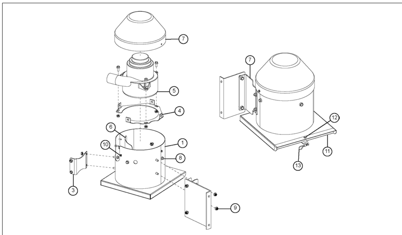
Figure 6-18 Moisture Sampler Blower (GT4-1540)
