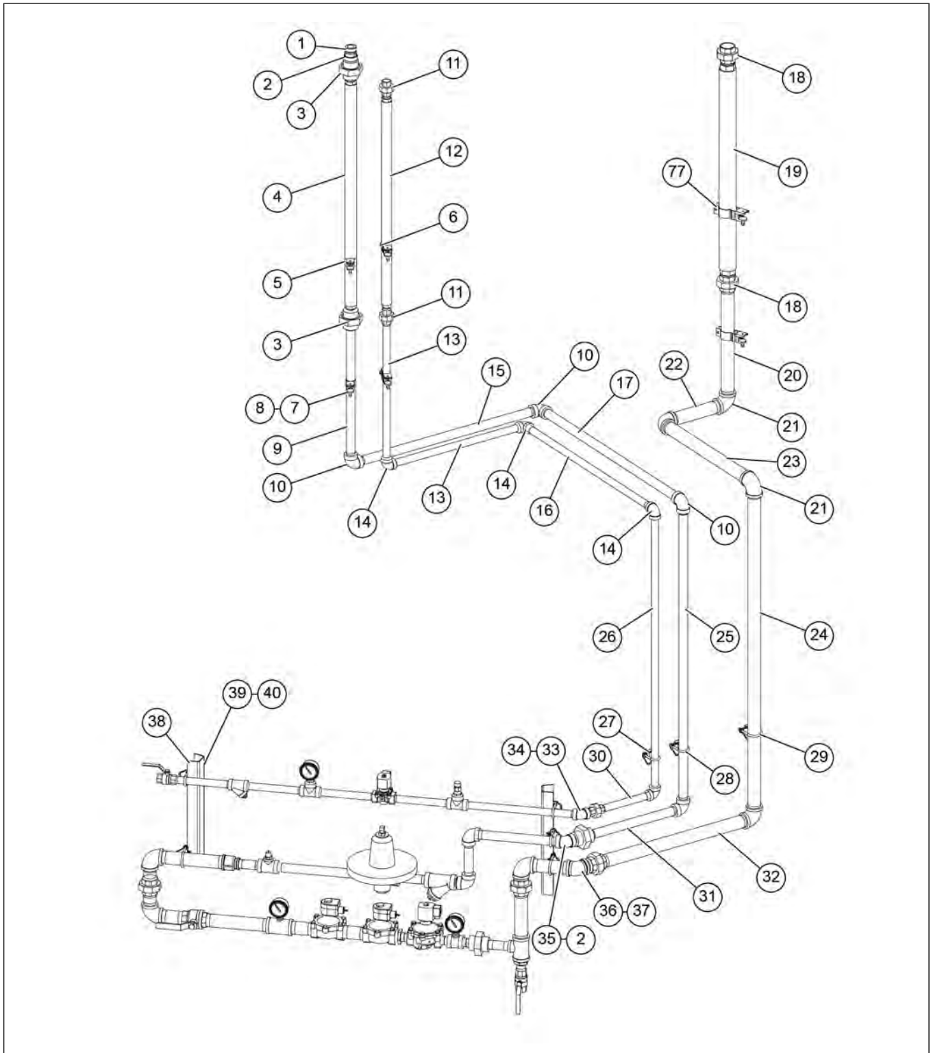
Figure 5-10 1008 Pipetrain – LP (GT4-7042)
