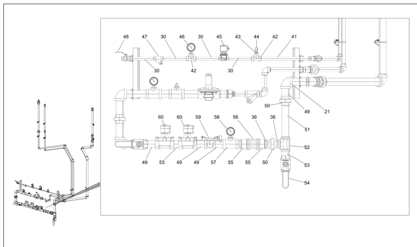
Figure 5-26 1015 Pipetrain – LP, Modulating Valve (GT4-7062) (Continued)
