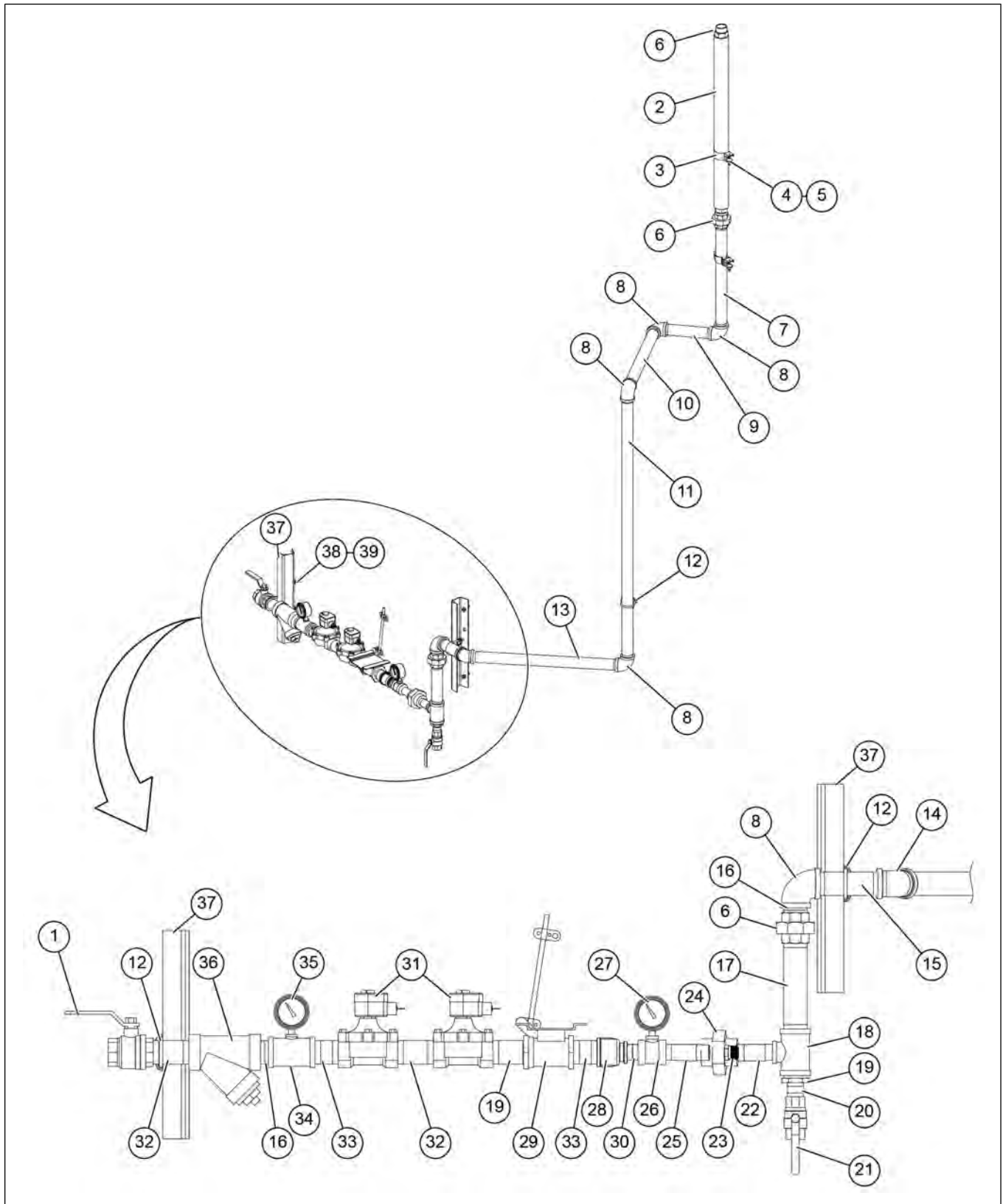
Figure 5-35 1010/1012 Pipetrain – NG, Modulating Valve (GT4-7053)
