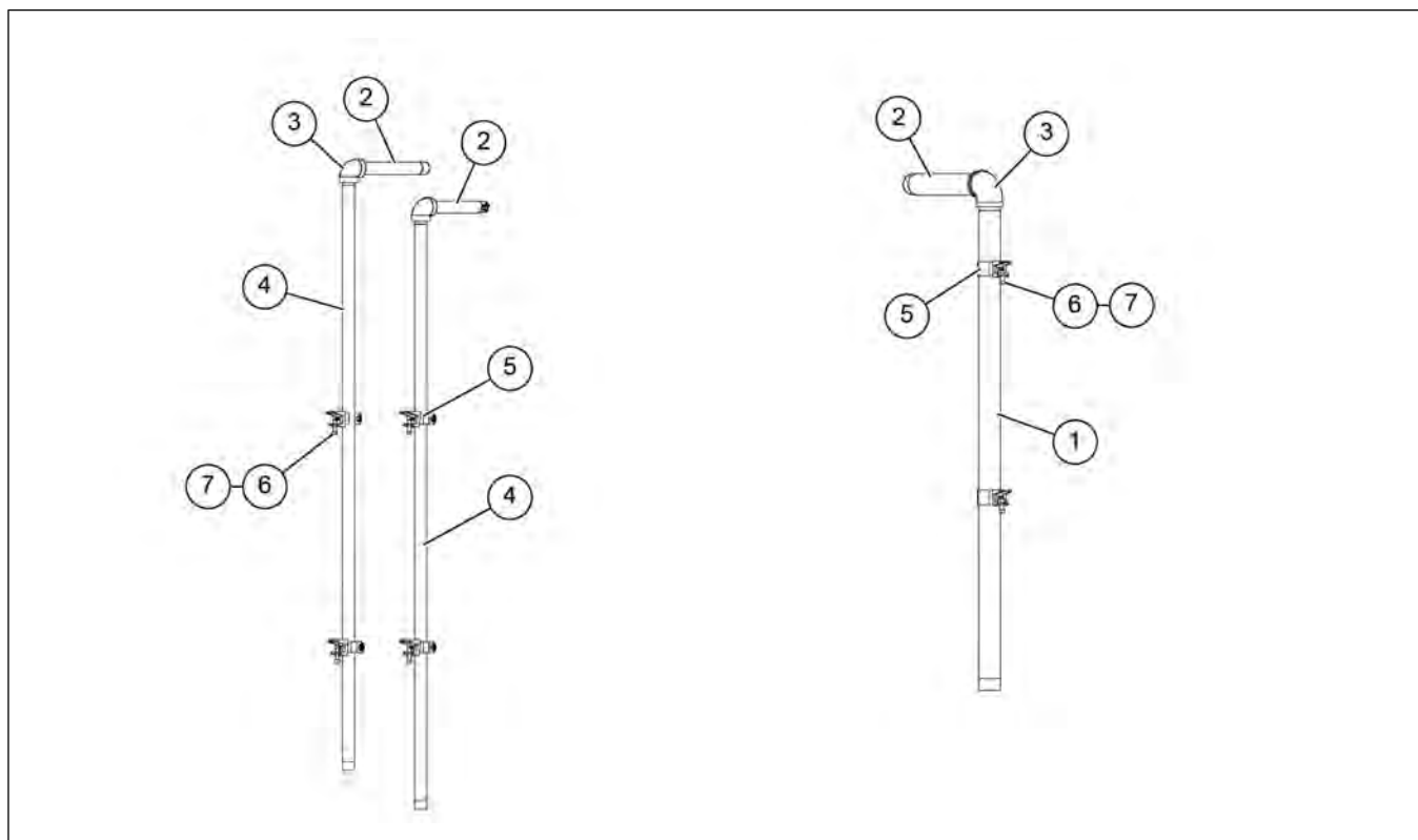
Figure 5-7 1008/1010/1012 Pipetrain – LP (GT4-7041)
