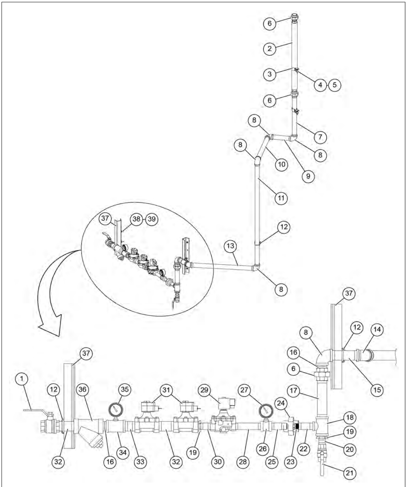
Figure 5-32 1008 Pipetrain – NG (GT4-7046)
