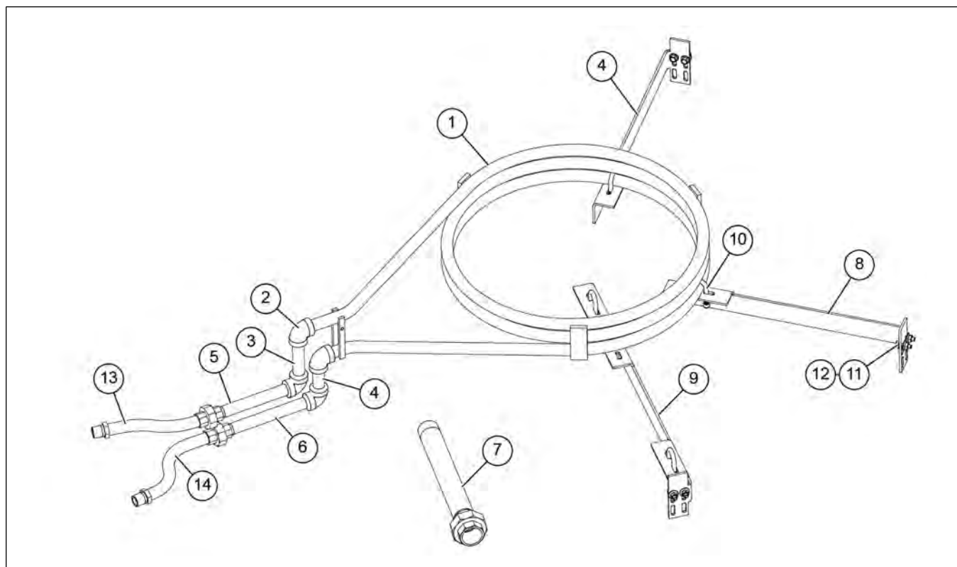
Figure 5-8 1015 Adjustable Pipetrain – LP (GT4-7189)
