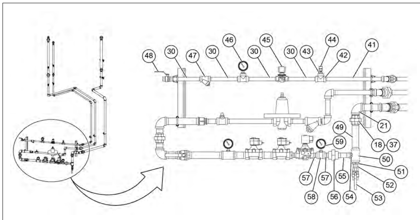
Figure 5-11 1008 Pipetrain – LP (GT4-7042) (Continued)
