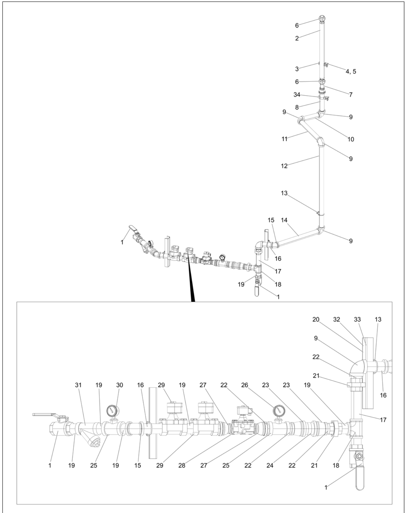
Figure 5-36 1015 Pipetrain – NG (GT4-7059)
