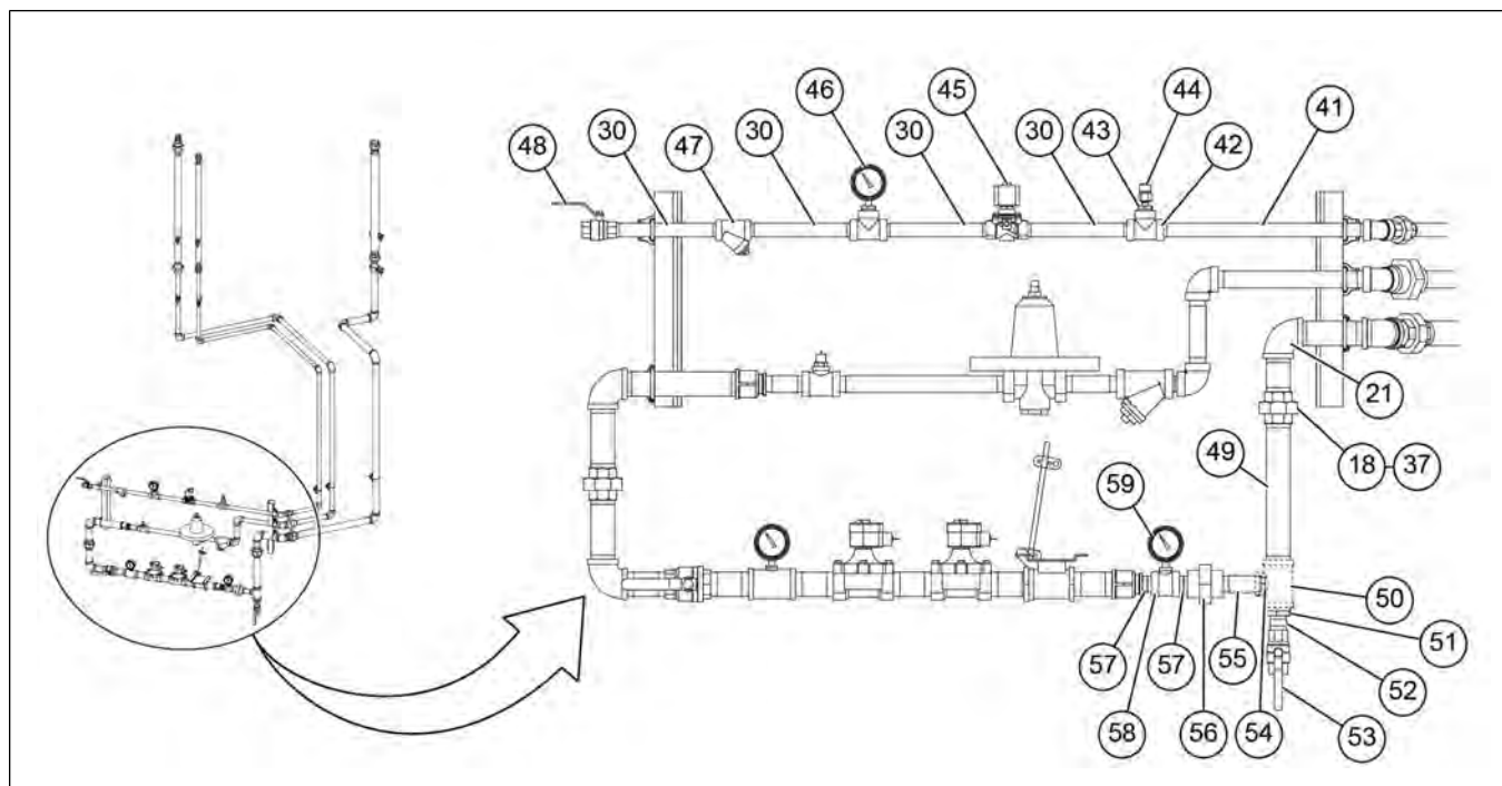
Figure 5-20 1010/1012 Pipetrain – LP, Modulating Valve (GT4-7052) (Continued)
