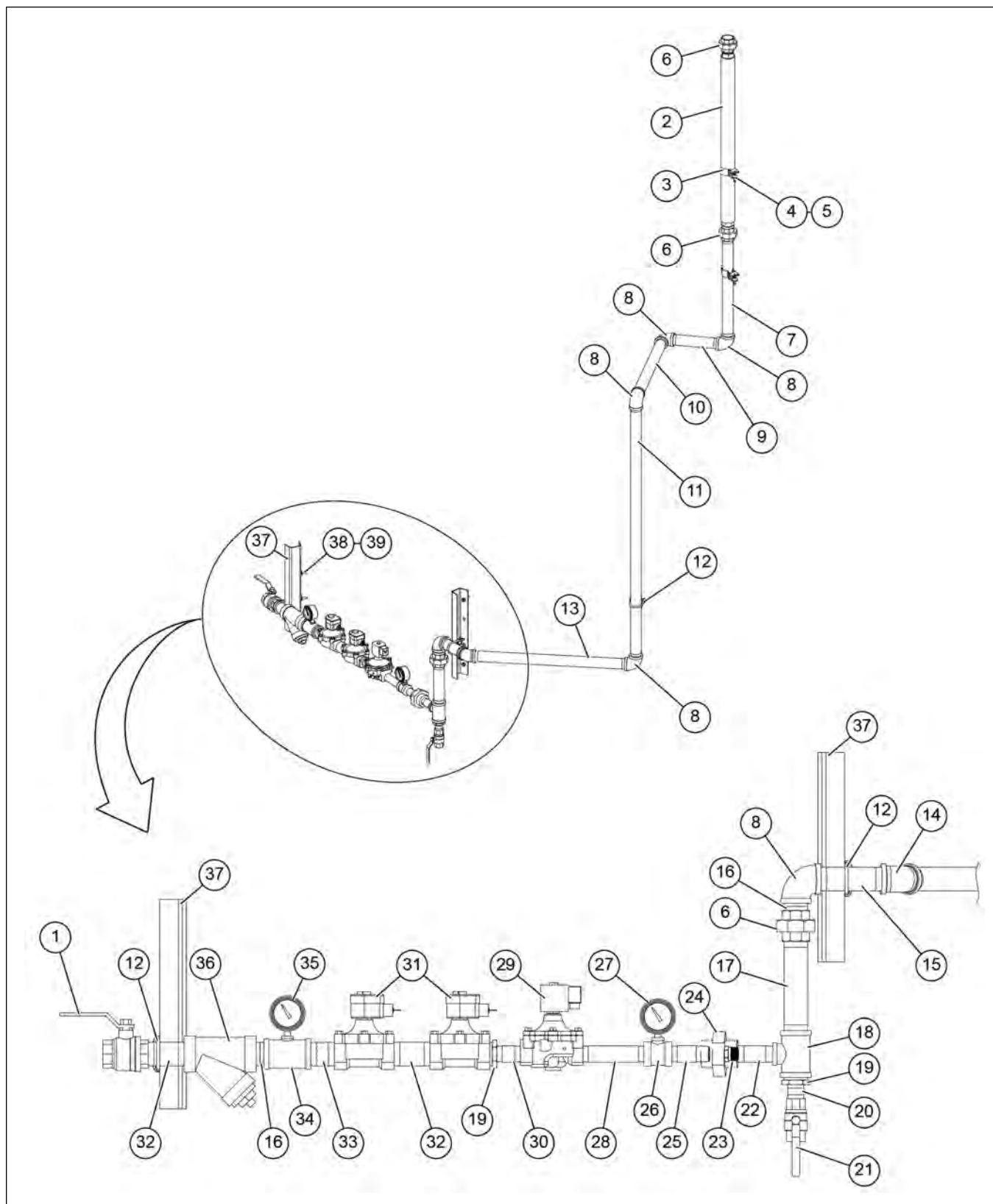
Figure 5-34 1010/1012 Pipetrain – NG (GT4-7047)
