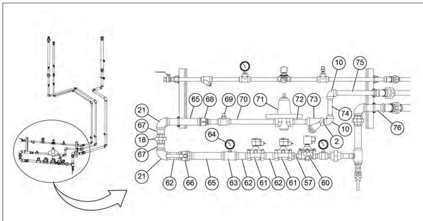
Figure 5-12 1008 Pipetrain – LP (GT4-7042) (Continued)
