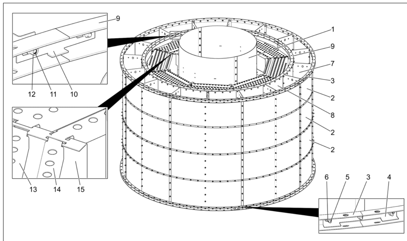
Figure 5-1 Heat Section Complete Assembly (GT4-7027)
