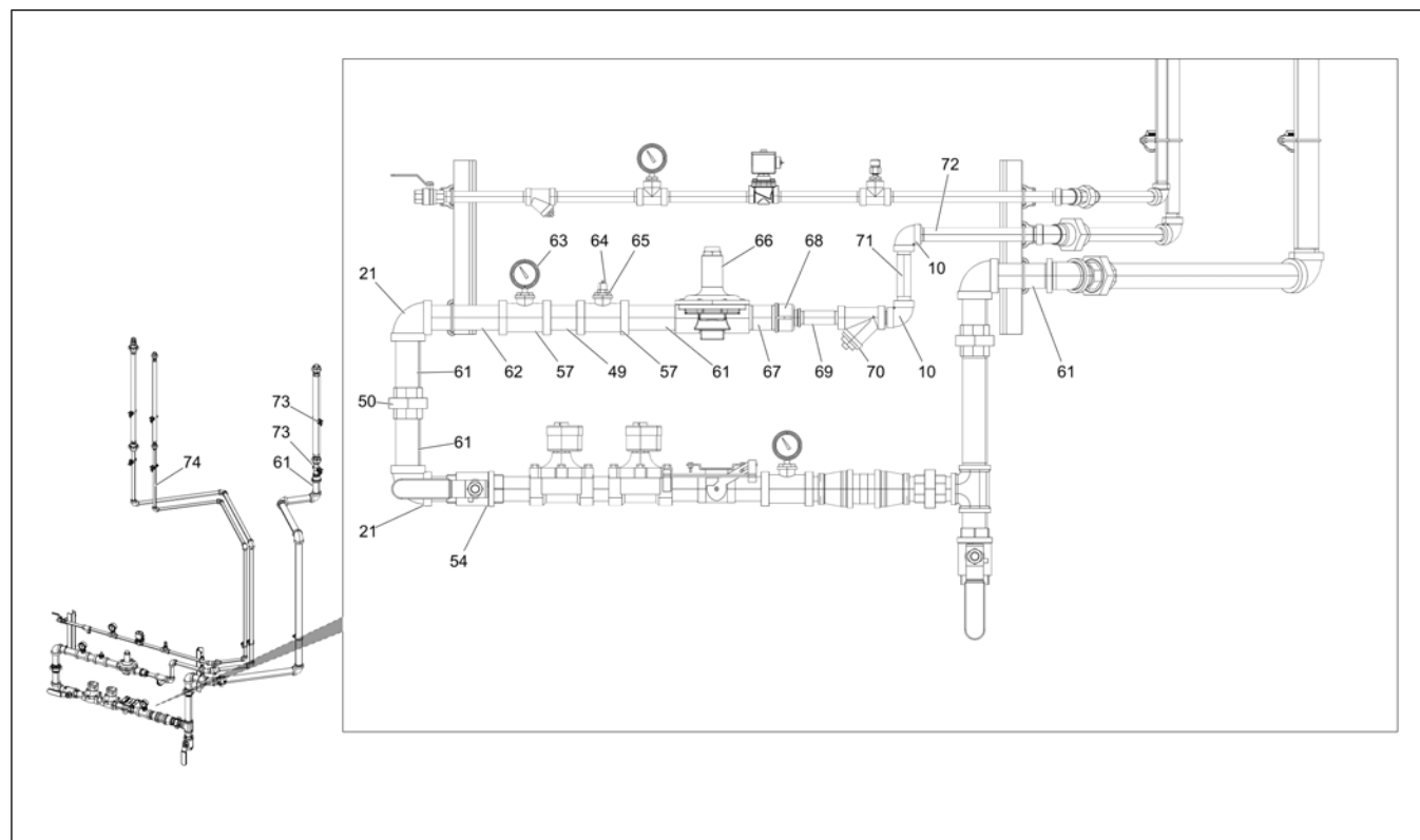
Figure 5-27 1015 Pipetrain – LP, Modulating Valve (GT4-7062) (Continued)
