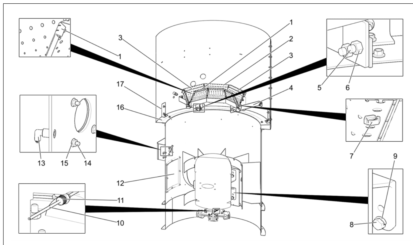
Figure 5-3 Burner Blower Assembly (GT4-9007) (Sectioned)
