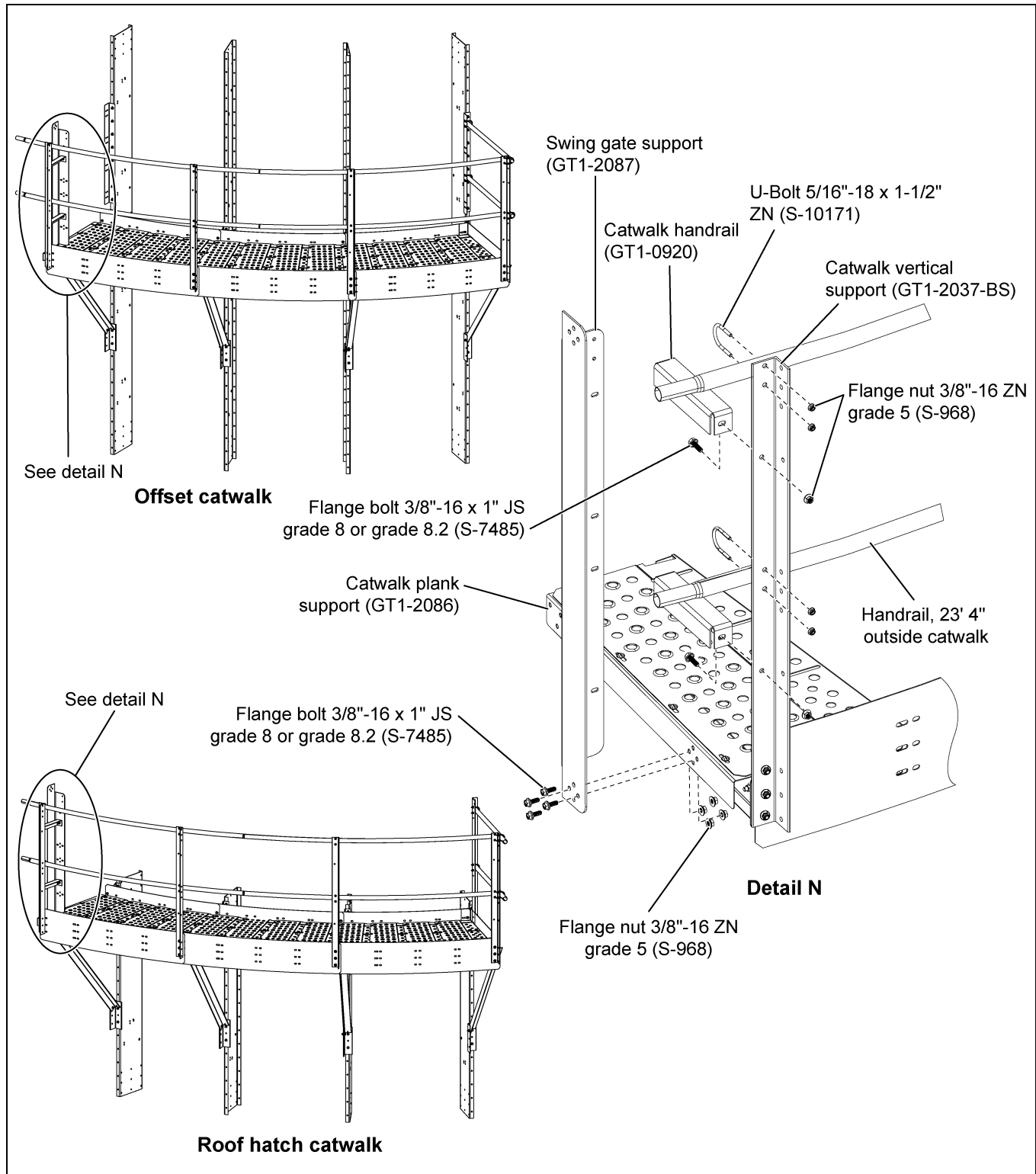
Figure 6X Installing Safety Gate (LDR-5218) to Offset and Roof Hatch Catwalks
