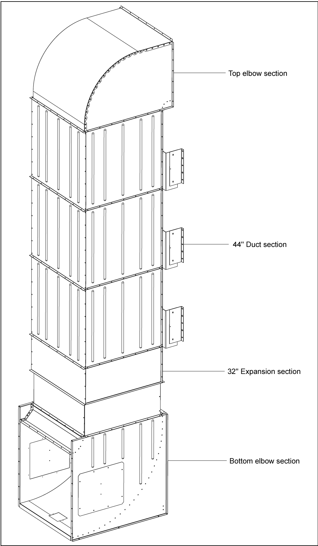
Figure 6A Duct Assembly - (7 Ring Top Dry)
