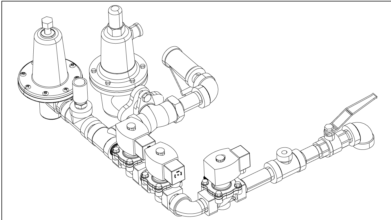
Figure 6A 36" LP Pipe Train
