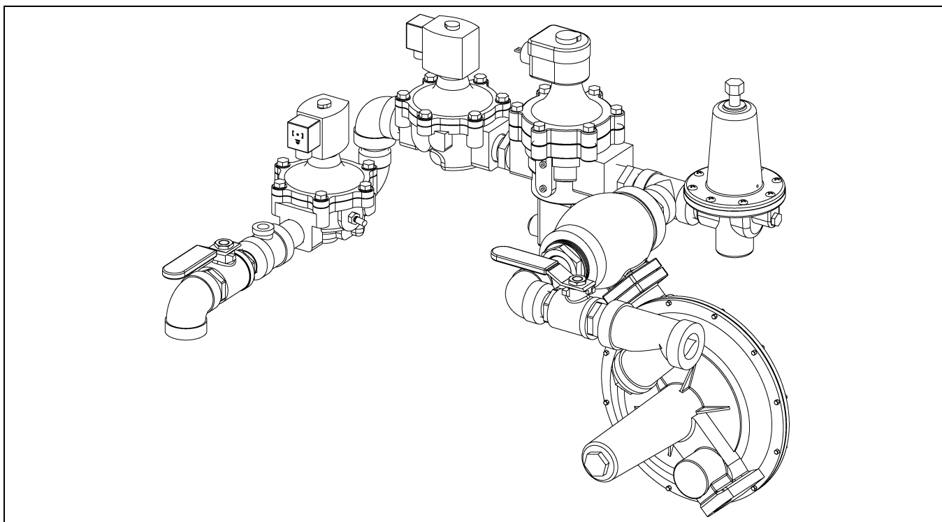
Figure 6D 40"-42" NG Pipe Train
