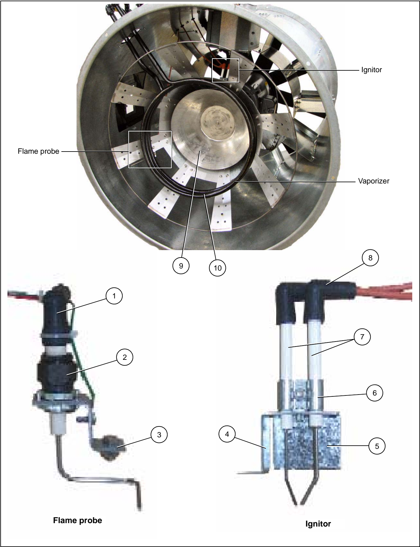
Figure 9B Ignitor and Flame Probe Assemblies
