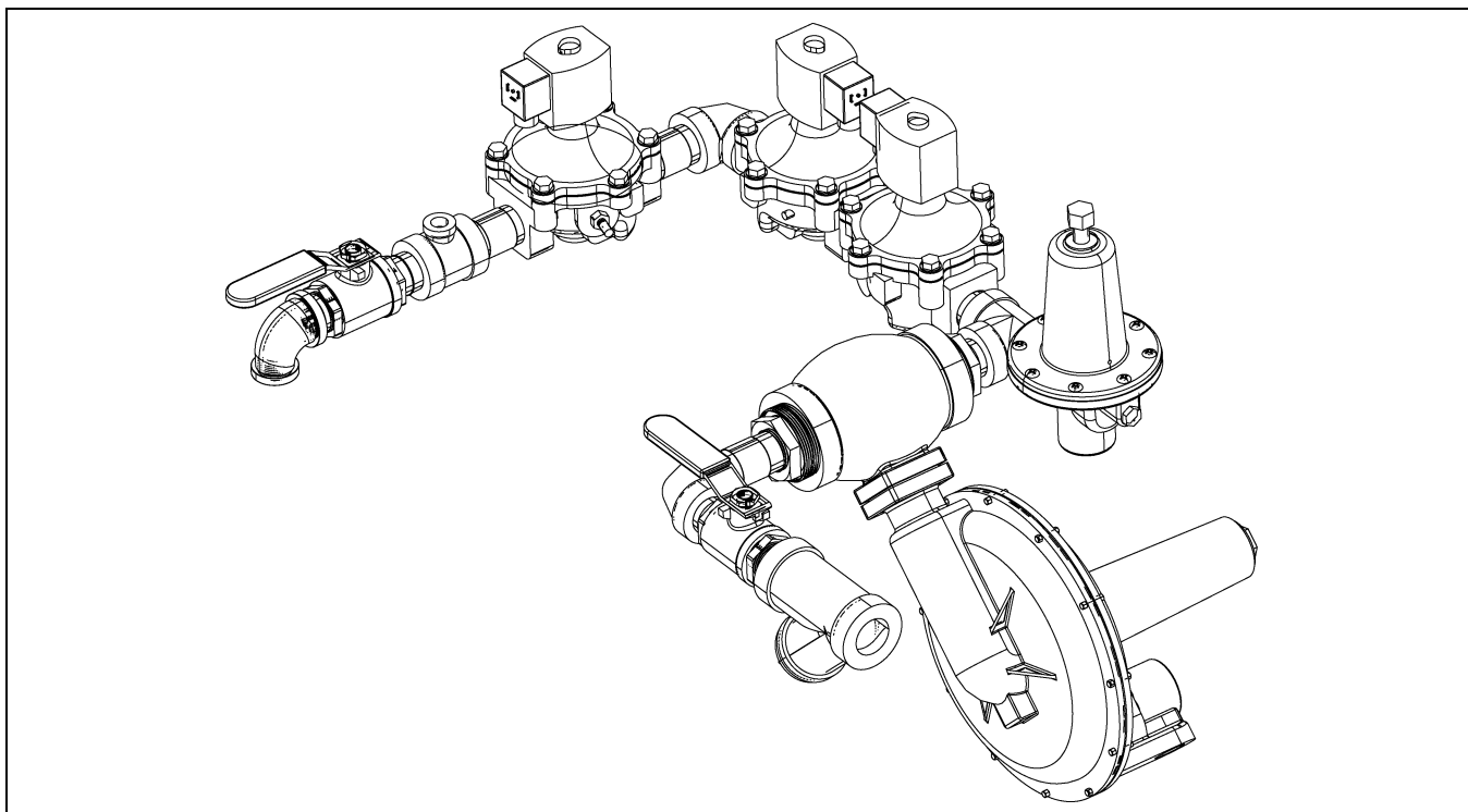
Figure 6B 36" NG Pipe Train
