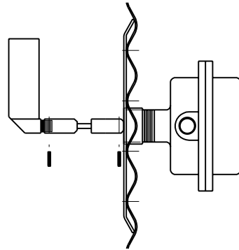
2.66" Corrugation
