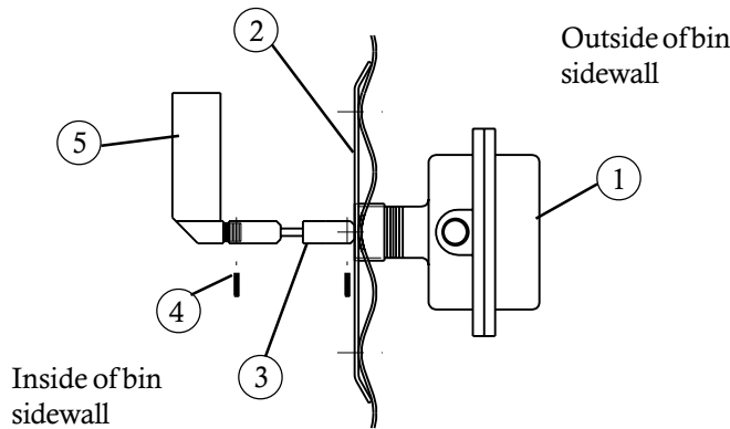
4.00" Corrugation
