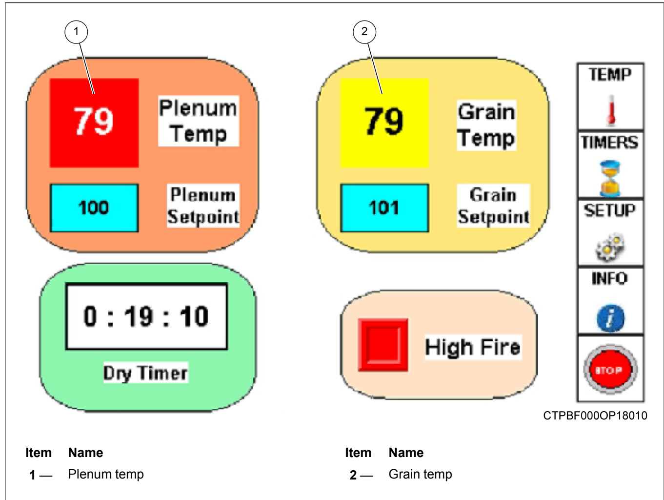
Figure 4-7 Temperature box
