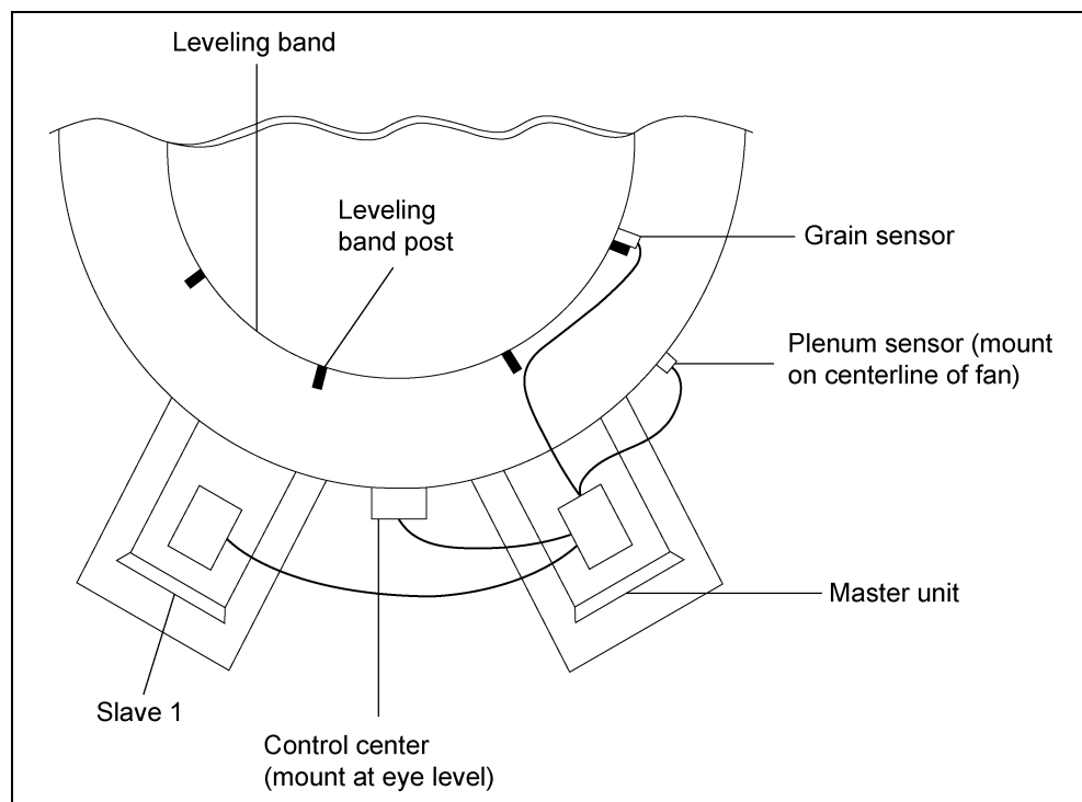
Figure 3A 2 Fan Top Dry Configuration
