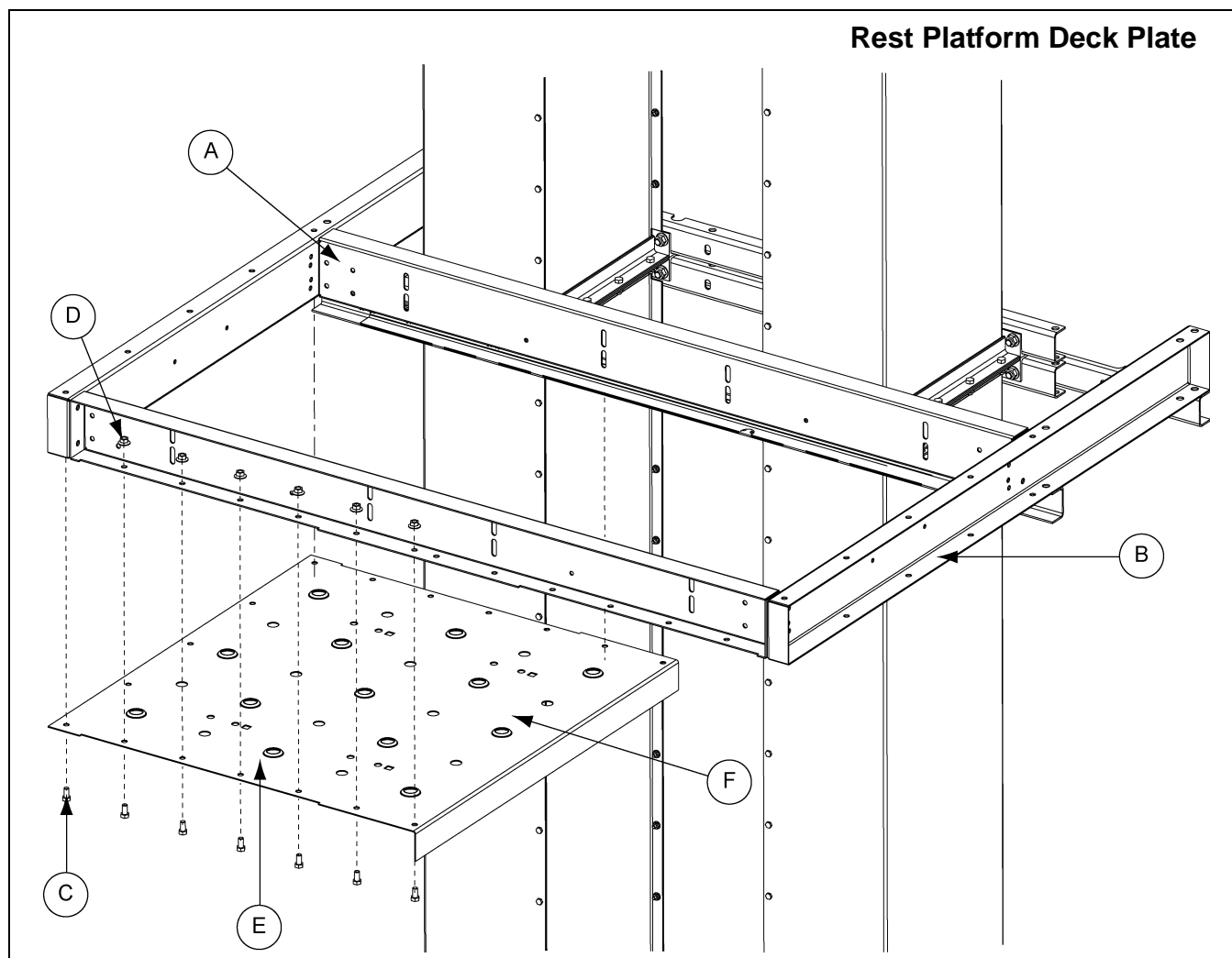
Figure 7H Deck Plate
