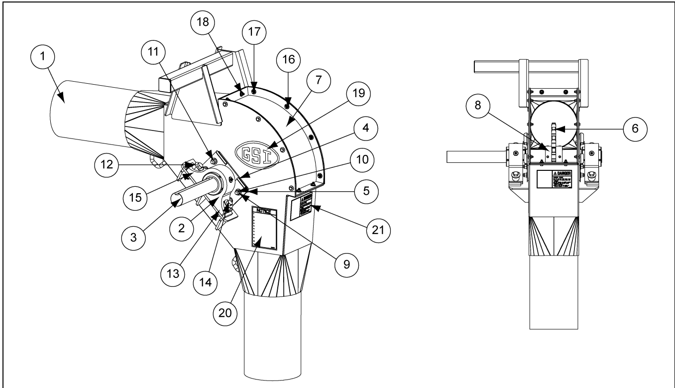
10" (40 HP-50 HP) Drive Components (8101511) Parts List
