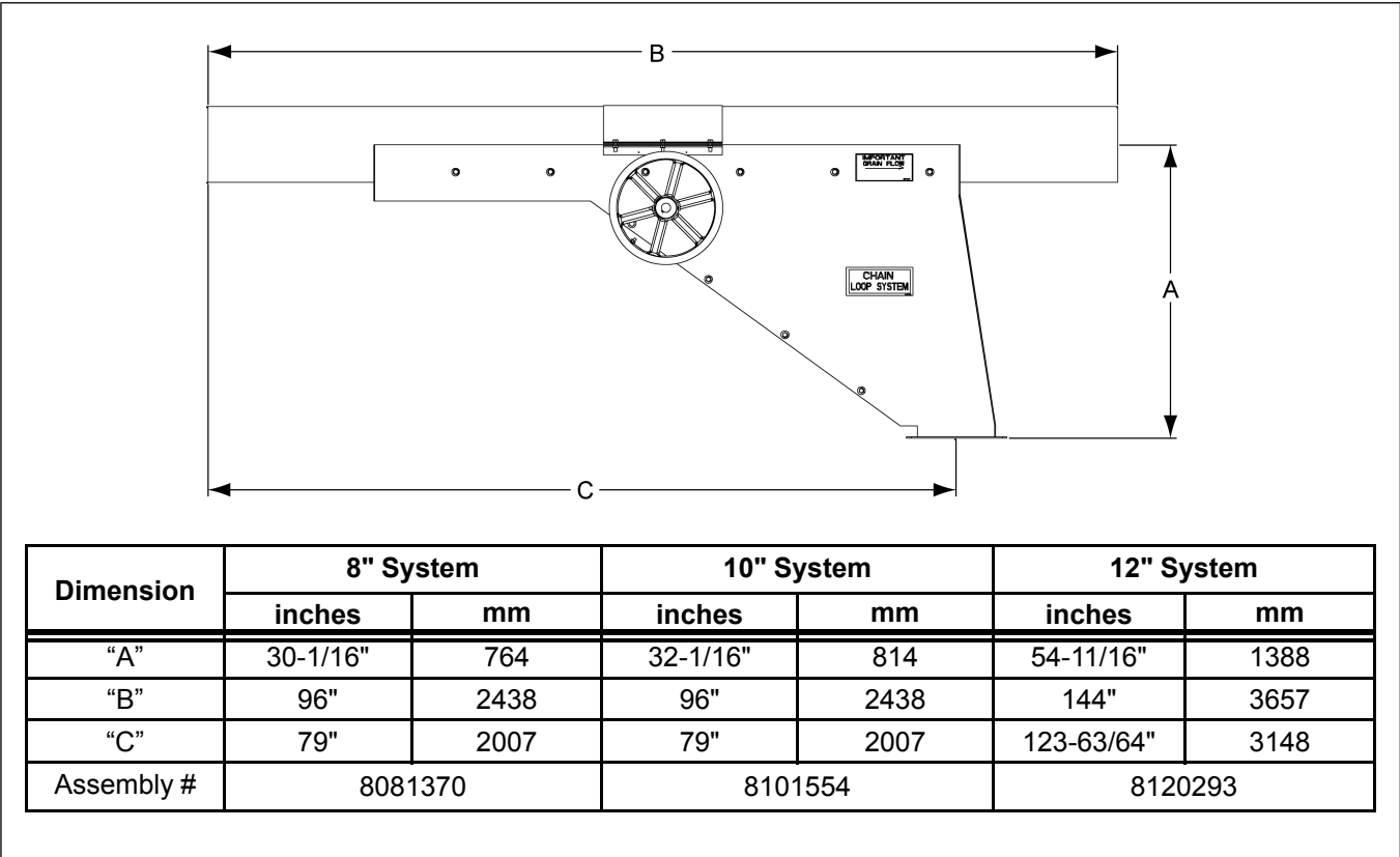
Figure 7-3 Discharge gates
