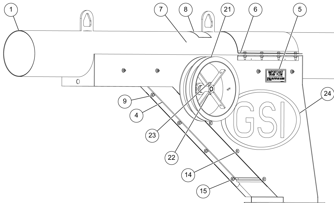
Isometric view
