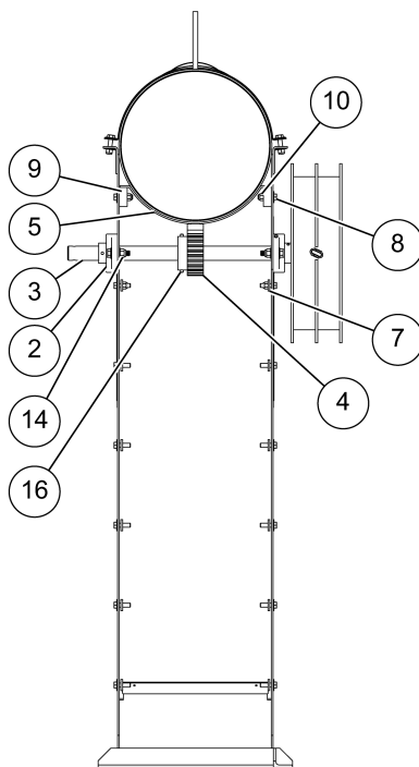
Section view
