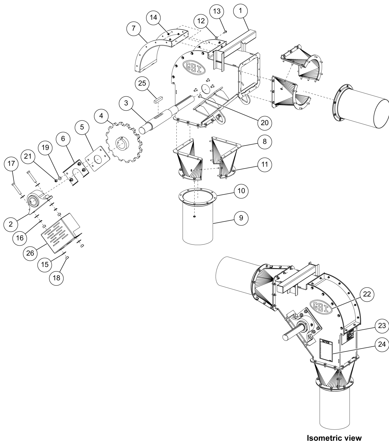
Figure 8-13 10 in. (15 HP-20 HP) HD drive components (8101633) parts
