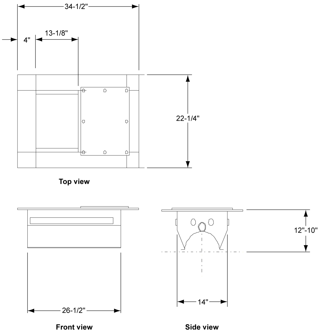
Figure 7-10 12" intermediate well
