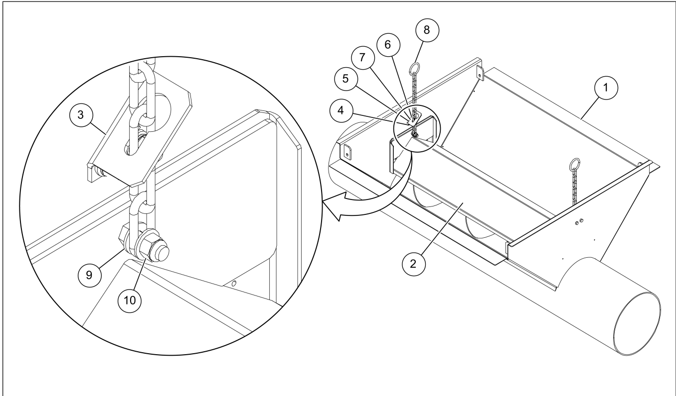
Figure 8-38 12 in. (7 Gauge) 42-1/2 in. Inlet dump hoppers (8120121) parts
