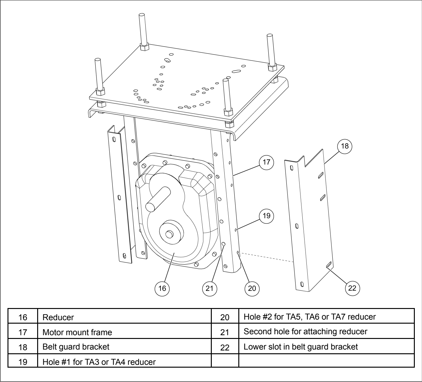
Figure 5-9 Drive box assembly
