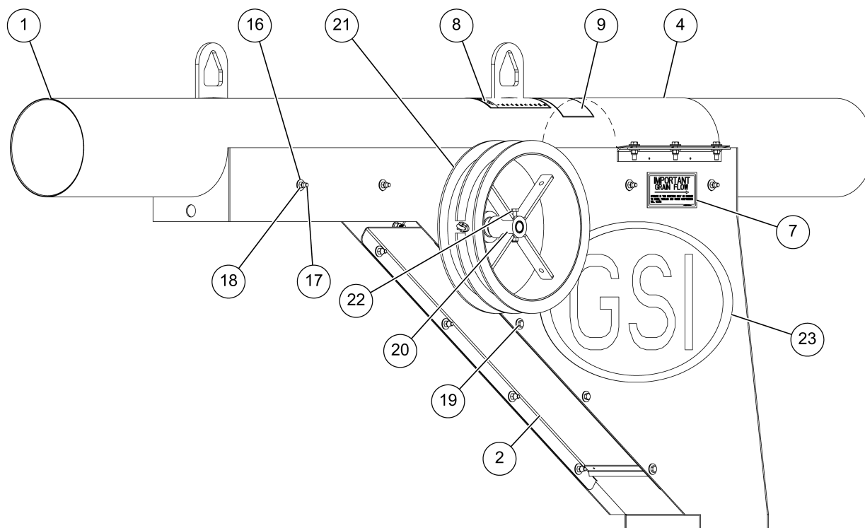
Isometric view
