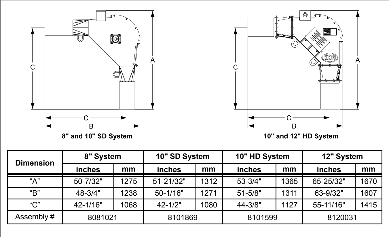
Figure 7-2 Standard corners
