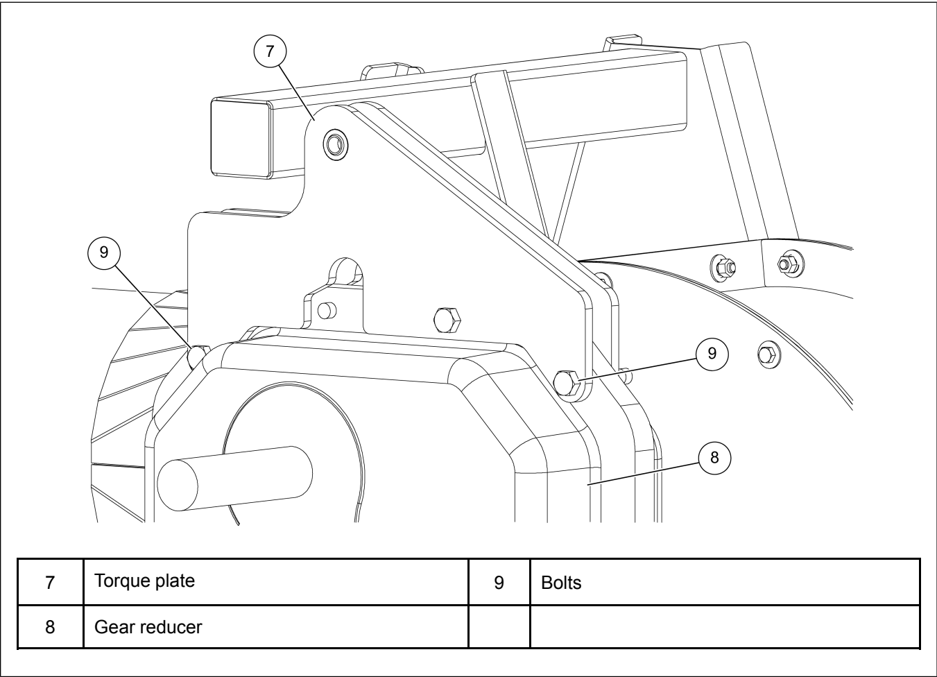
Figure 5-4 Attaching the torque plate
