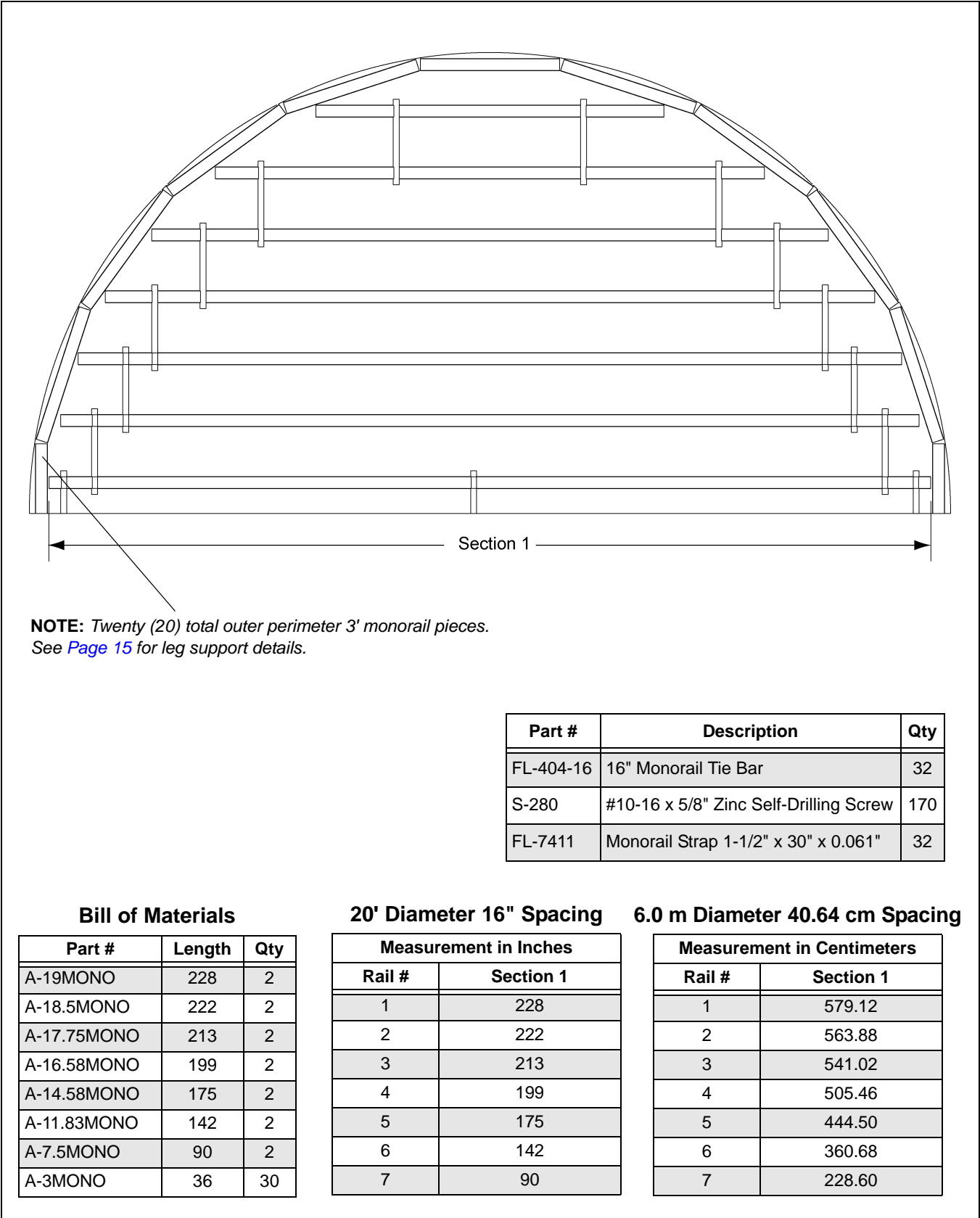
Figure 6B 20' Diameter Bin with 16" Monorail Spacing
