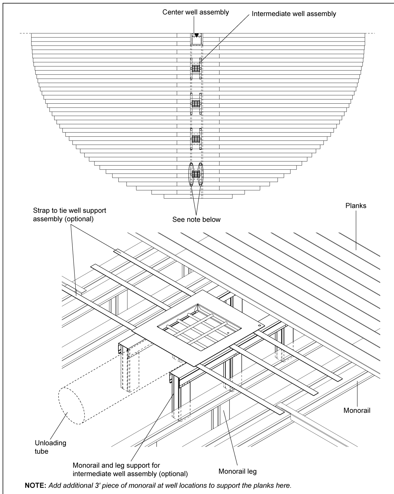
Figure 5E 20' Diameter Bin Intermediate Well Position
