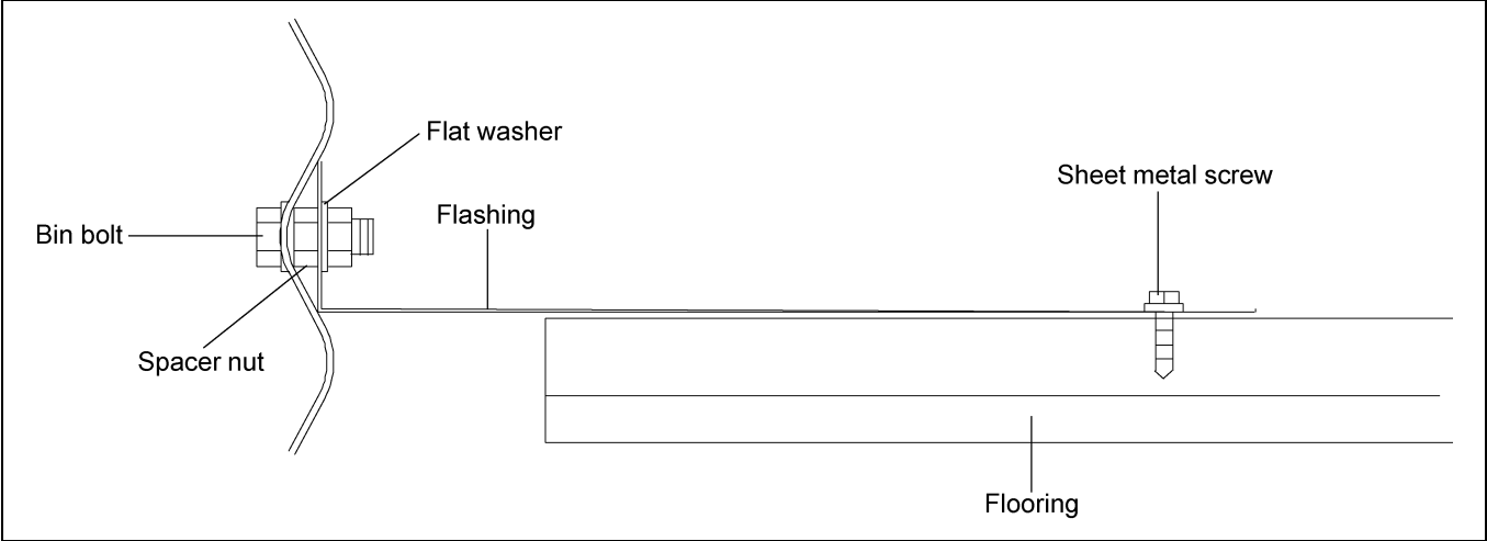
Figure 5B 2.66" Corrugation
