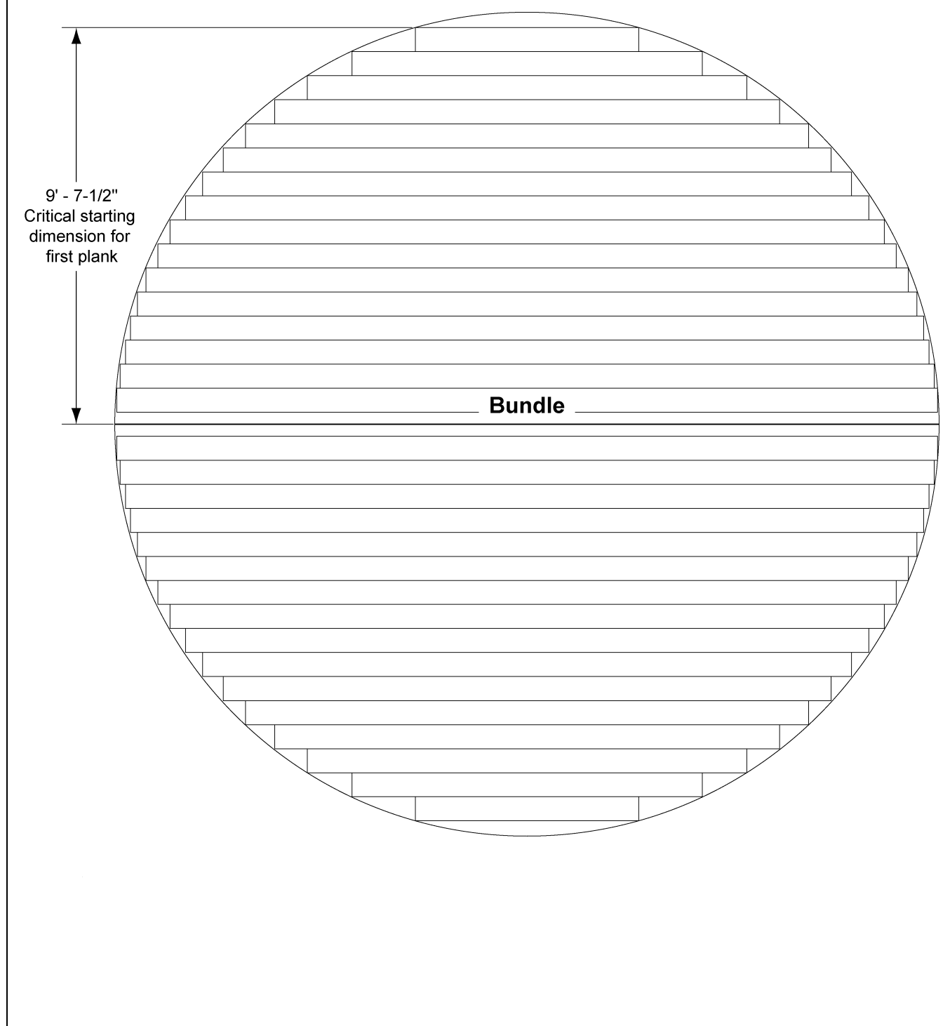
Figure 6C 20' Floor Bundle Layout
