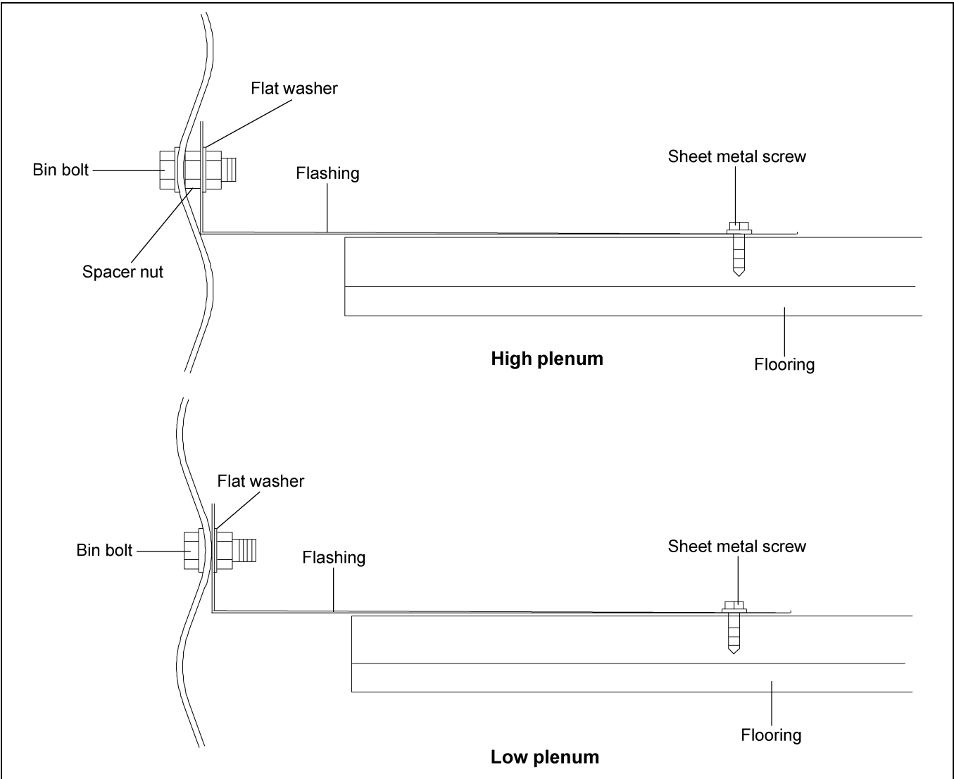
Figure 5C 4.00" Corrugation
