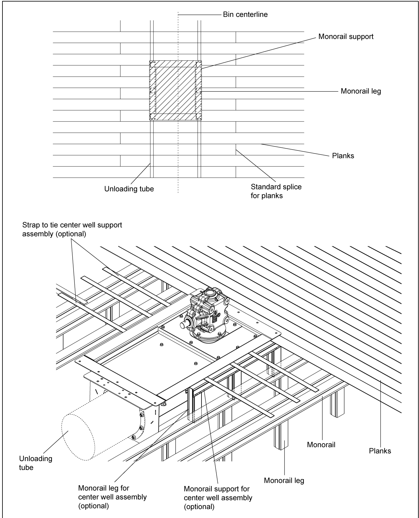
Figure 5D 20' Diameter Bin Center Well Position
