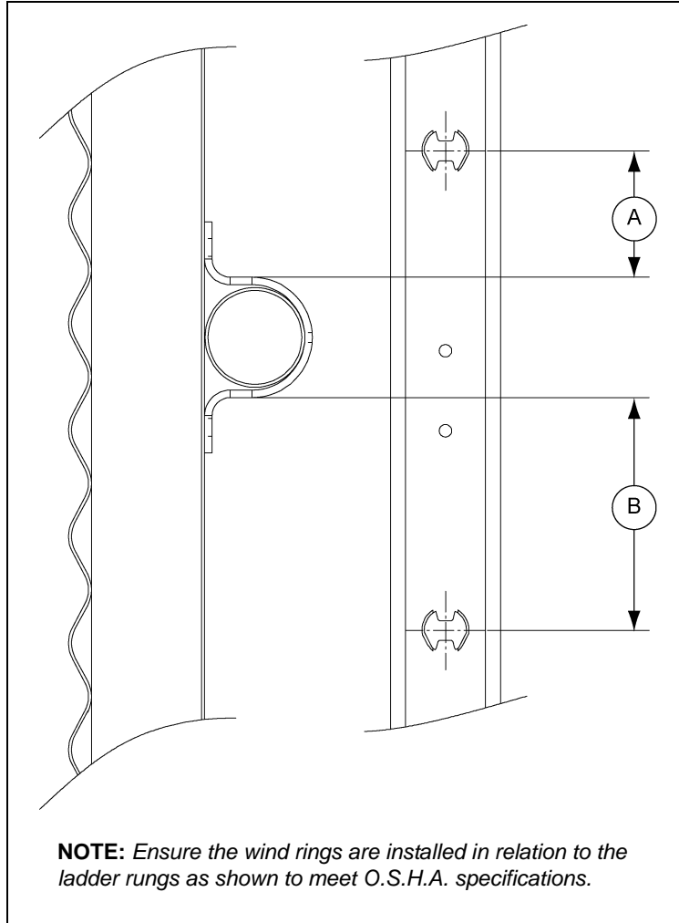
Figure 10M Dimensions for O.S.H.A. Complaint Ladder Rung Placement
