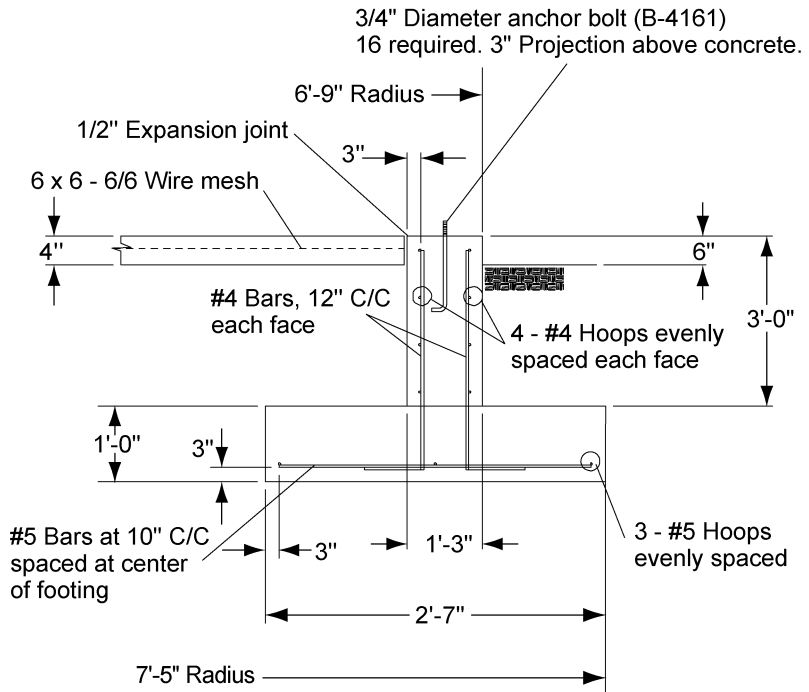
Footing detail (NOTE: Not to scale)
