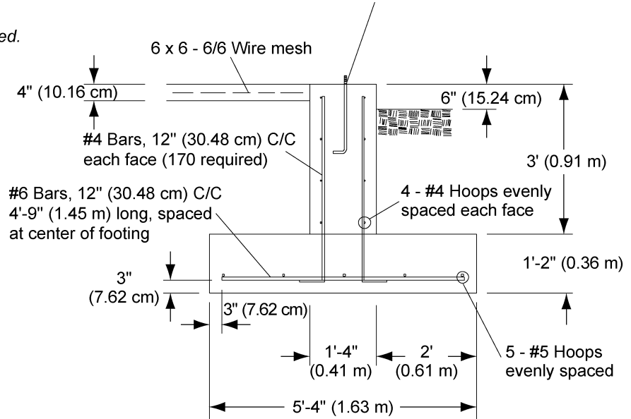
Footing detail (NOTE: Not to scale)
