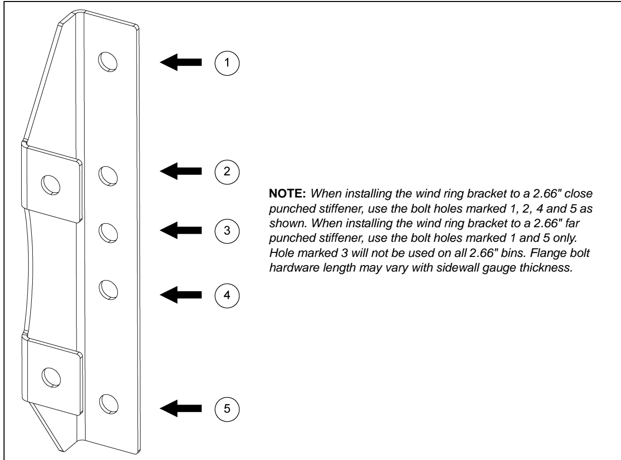
Figure 10N Wind Ring Bracket
