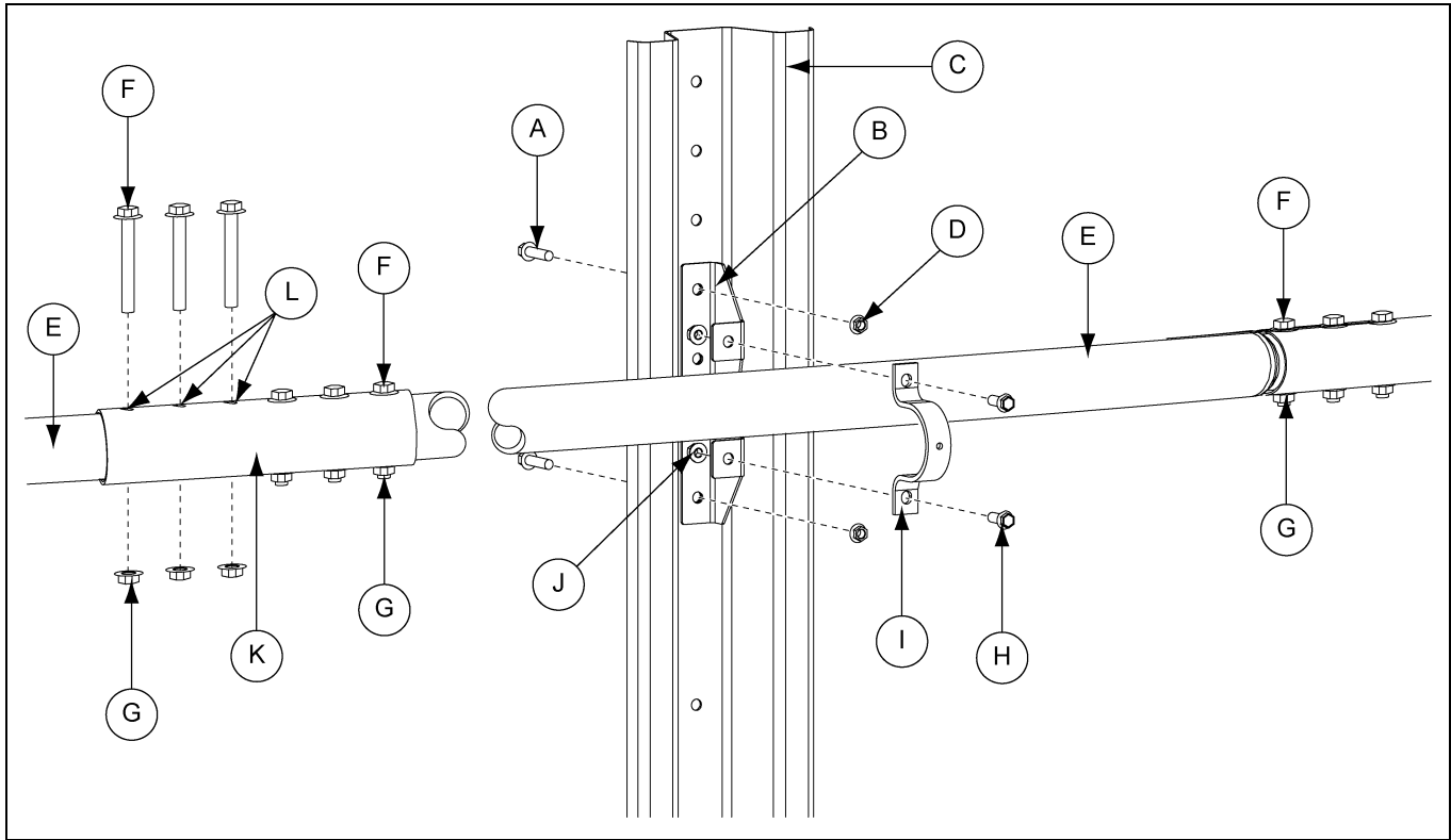
Figure 100 Exploded View of Wind Ring Installed at Upper Portion of Stiffener
