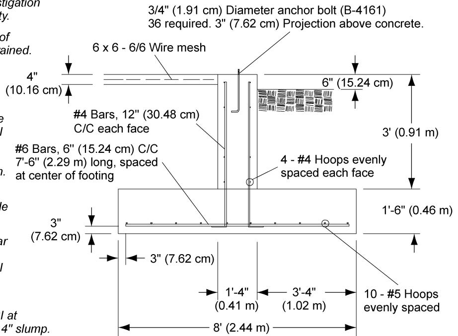
Footing detail (NOTE: Not to scale)
