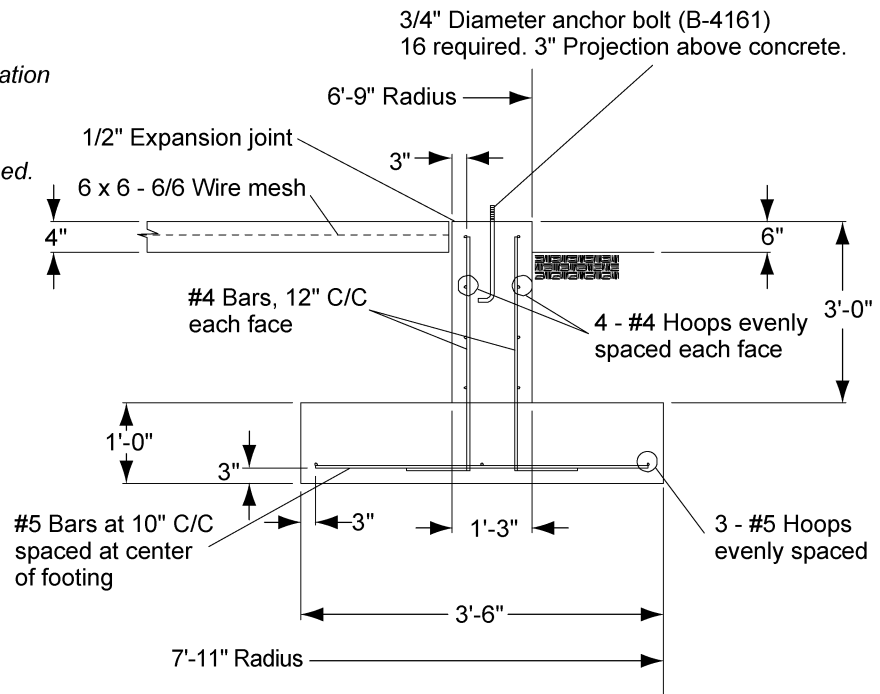
Footing detail
