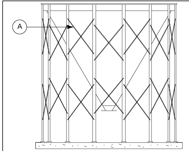
Figure 5M Completed Hopper Assembly
