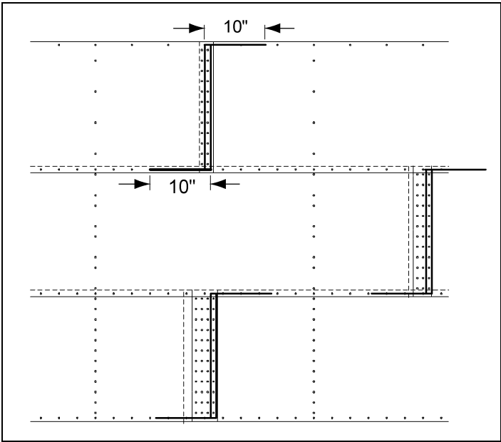
Figure 9B Standard, Triple and Quad Punched Sidewall Sheets as Viewed from Outside
