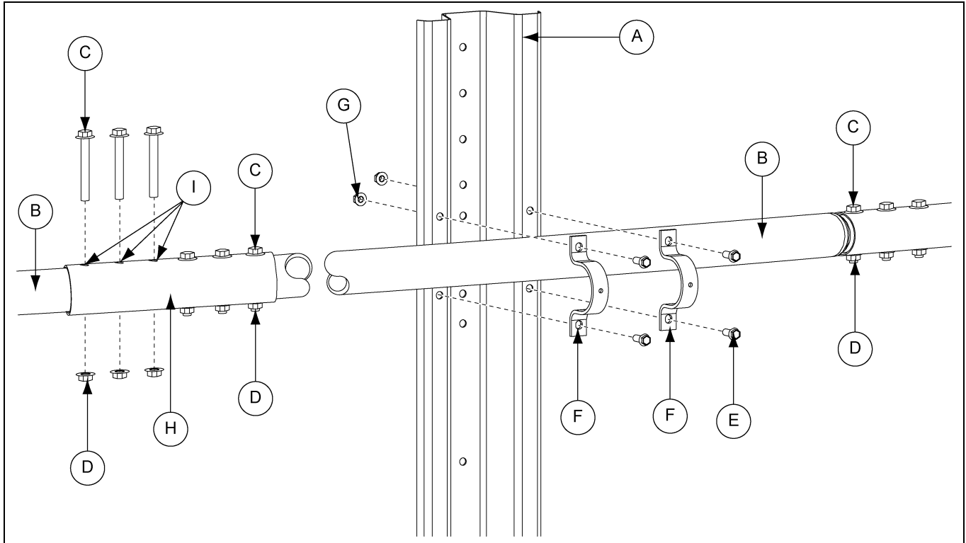
Figure 10N Exploded View of Wind Ring Installed at Upper Portion of Stiffener
