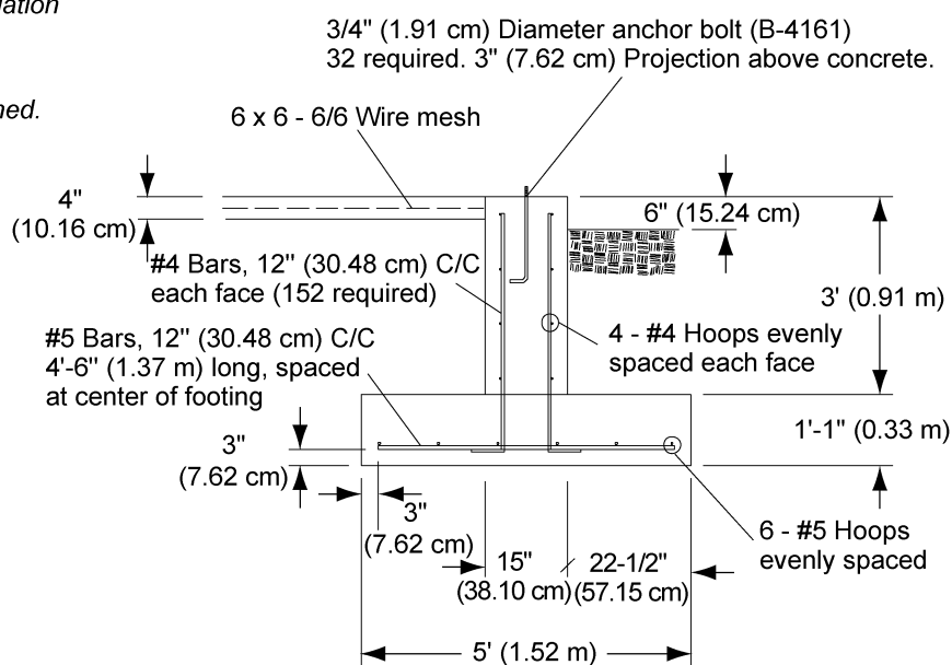
Footing detail
