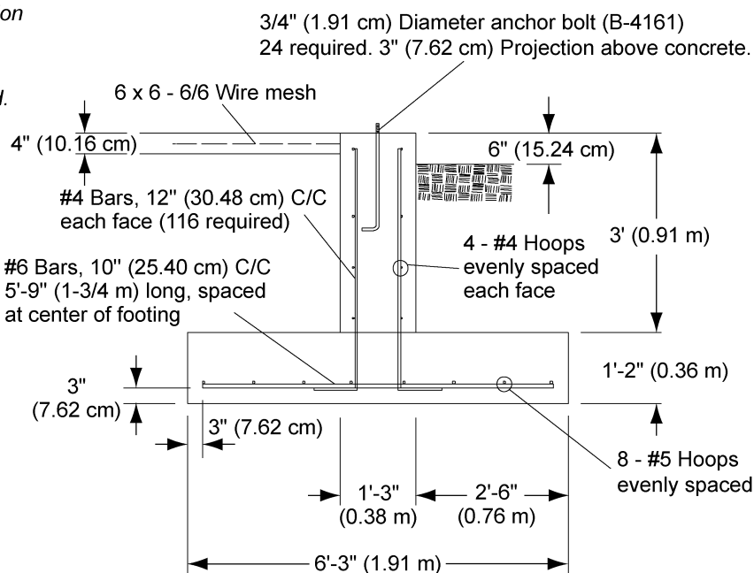
Footing detail
