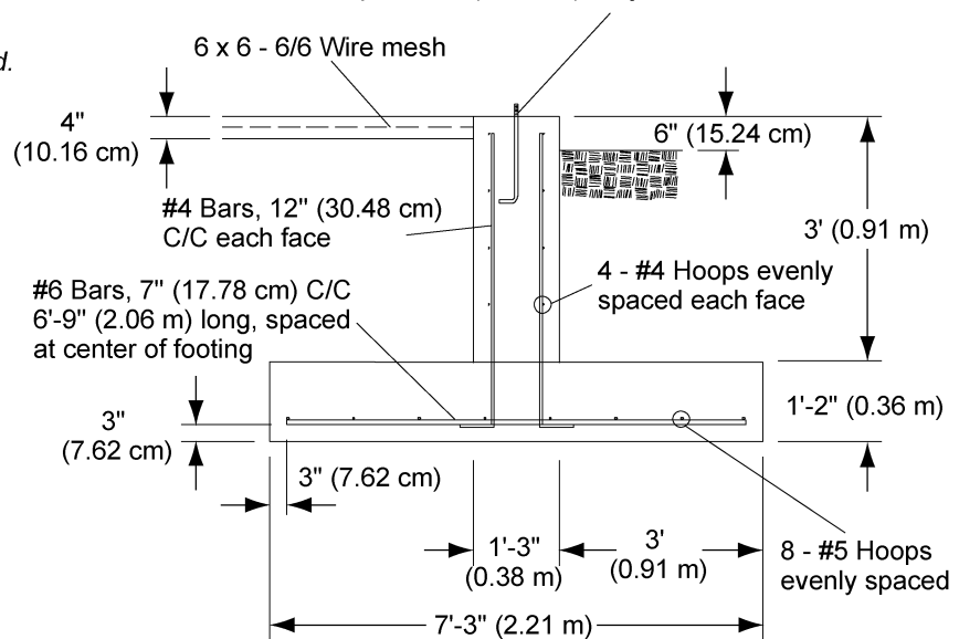
Footing detail
