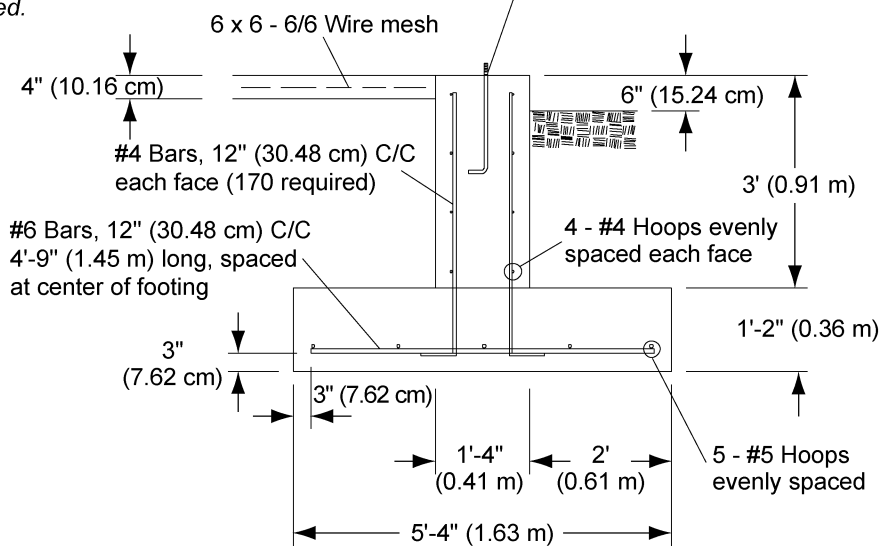
Footing detail
