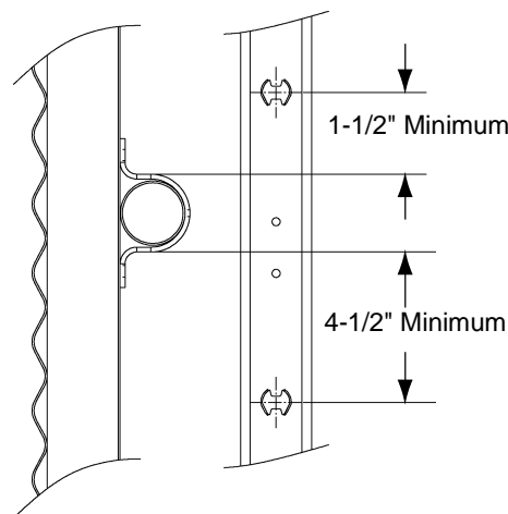
Figure 10M Dimensions for O.S.H.A. Compliant Ladder Rung Placement
