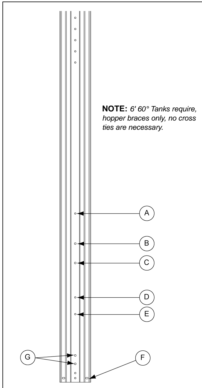
Figure 13H 6' Leg 60°
