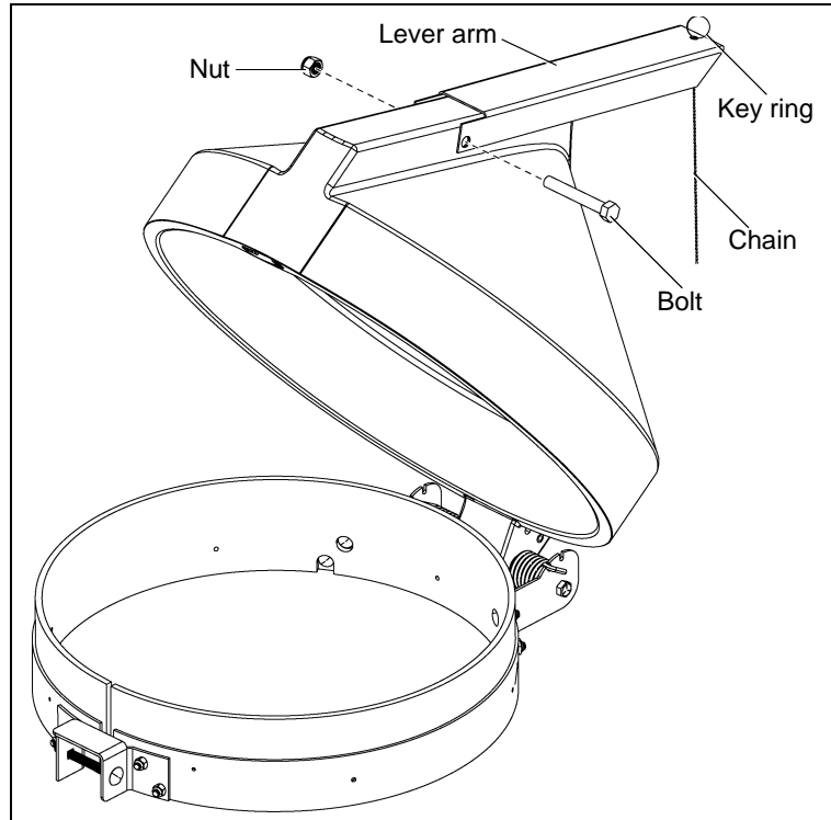
Figure 6 Installing the Lever Arm and Chain
