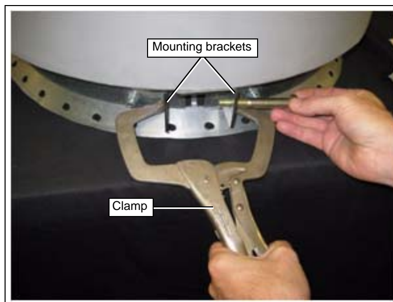
Figure 7 Mounting the Lid to Peak Ring
