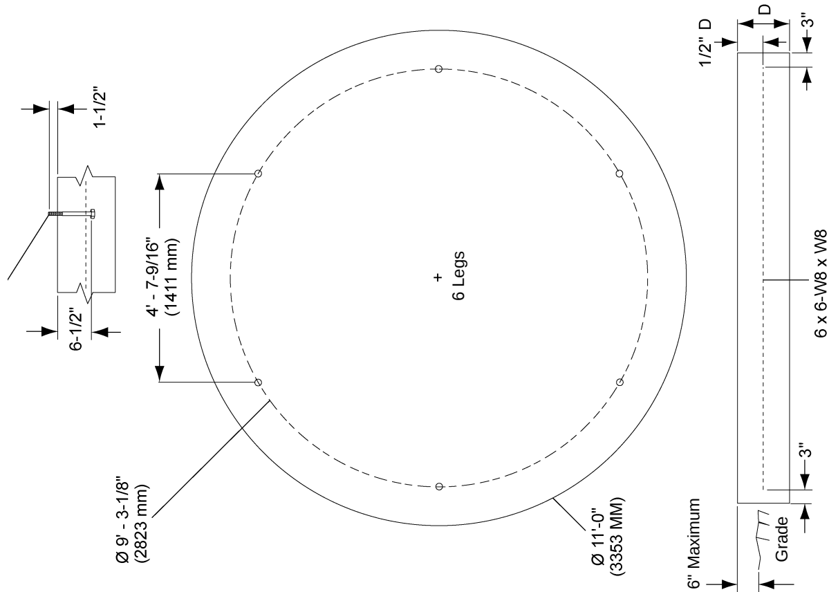
Figure 5F 9' 2-9 Rings BFT/ GHT 45° and 60° Round Pad
