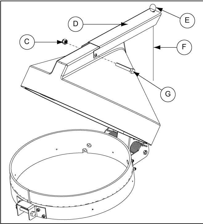
Figure 11B Install Lever Arm and Chain
