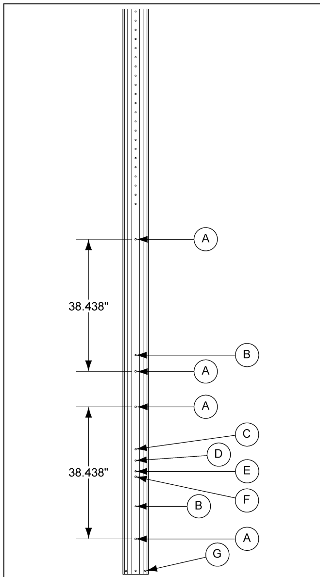
Figure 13E 7' Leg 67° - 7-8 Rings and 9' Leg 60° - 7-11 Rings (BLK-12504)
