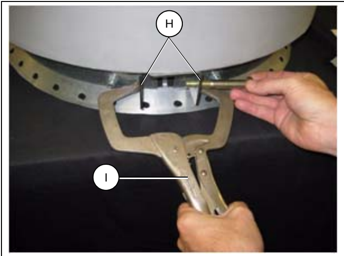
Figure 11C Mount Lid to Peak Ring
