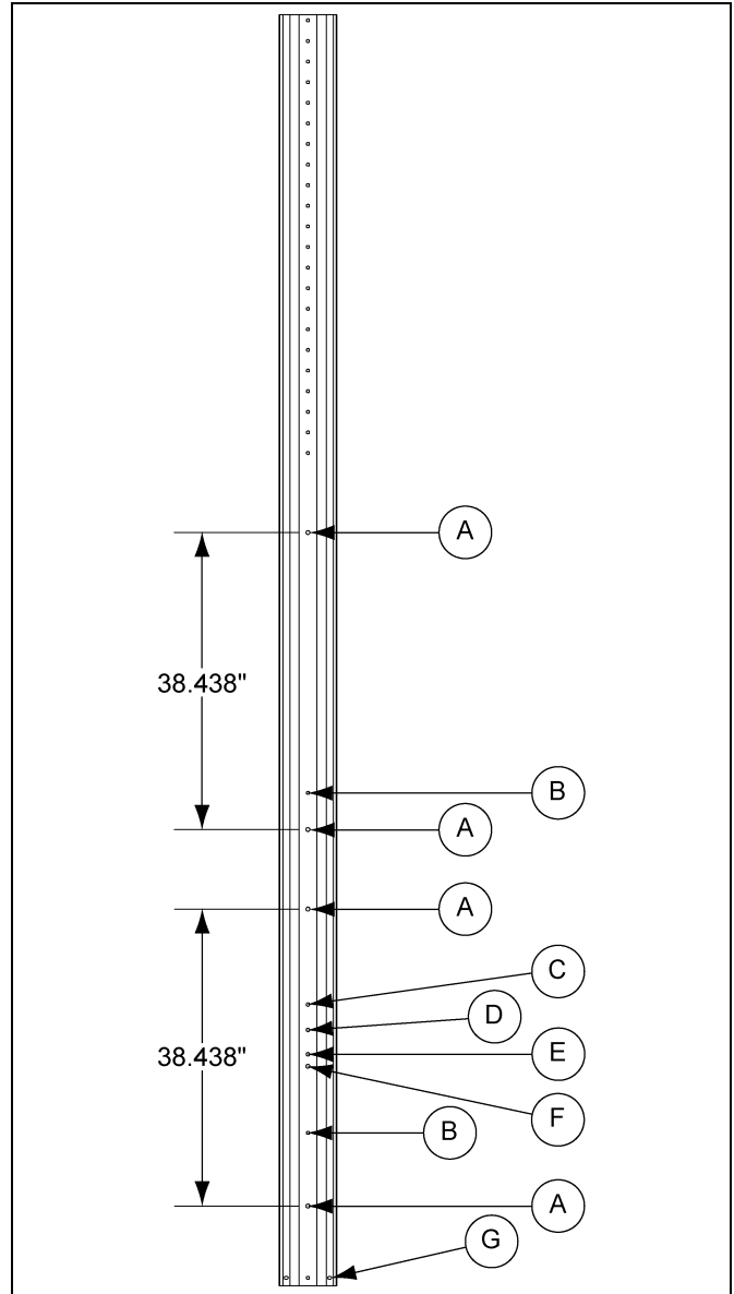
Figure 12E 7' Leg 67° - 7-8 Rings and 9' Leg 60° - 7-11 Rings (BLK-12504)
