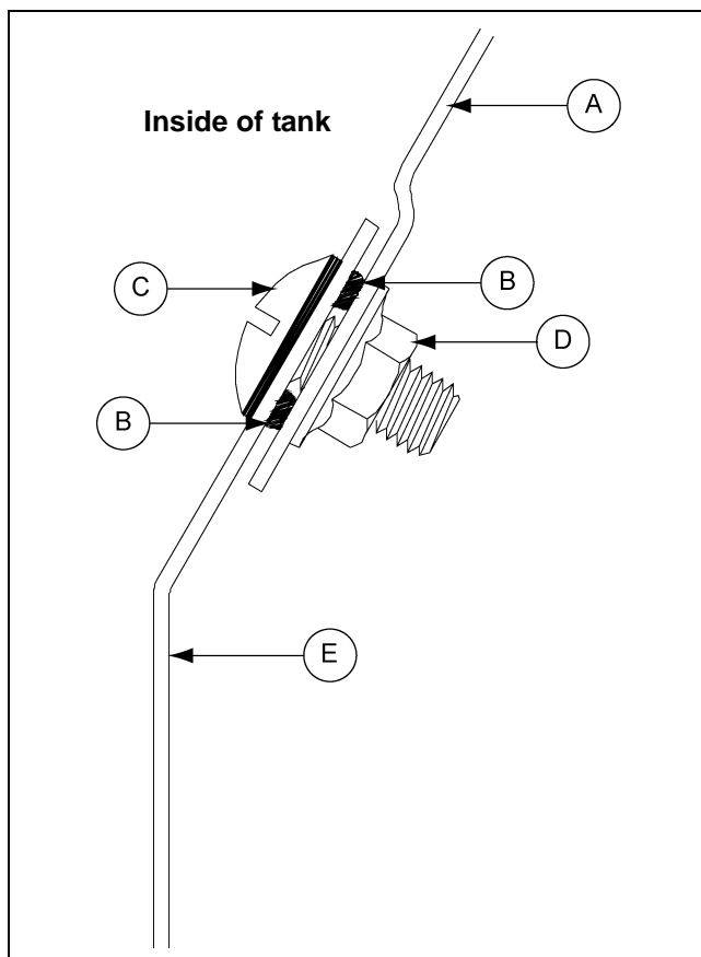
Figure 11H Bolt Detail Hopper Collar
