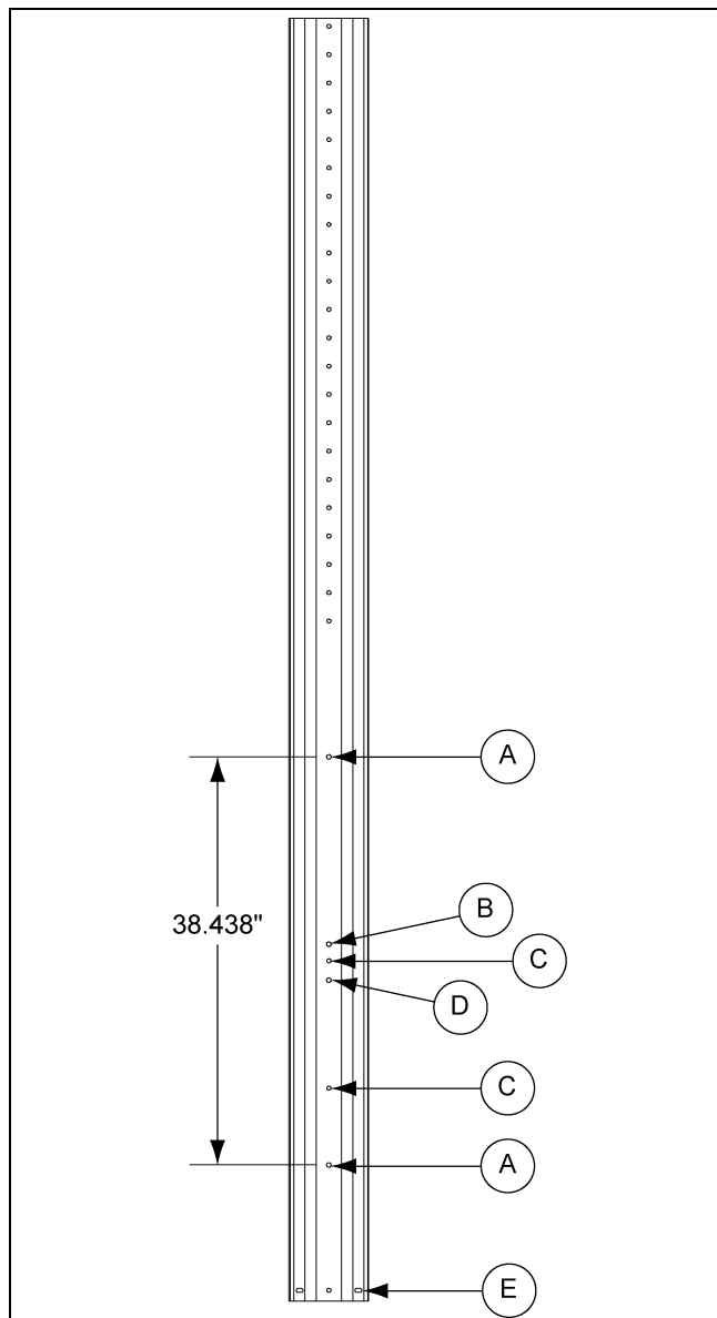
Figure 12C 7' Leg 45° - 7-8 Rings (BLK-12538)
