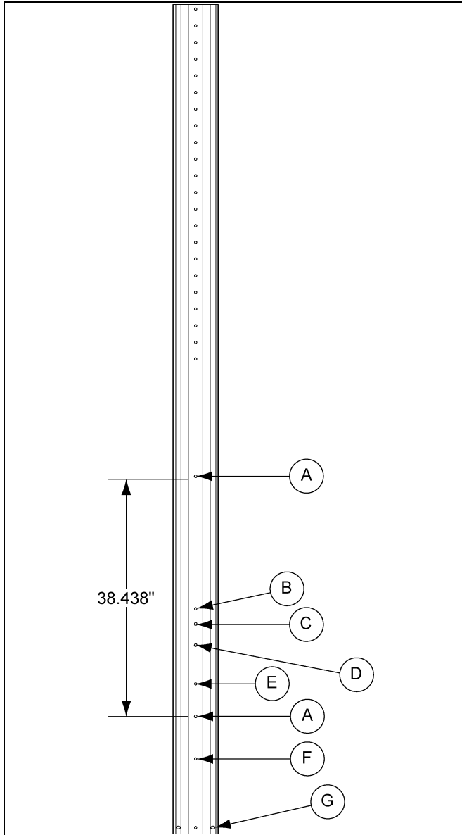
Figure 12D 9' Leg 45° - 7-11 Rings (BLK-12505)
