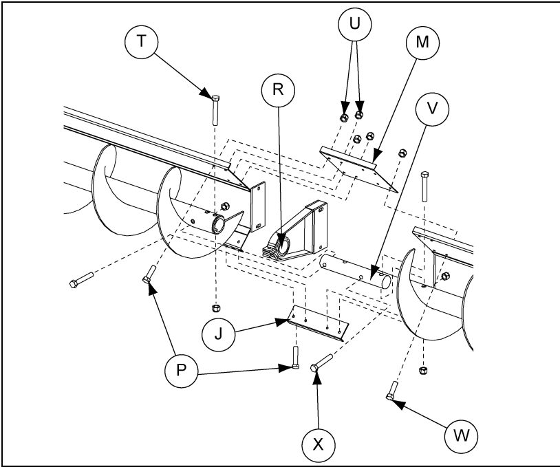
Figure 4K Splice Plate Angled View
