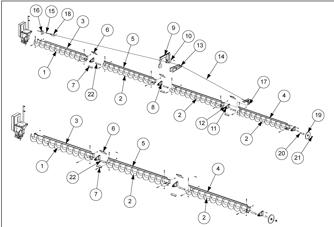
12" Flight and Shield Parts List
