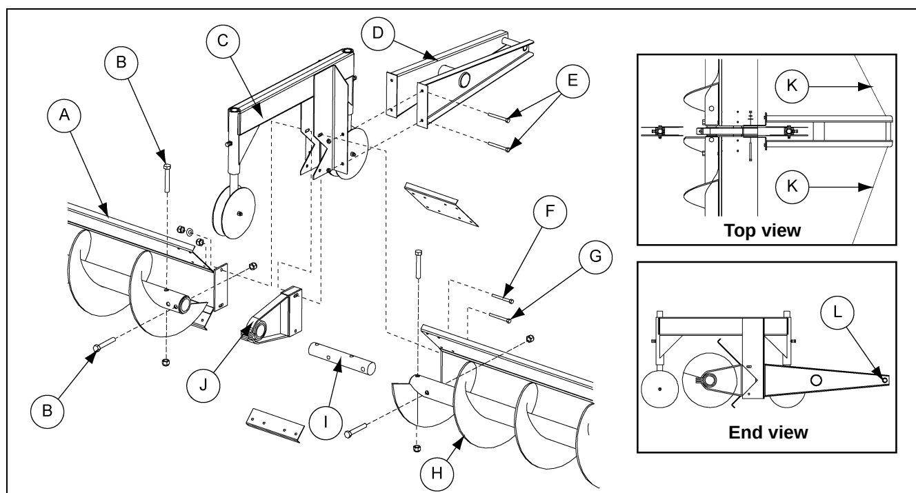
Figure 4M Sweep Carrier Wheel and Truss Stand Detail
