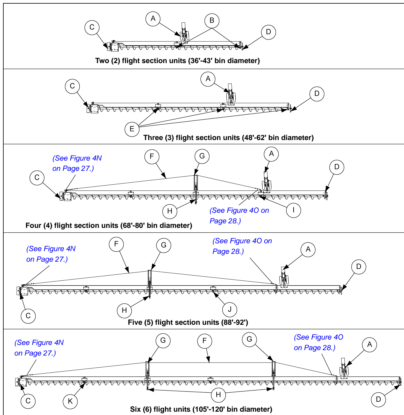
Figure 4F Sweep Flight Back Shield Layouts
