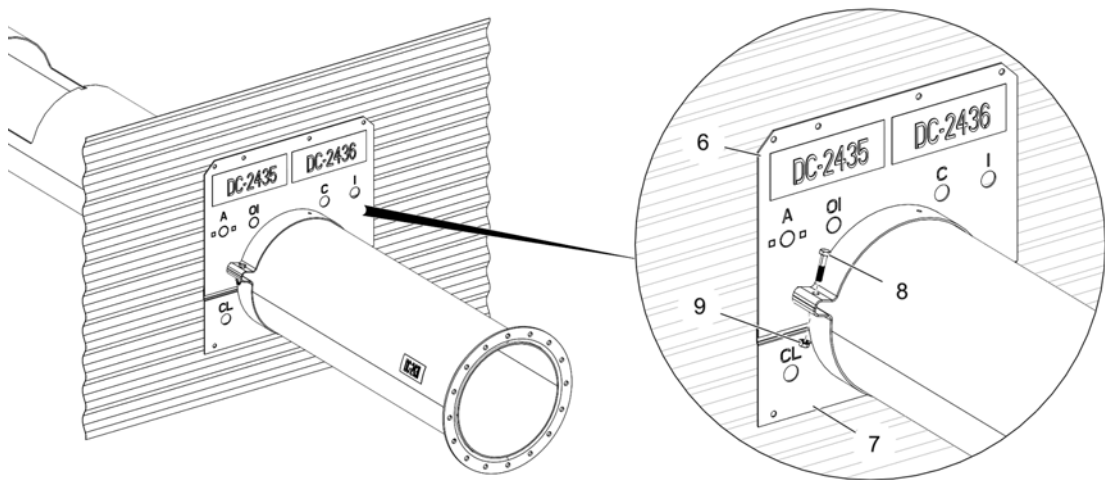
Figure 3-7 Installing the upper and lower bin flanges
