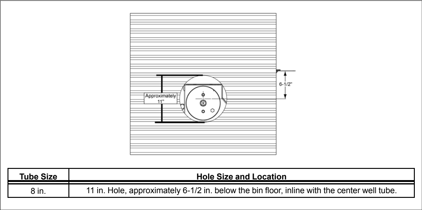
Figure 3-2 8 in. Tube
