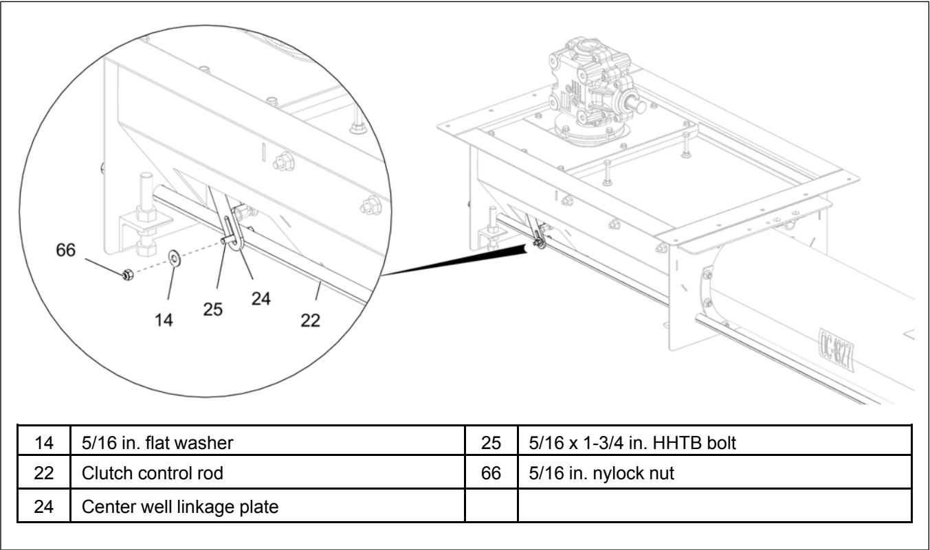
Figure 3-23 Installing the clutch control rod to center well linkage
