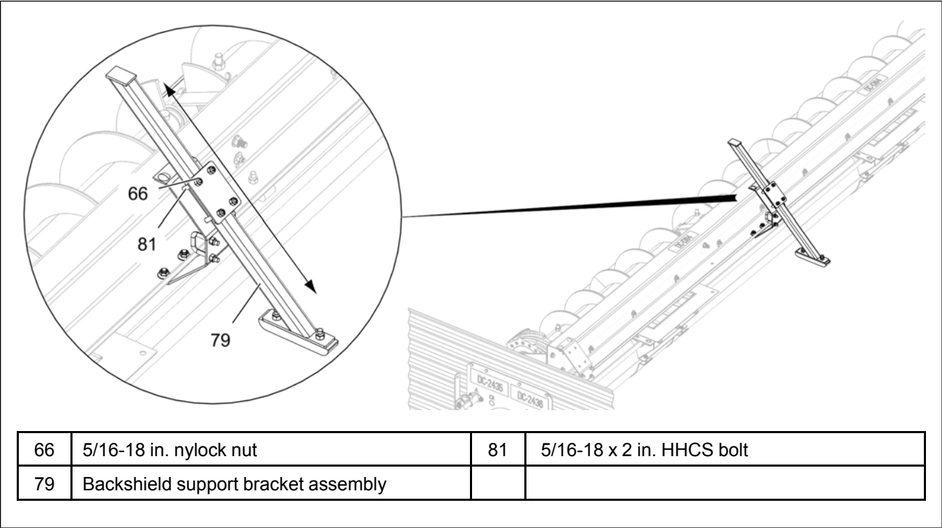
Figure 3-45 Adjusting the backshield assembly
