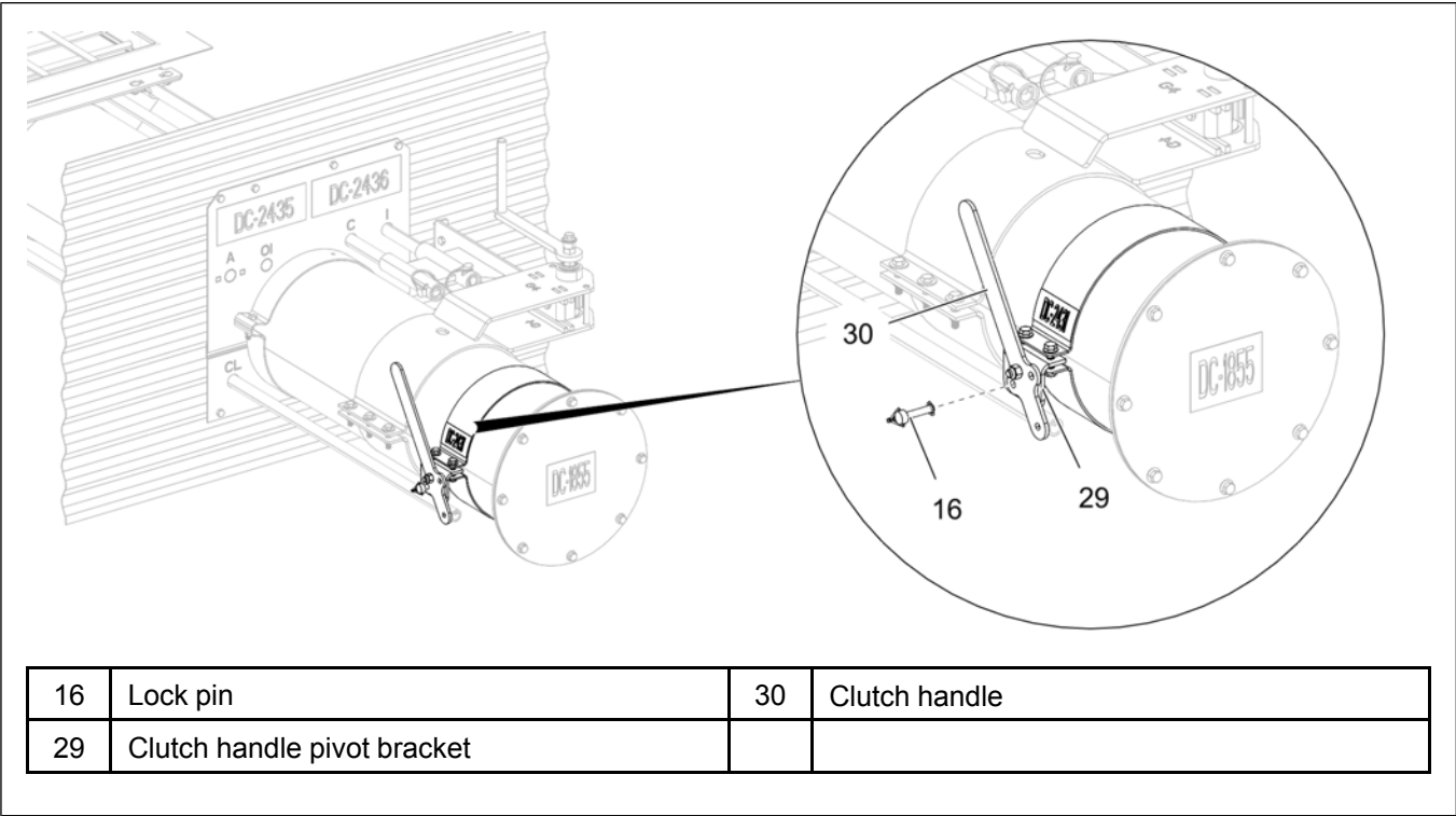
Figure 3-27 Inserting the lock pin
