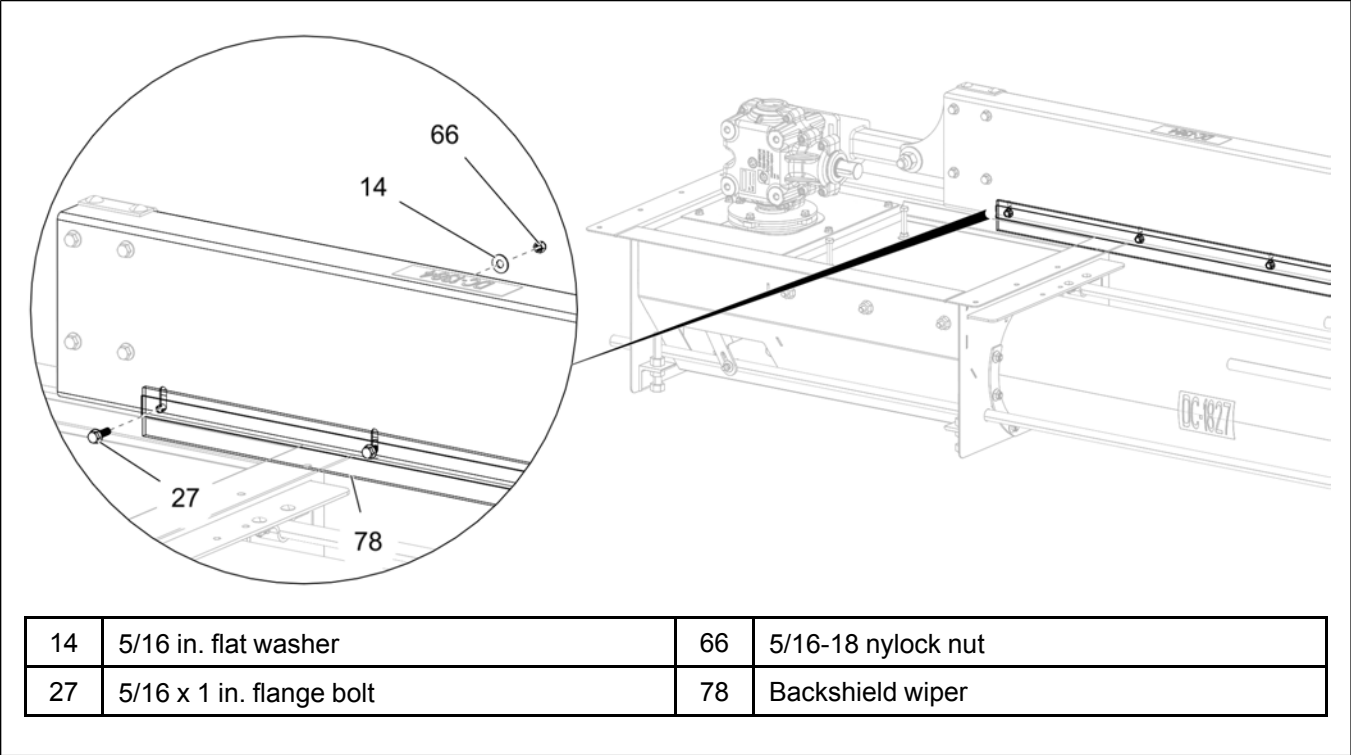
Figure 3-43 Wiper in DOWN position
