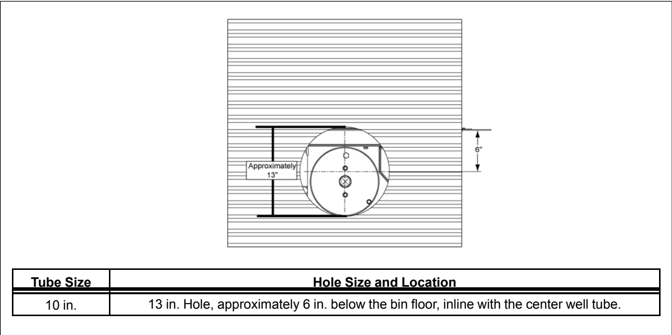
Figure 3-3 10 in. Tube
