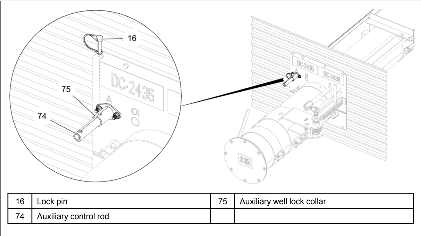
Figure 3-17 Installing the lock pin
