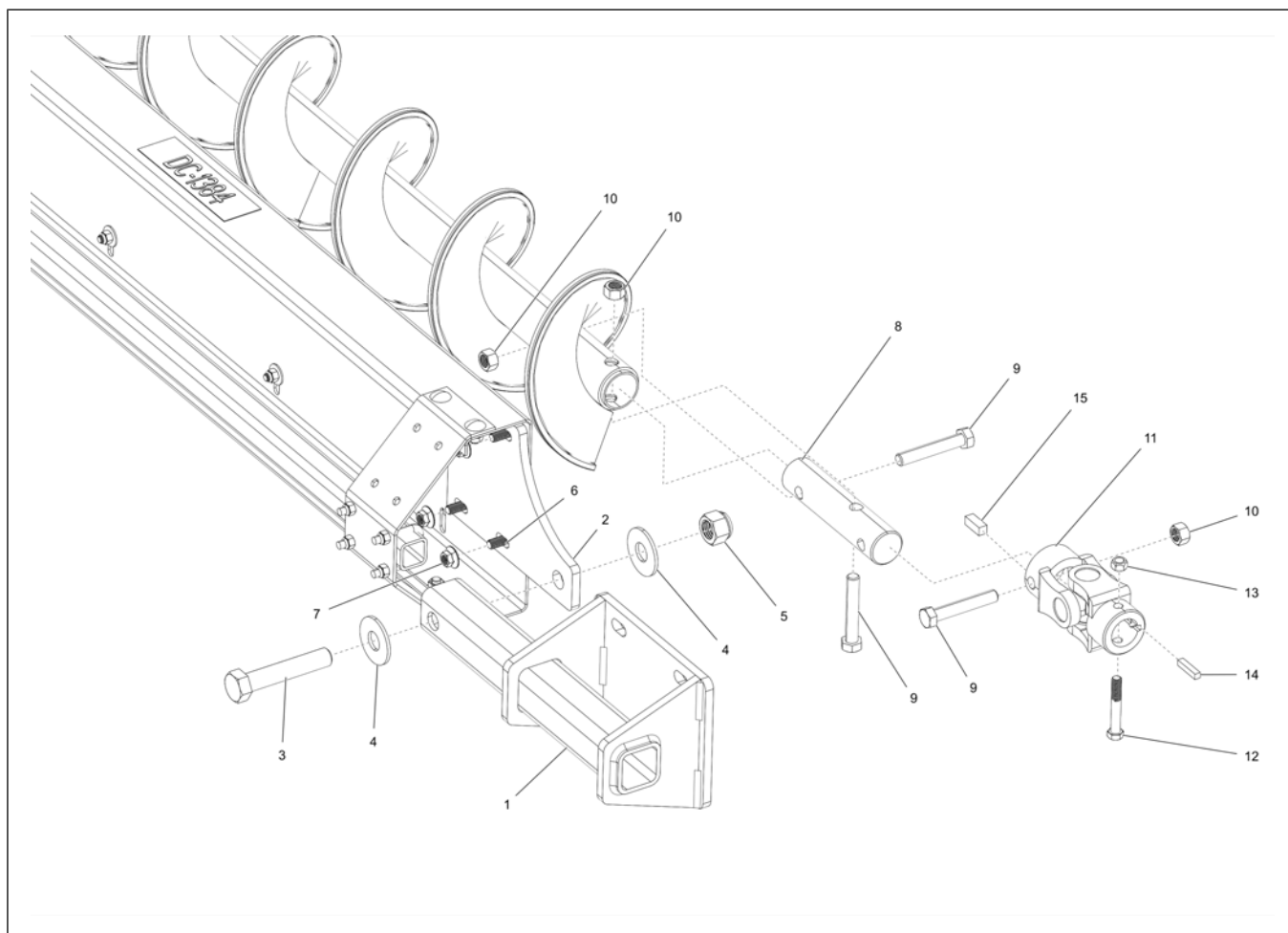
Figure 7-20 Backshield connections – Exploded view
