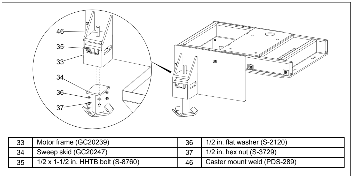
Figure 2-7 Installing the skids and caster mount to the motor frame
