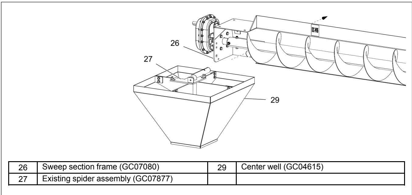
Figure 2-3 Separating the center well
