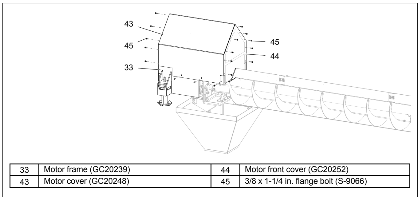
Figure 2-11 Installing the motor cover and end panels to the motor frame
