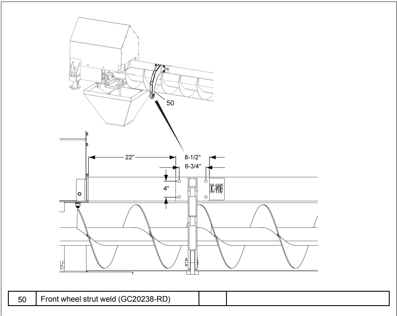
Figure 2-13 Field drill holes for front wheel strut
