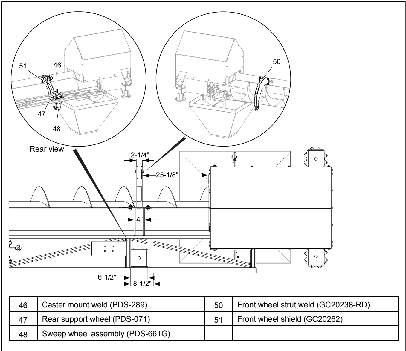
Figure 2-12 Position of wheel assembly, rear support and front wheel strut
