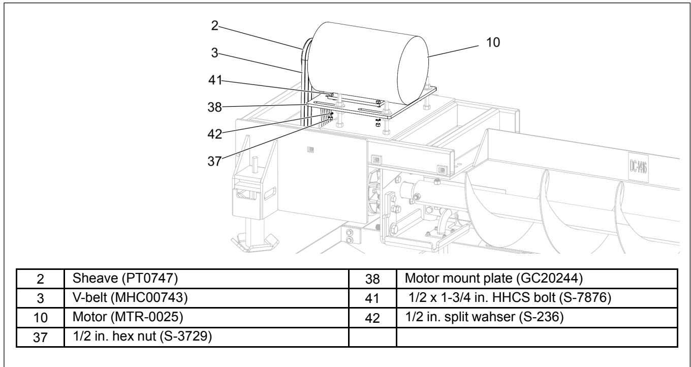
Figure 2-10 Installing the pulley, belts and motor to the motor frame
