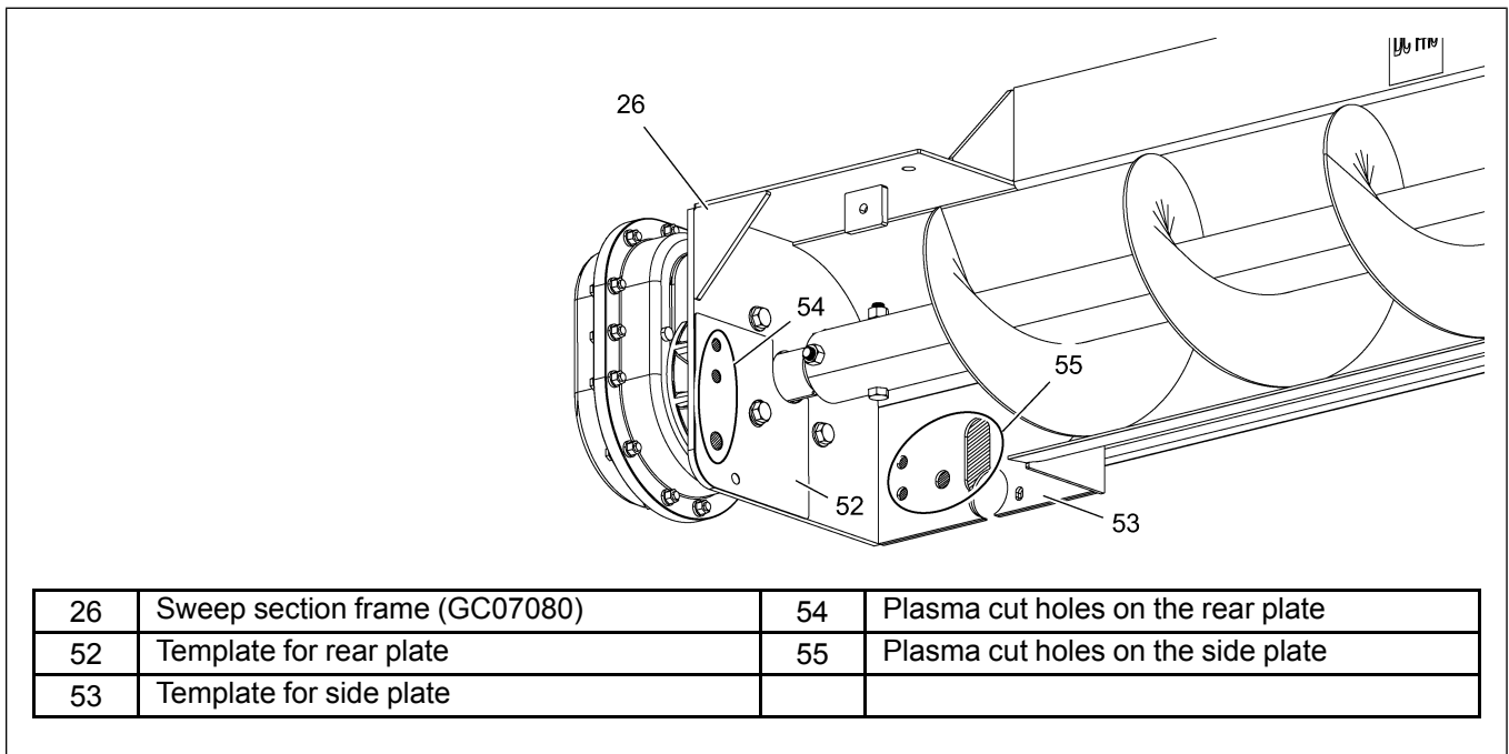
Figure 2-5 Plasma cutting holes and slot
