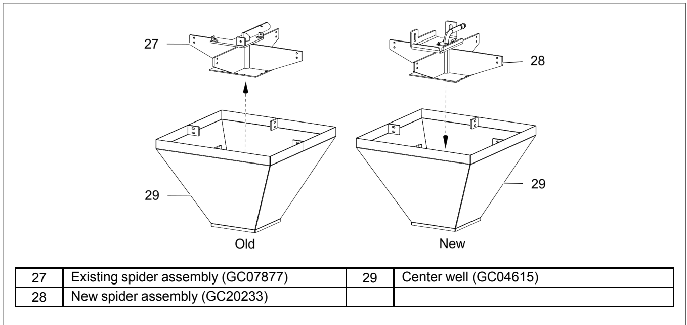
Figure 2-4 Replacing the spider assembly
