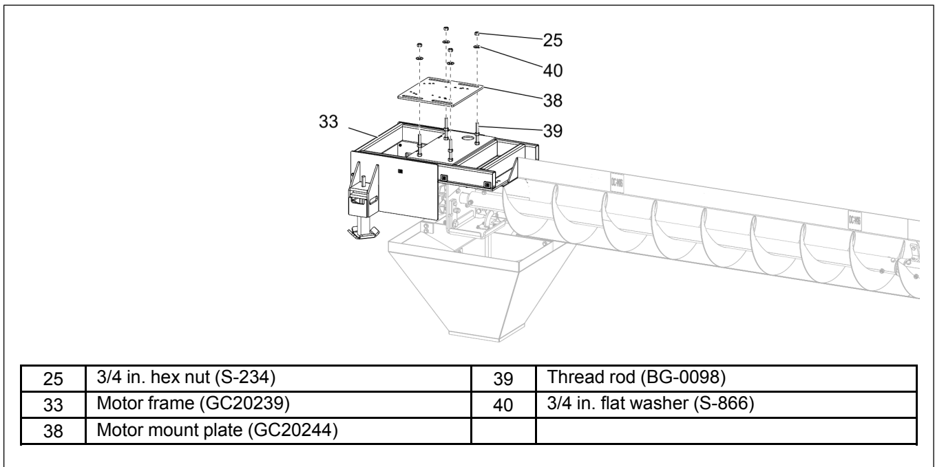
Figure 2-9 Installing the motor mount plate to the motor frame
