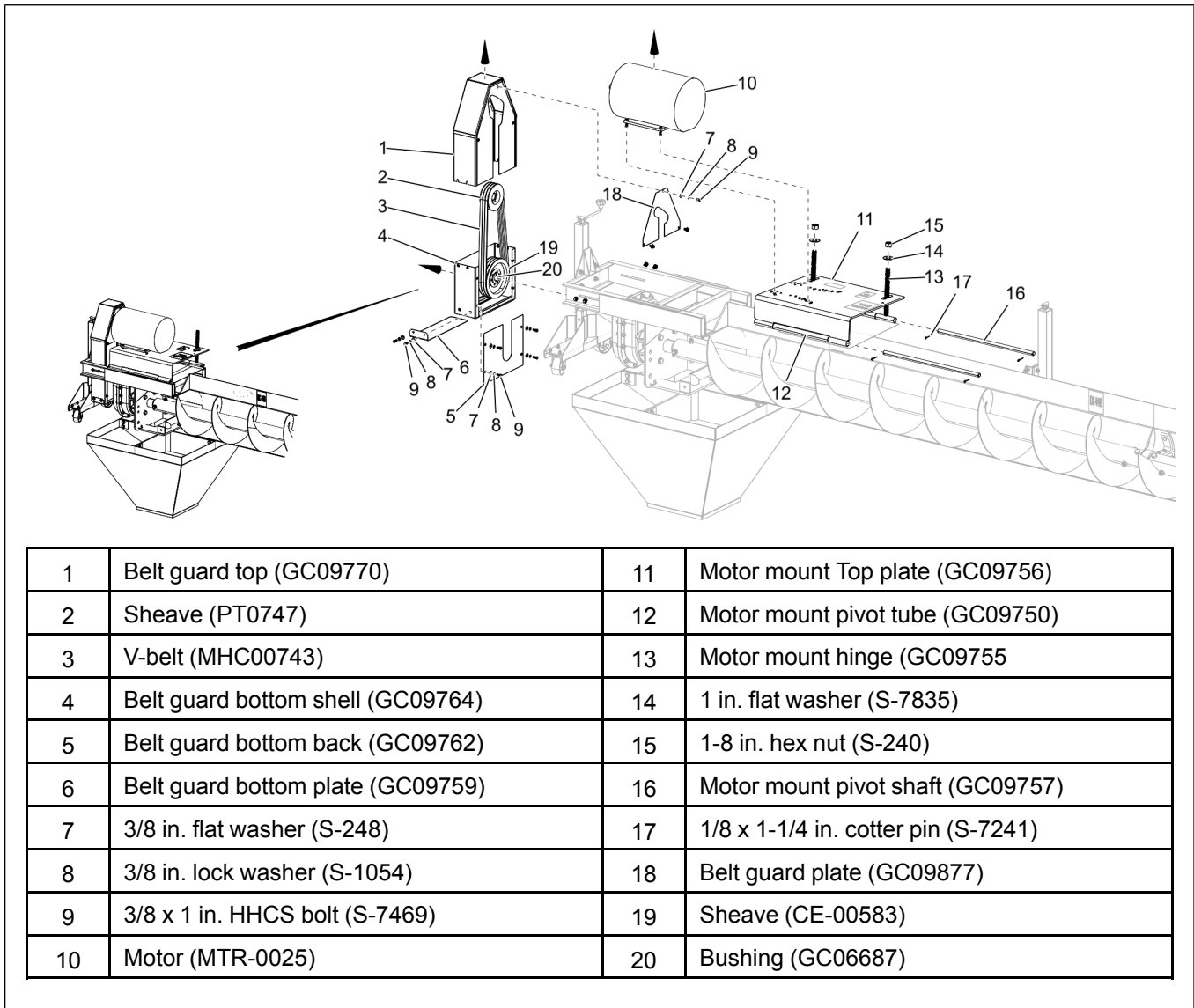
Figure 2-1 Removing the belt guards, belts, motor and pulley
