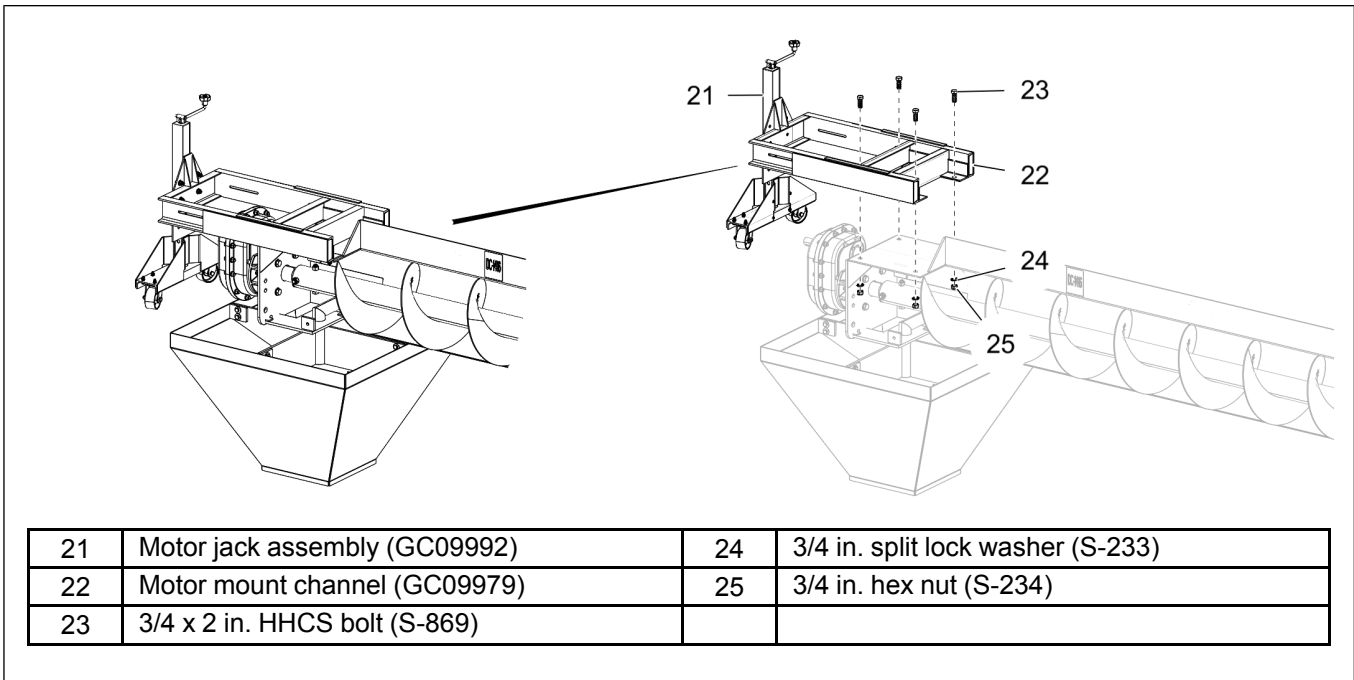
Figure 2-2 Removing the motor frame
