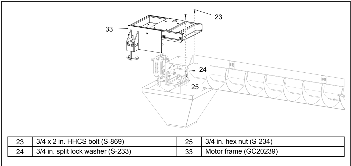
Figure 2-8 Installing the new motor frame to the sweep center section
