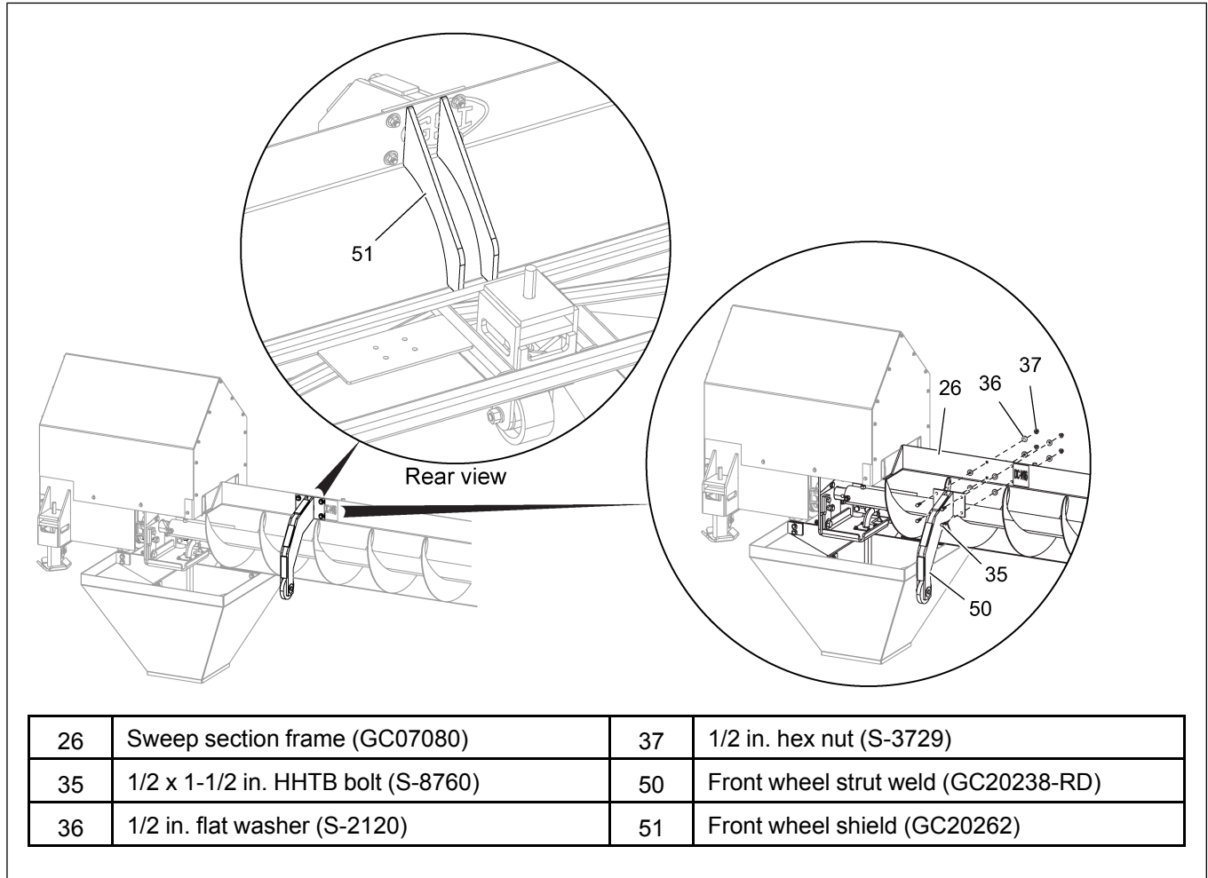
Figure 2-15 Assembling the front wheel strut
