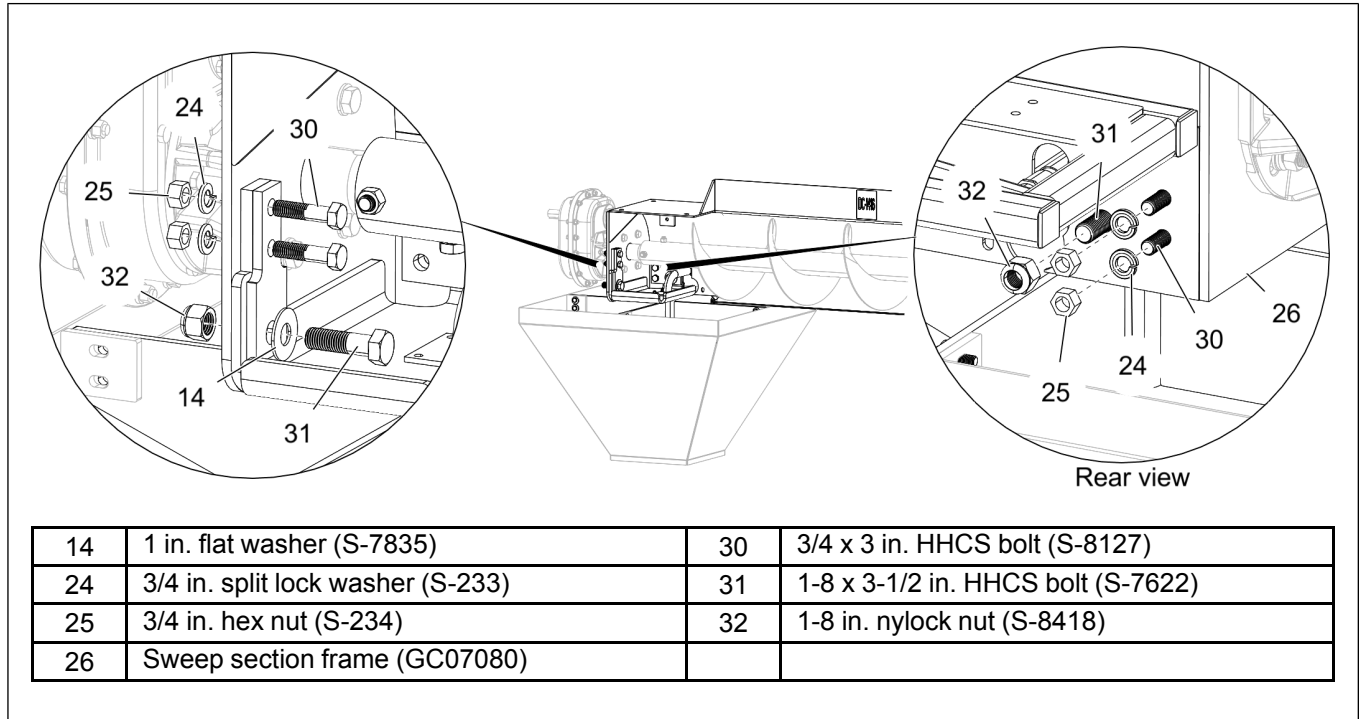
Figure 2-6 Attaching the sweep section to the spider assembly
