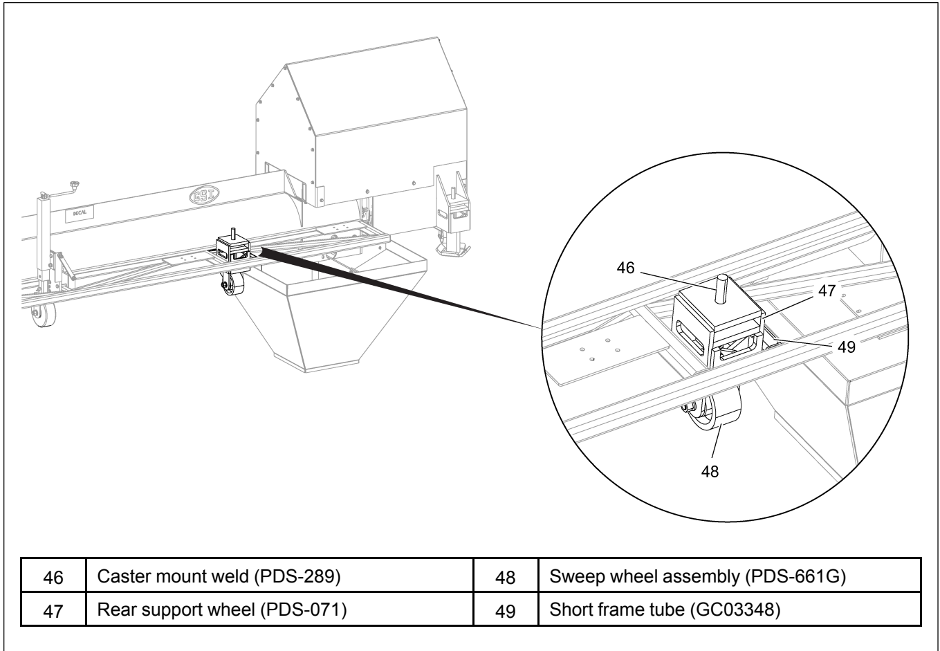
Figure 2-14 Welding the rear support and wheel assembly
