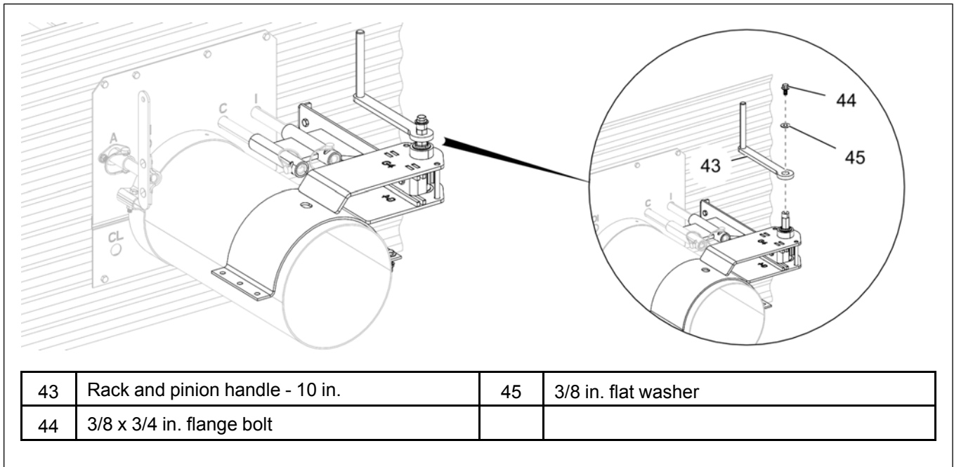
Figure 3-23 Installing the handle to rack and pinion - 10 in. (gate opening side)
