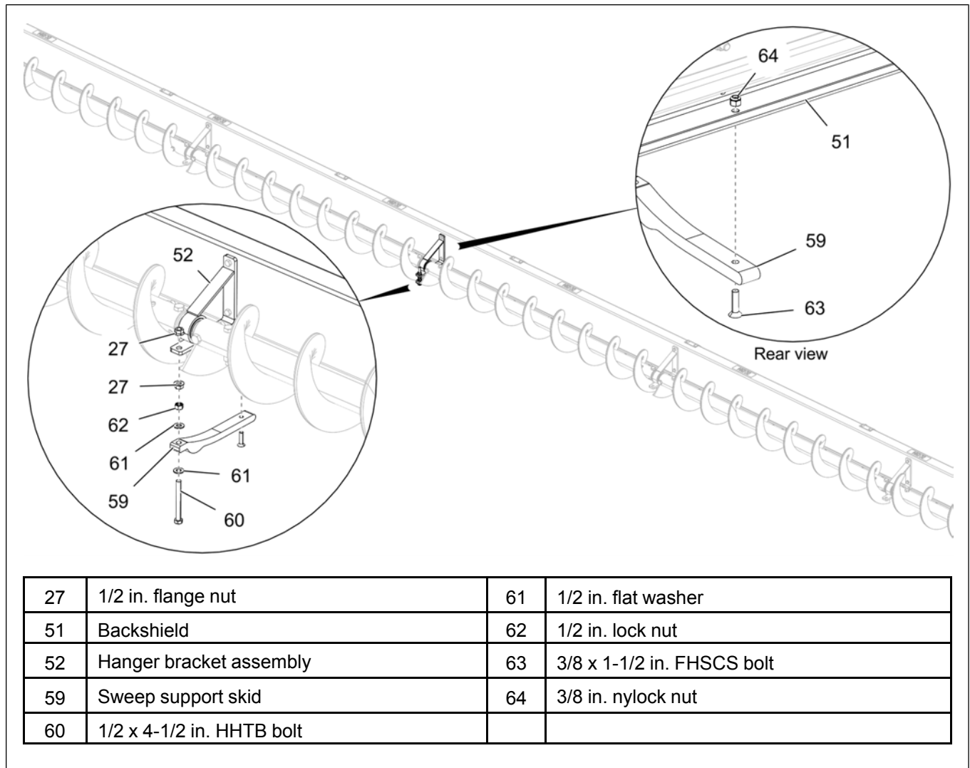
Figure 3-42 Assembling the sweep support skid
