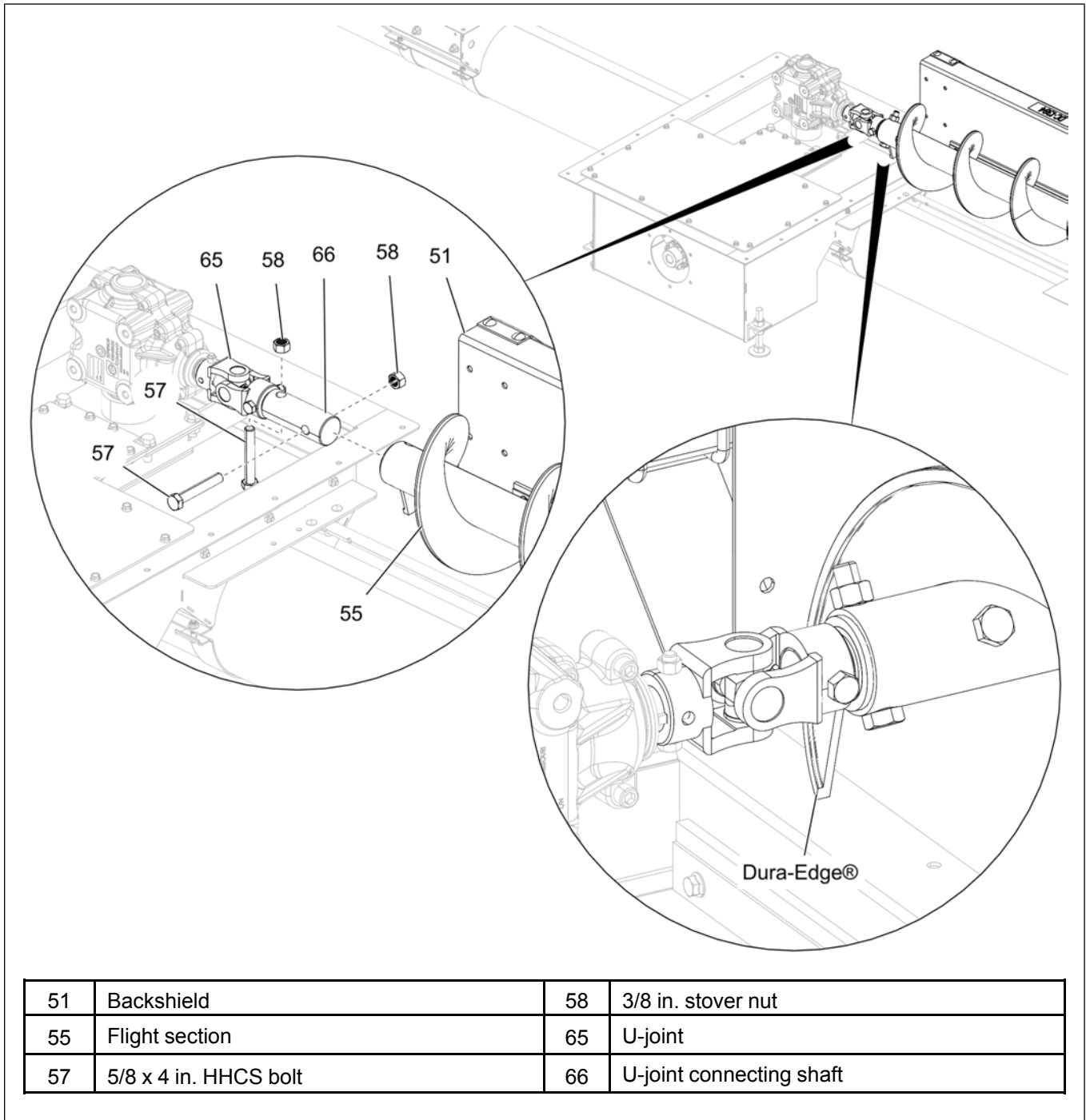
Figure 3-45 Attaching the auger to the U-joint
