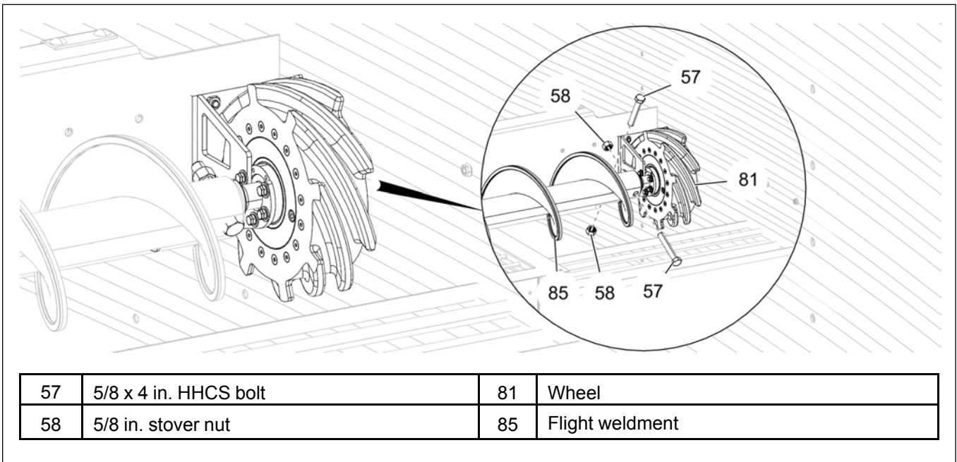
Figure 3-50 Installing the wheel to auger
