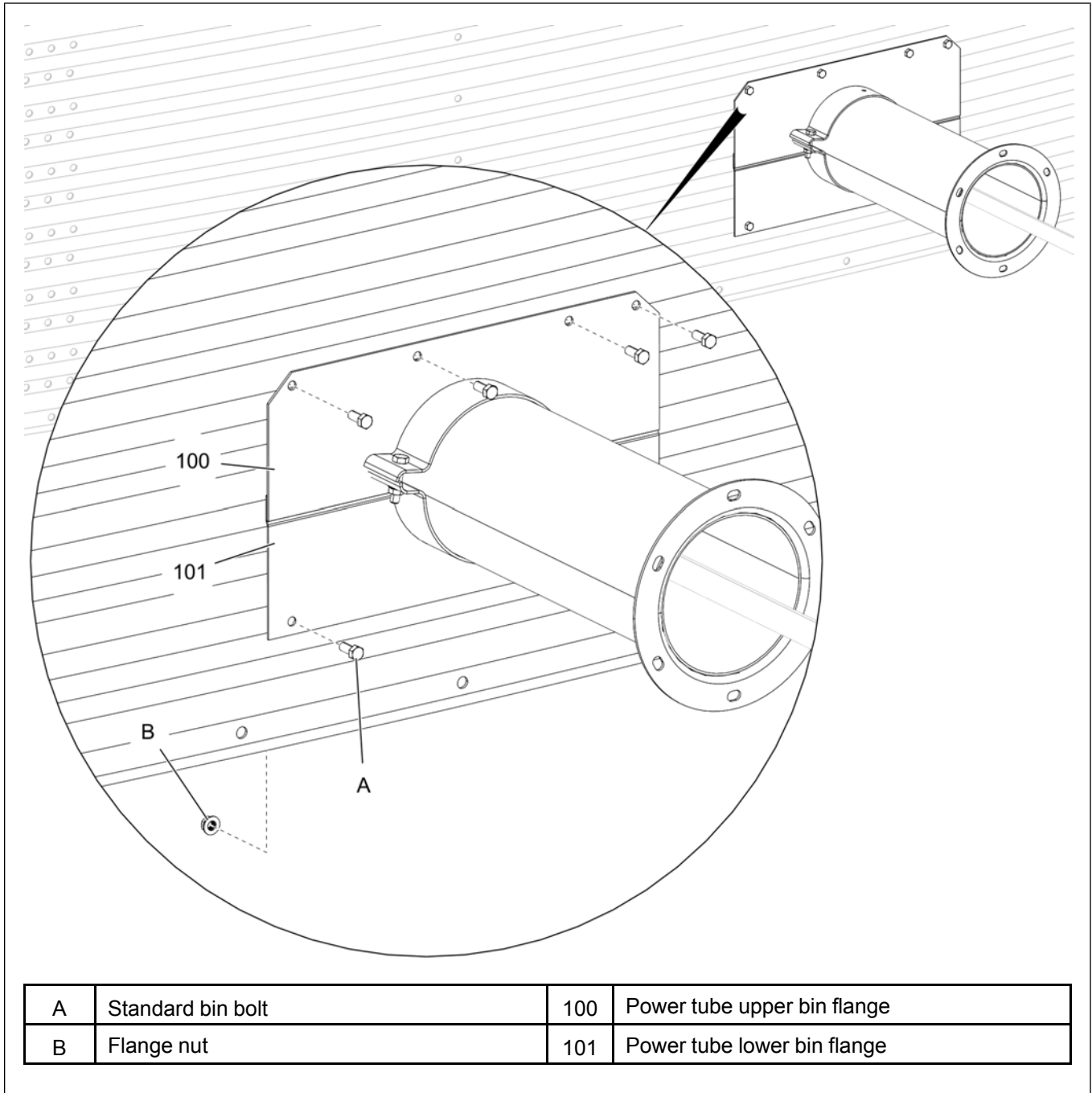
Figure 3-62 Secure the upper and lower bin flanges
