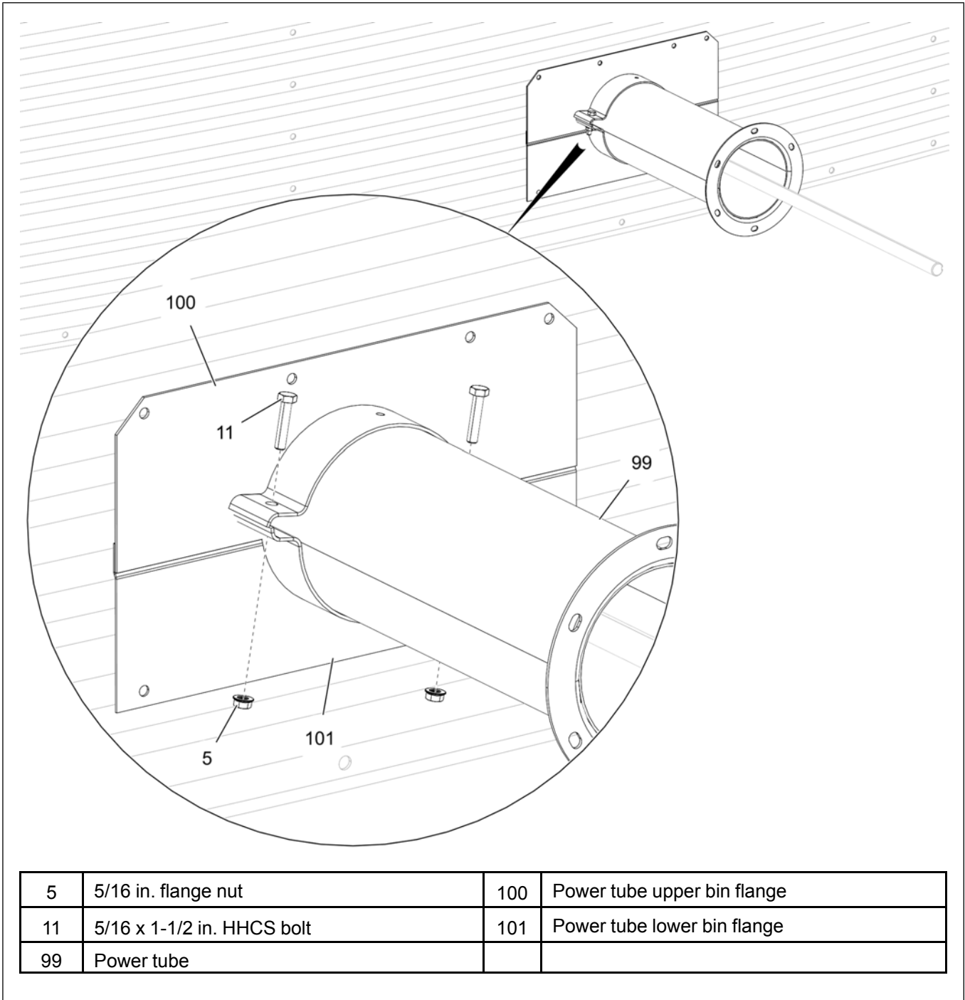
Figure 3-61 Installing the upper and lower bin flanges for power tube
