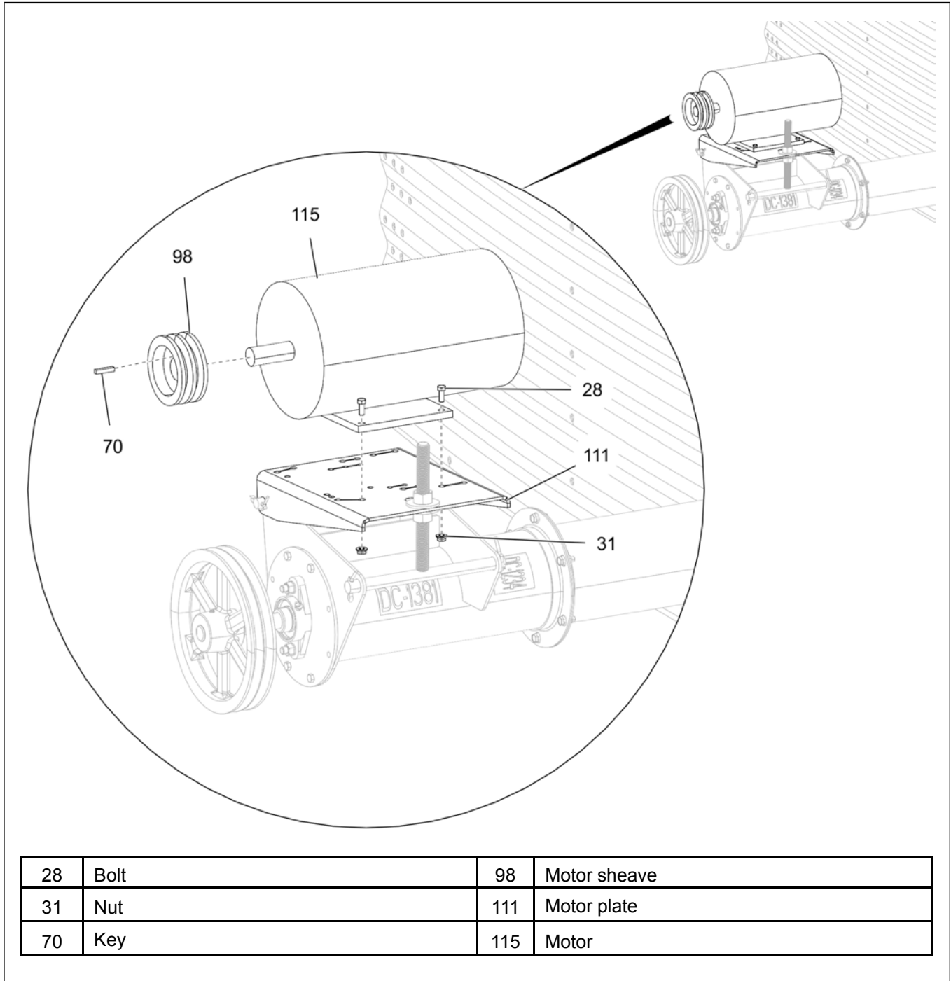
Figure 3-67 Installing the motor
