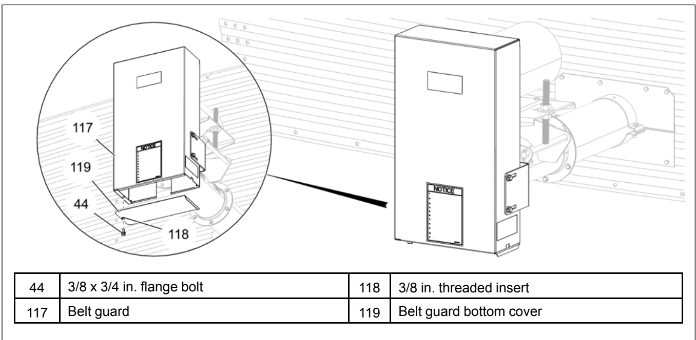
Figure 3-71 Installing the belt guard bottom cover
