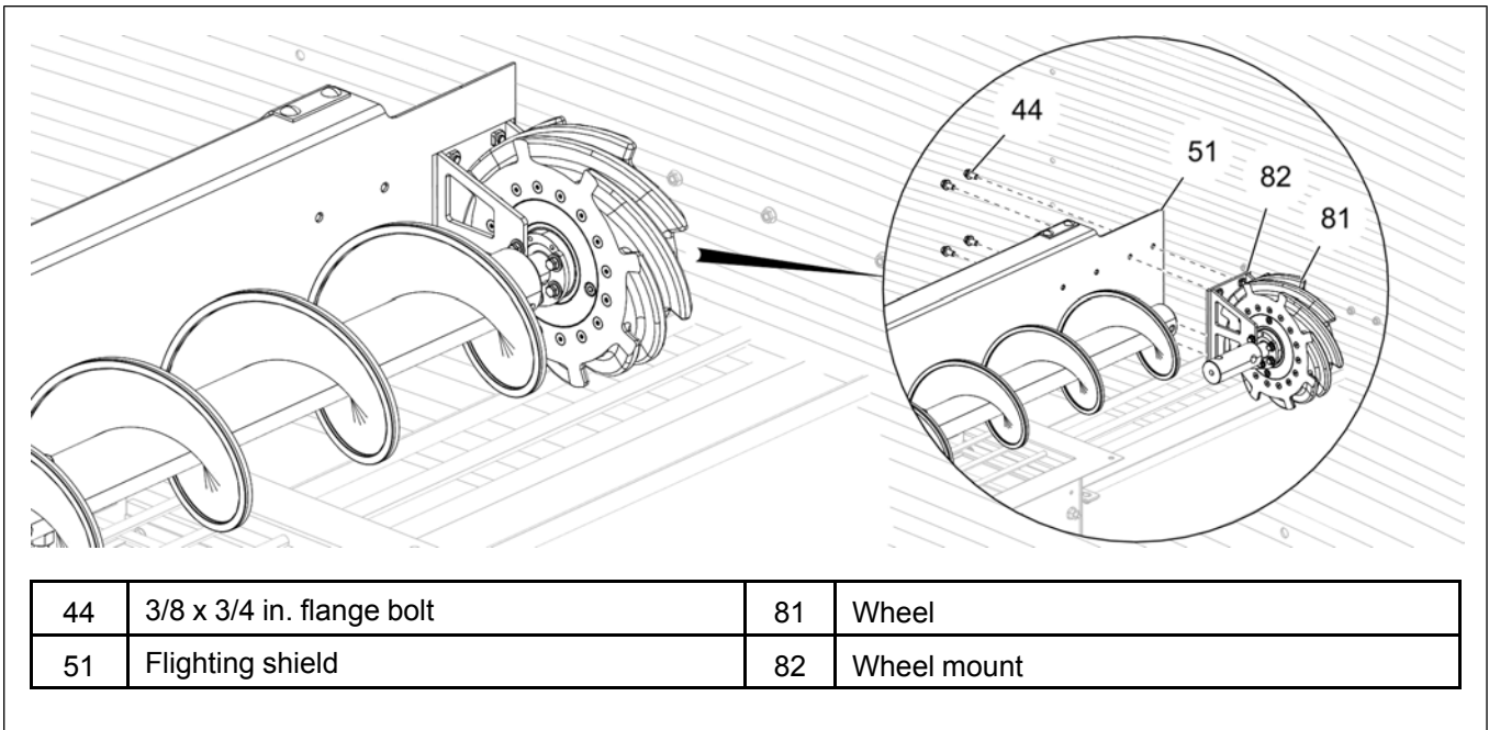
Figure 3-49 Attaching the wheel mount to shield
