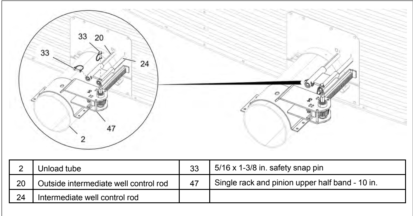
Figure 3-27 Installing the rack and pinion - 10 in. (opposite side)
