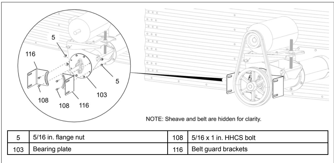
Figure 3-69 Installing the belt guard brackets
