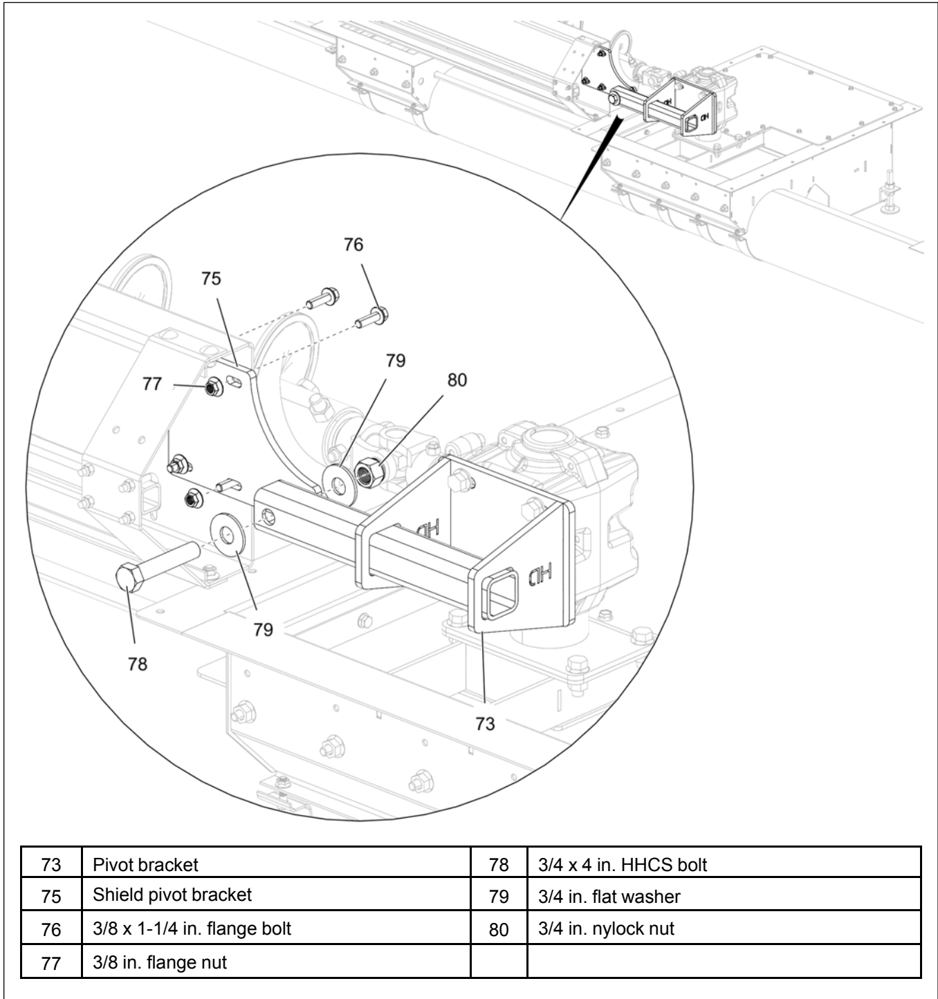
Figure 3-47 Attaching the flighting shield pivot bracket to pivot bracket
