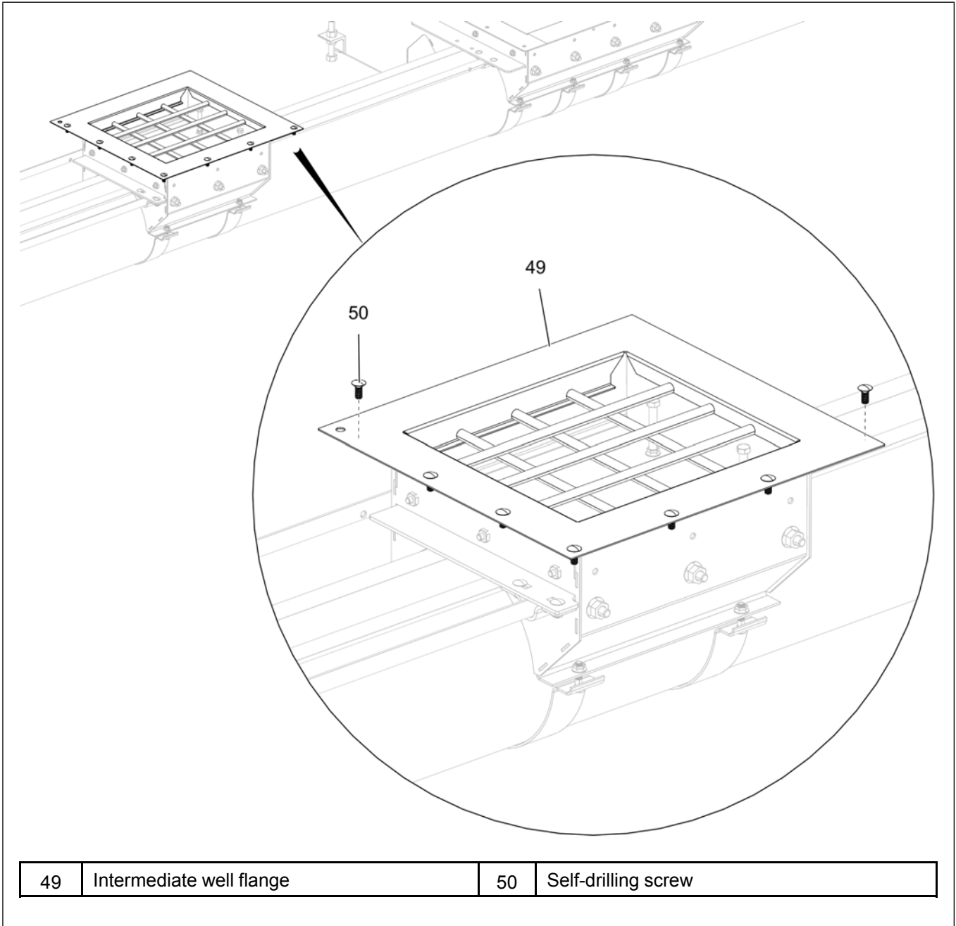
Figure 3-39 Installing the intermediate well flange
