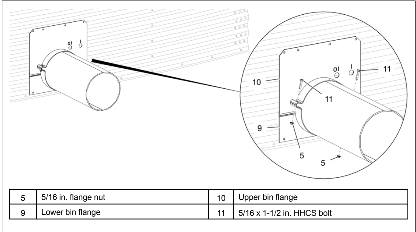
Figure 3-6 Installing the upper and lower bin flanges (opposite side)
