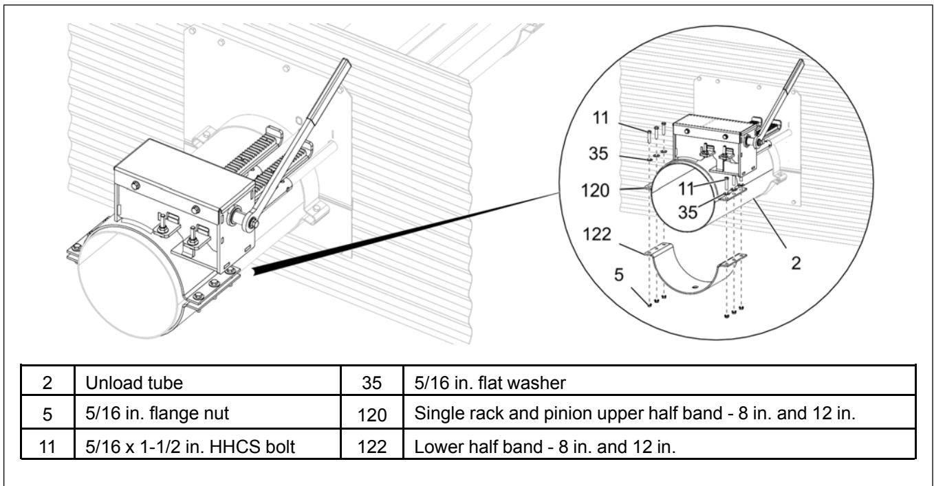
Figure 3-32 Installing the lower half band to rack and pinion - 8 in. and 12 in. (opposite side)
