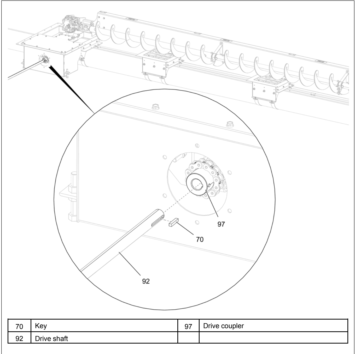
Figure 3-60 Installing the drive shaft to the center well drive coupler
