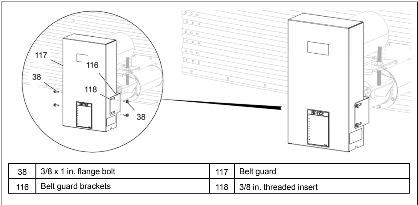
Figure 3-70 Installing the belt guard
