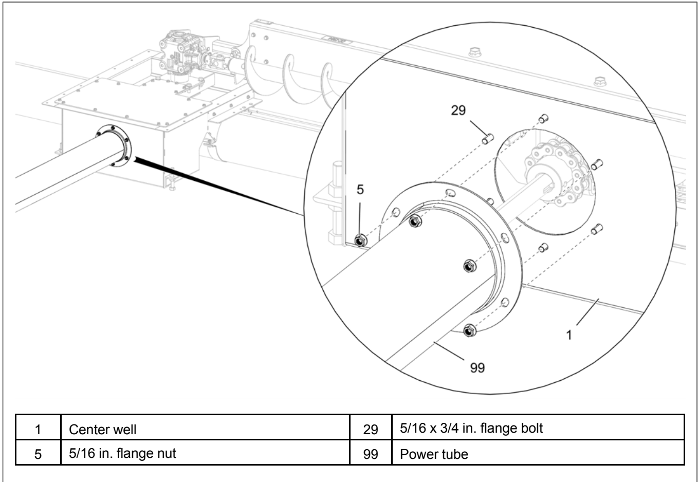
Figure 3-58 Secure the power tube to the center well
