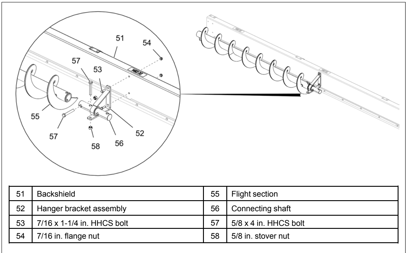
Figure 3-40 Attaching the first flight section with hanger bracket to the backshield
