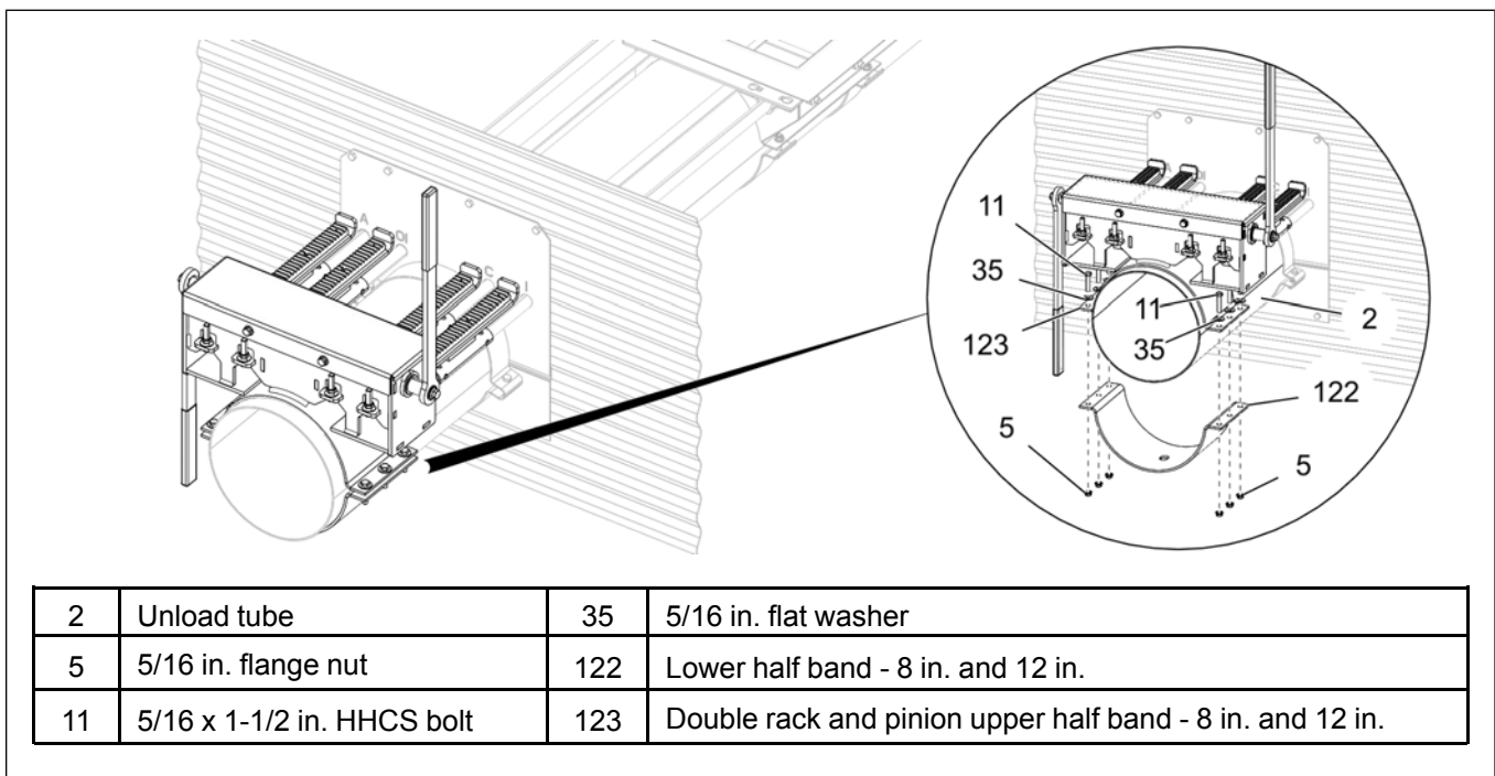
Figure 3-38 Installing the lower half band to double rack and pinion - 8 in. and 12 in.
