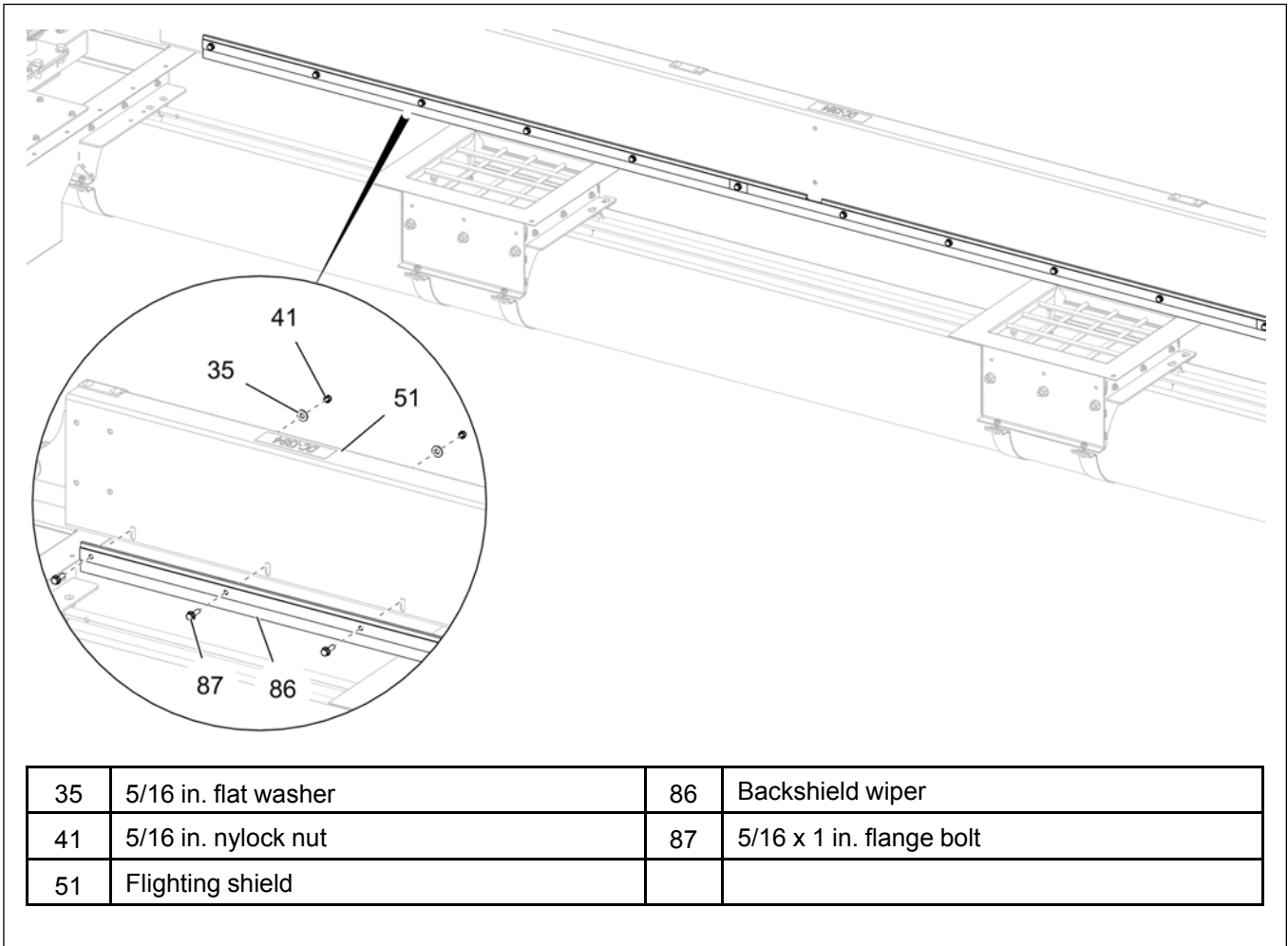
Figure 3-51 Wiper in UP position
