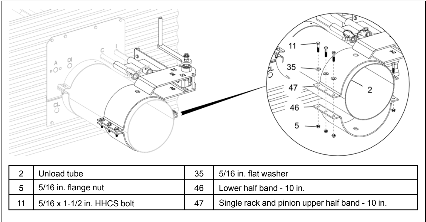
Figure 3-25 Installing the lower half band to rack and pinion - 10 in. (gate opening side)
