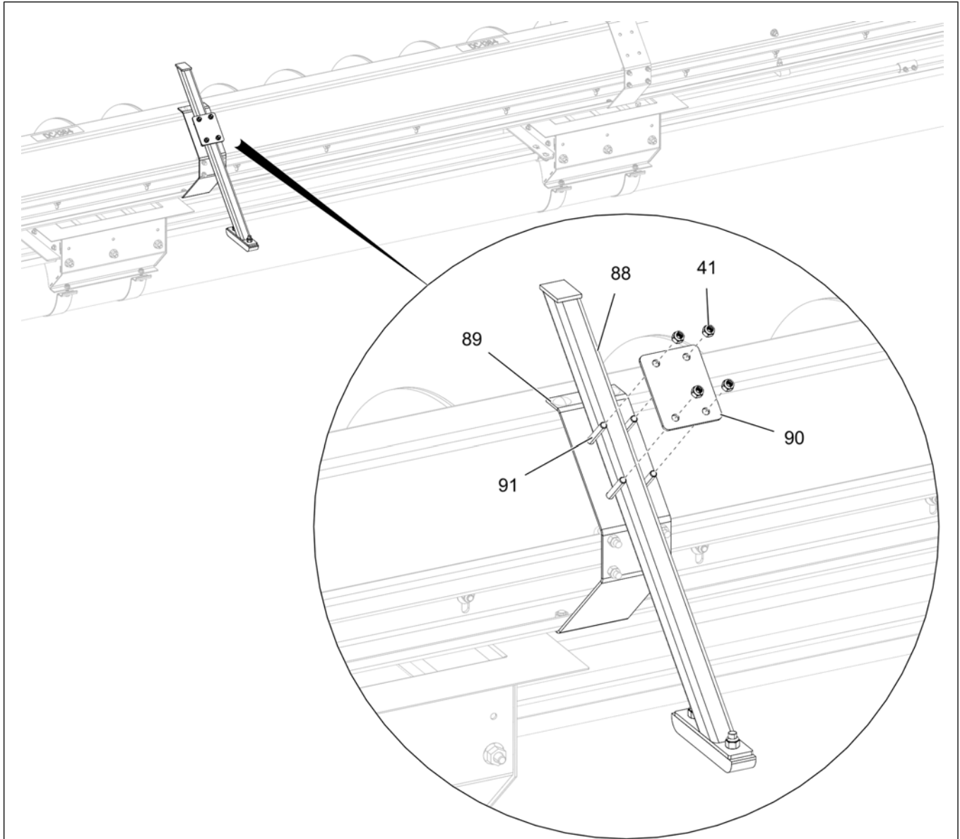
Figure 3-54 Installing the backshield support assembly
