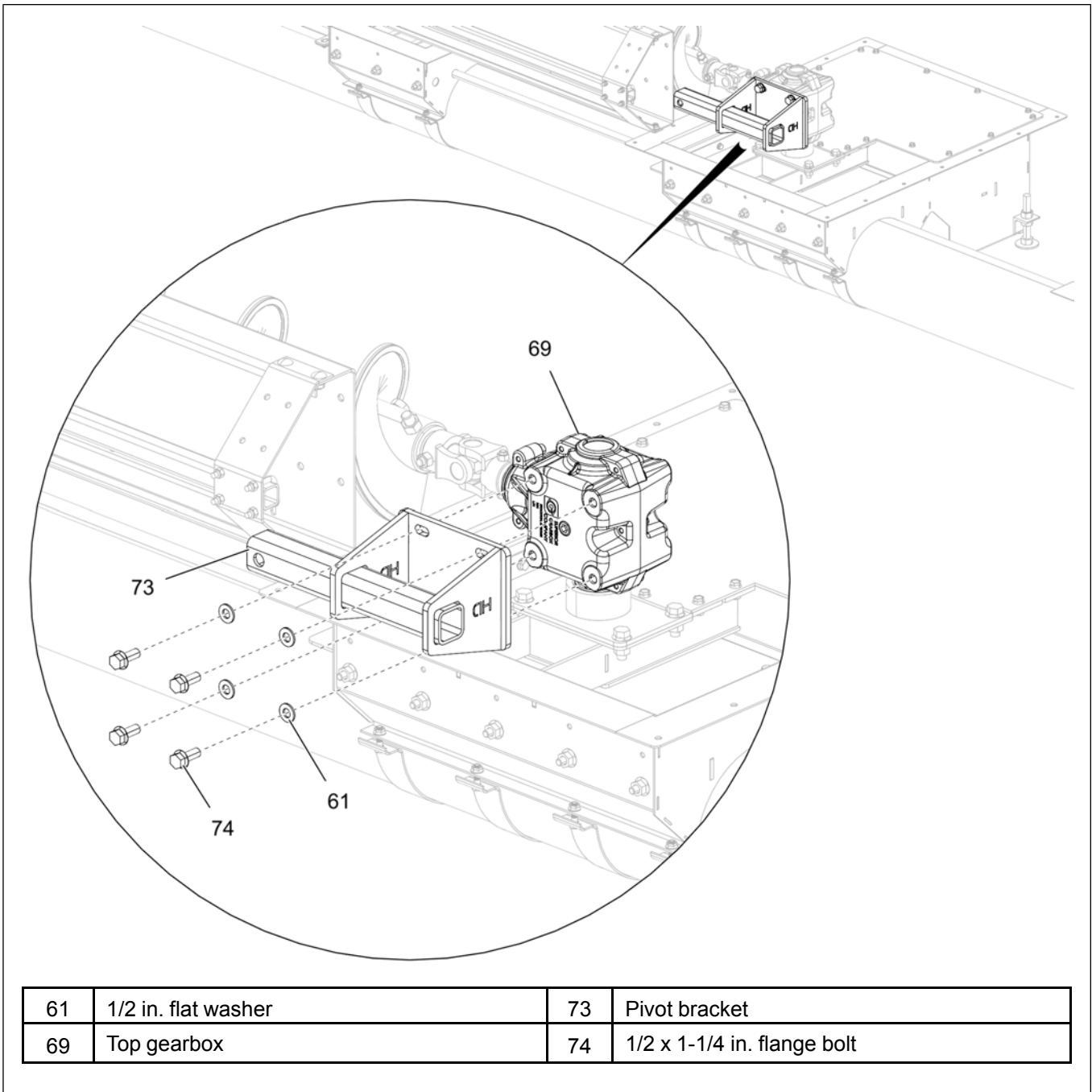
Figure 3-46 Attaching the pivot bracket to the gearbox
