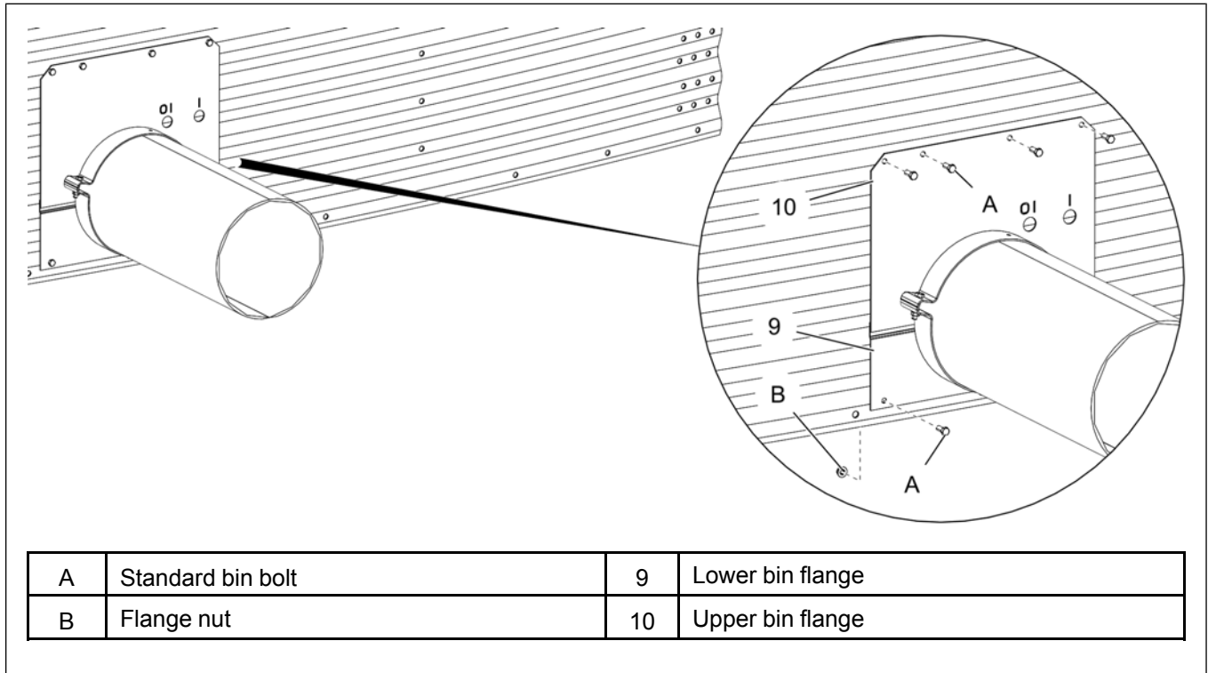
Figure 3-7 Secure the upper and lower bin flanges (opposite side)
