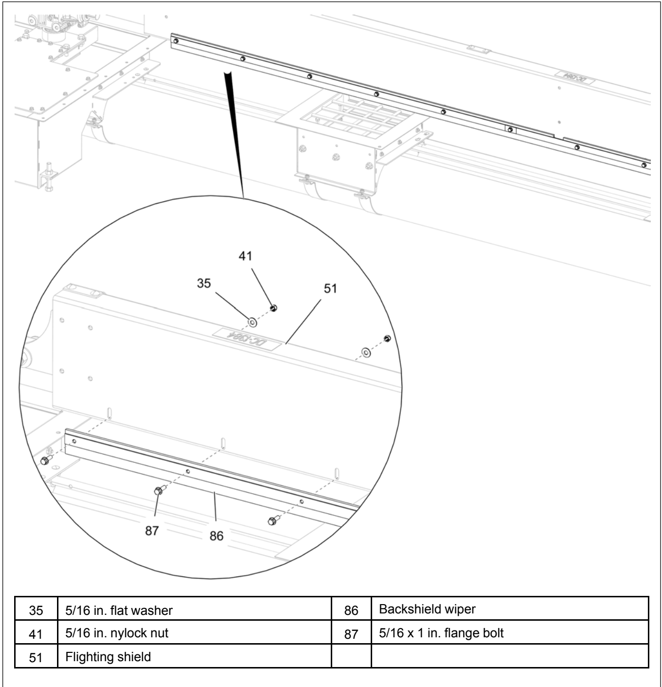
Figure 3-52 Wiper in DOWN position
