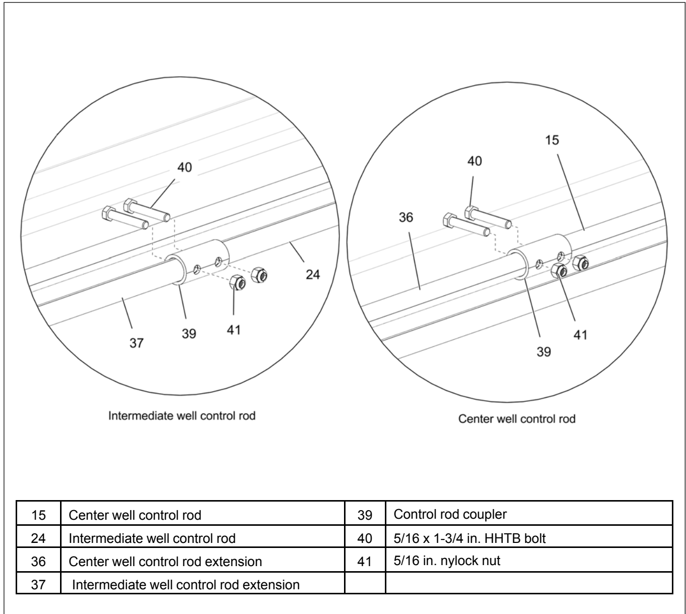
Figure 3-20 Connecting the control rods
