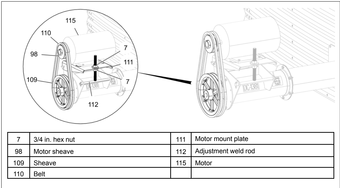
Figure 3-68 Installing the belt
