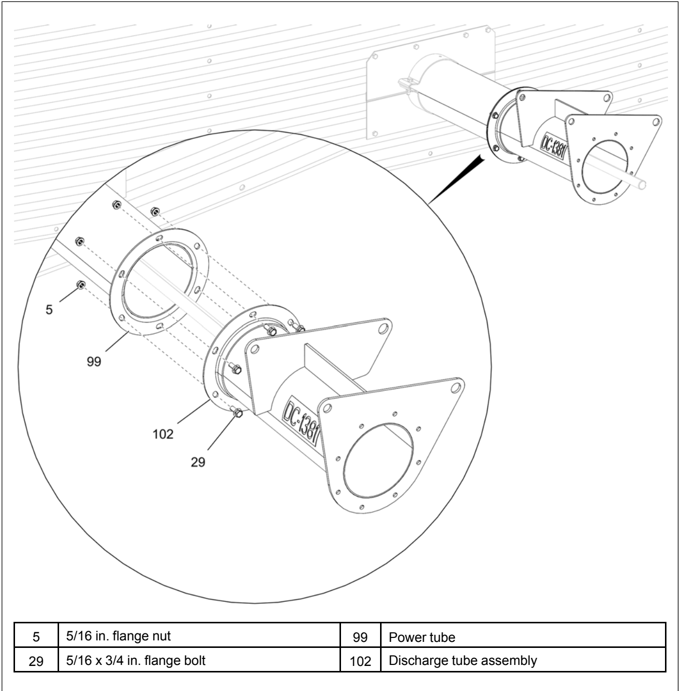
Figure 3-63 Attaching the power tube assembly to the drive head tube assembly
