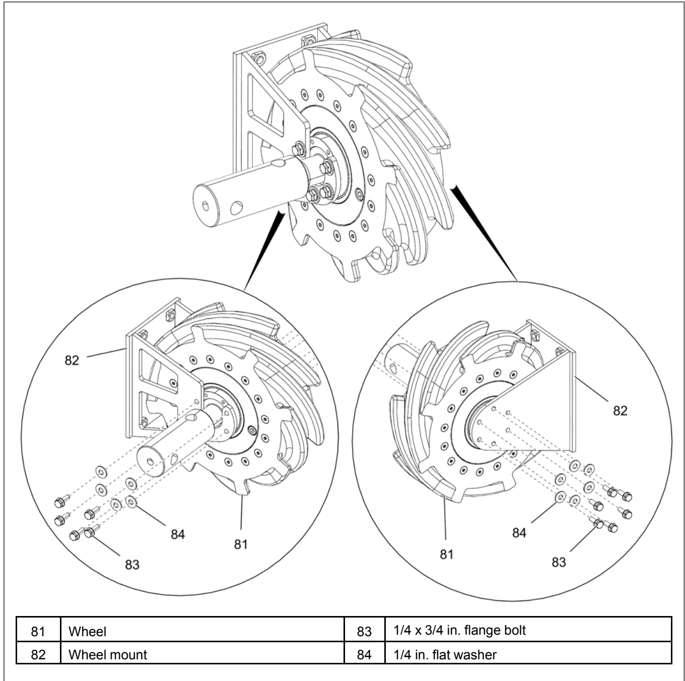
Figure 3-48 Attaching the wheel to wheel mount
