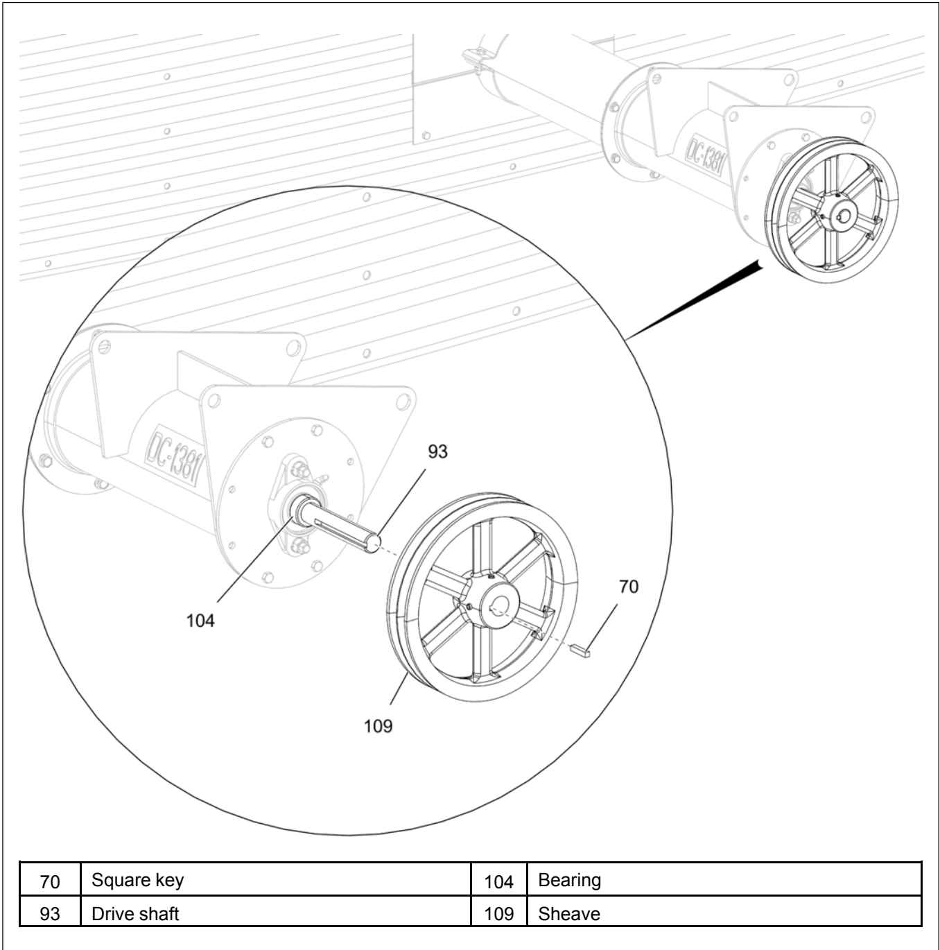
Figure 3-65 Installing the sheave to the drive shaft
