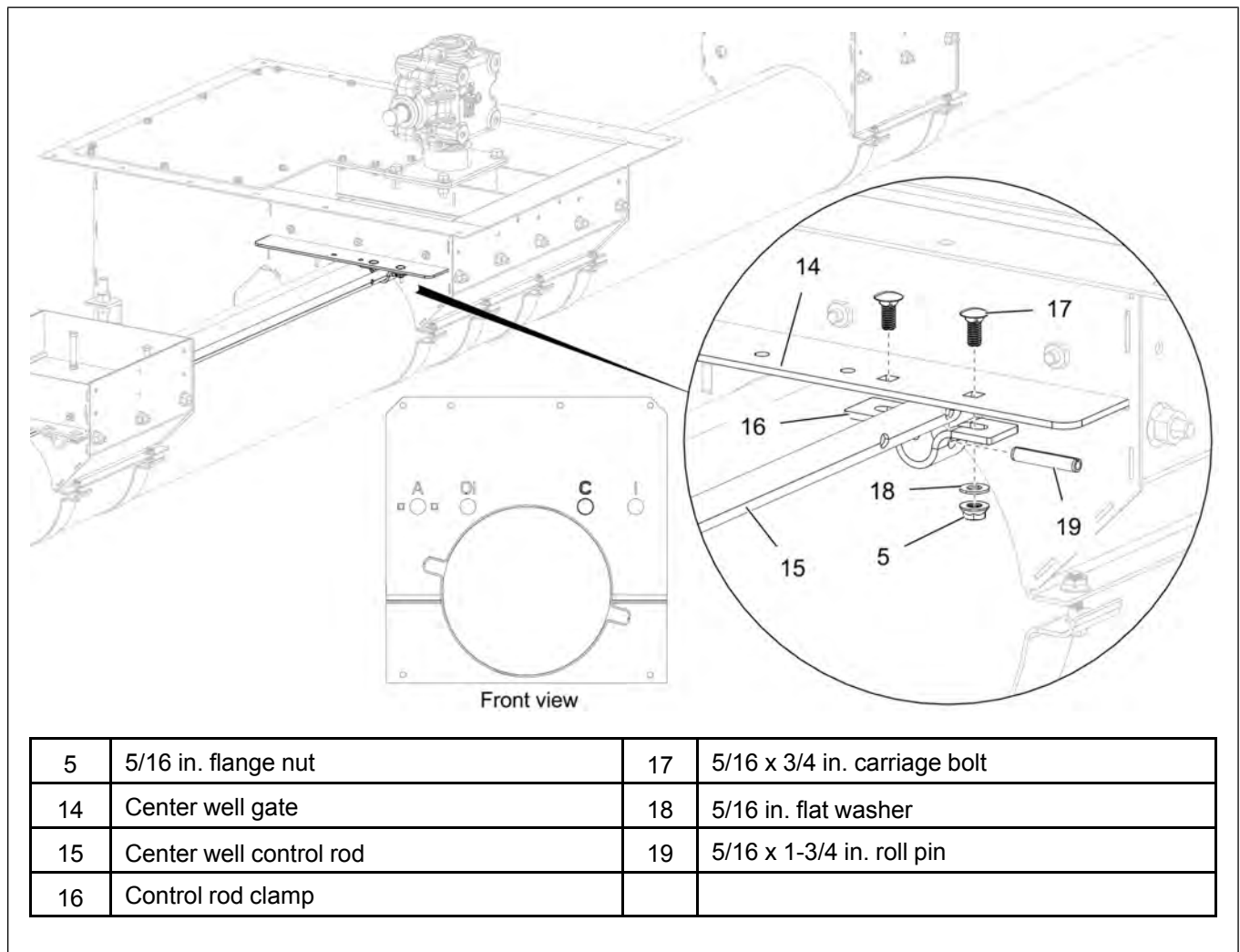
Figure 3-11 Center well gate assembly
