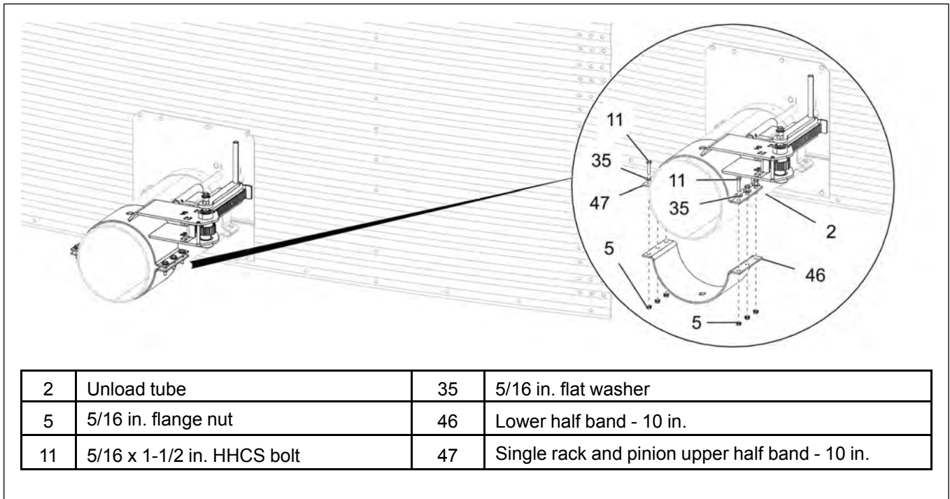
Figure 3-31 Installing the lower half band to rack and pinion - 10 in. (opposite side)
