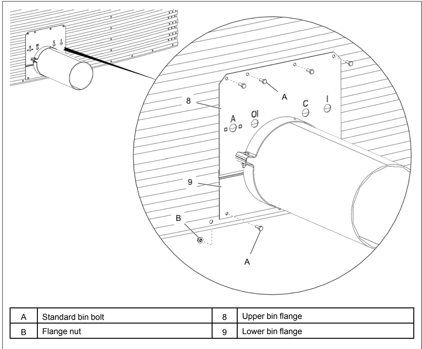
Figure 3-5 Secure the upper and lower bin flanges (gate side)
