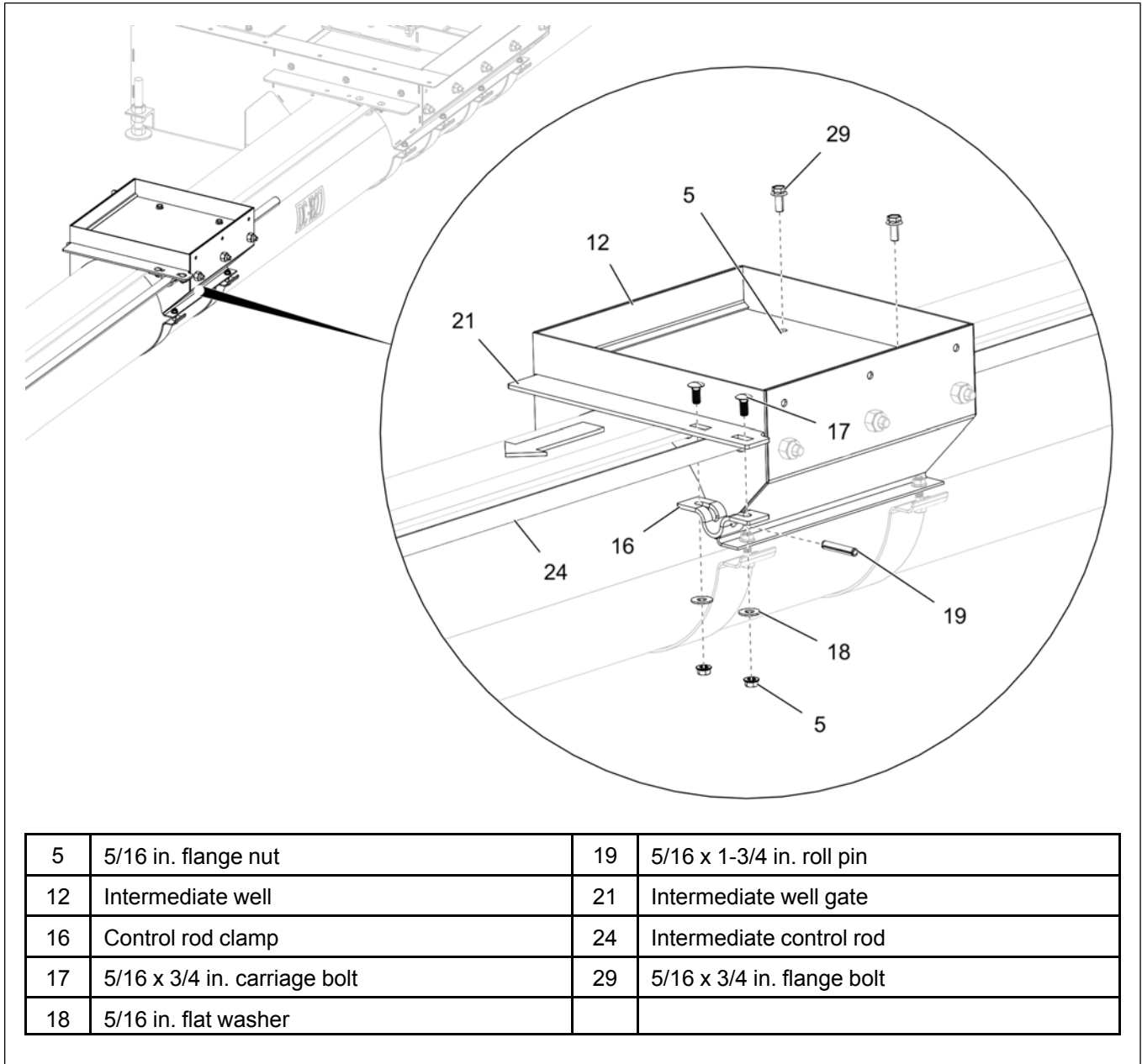
Figure 3-14 Removing the intermediate gate (10 in. sweep)
