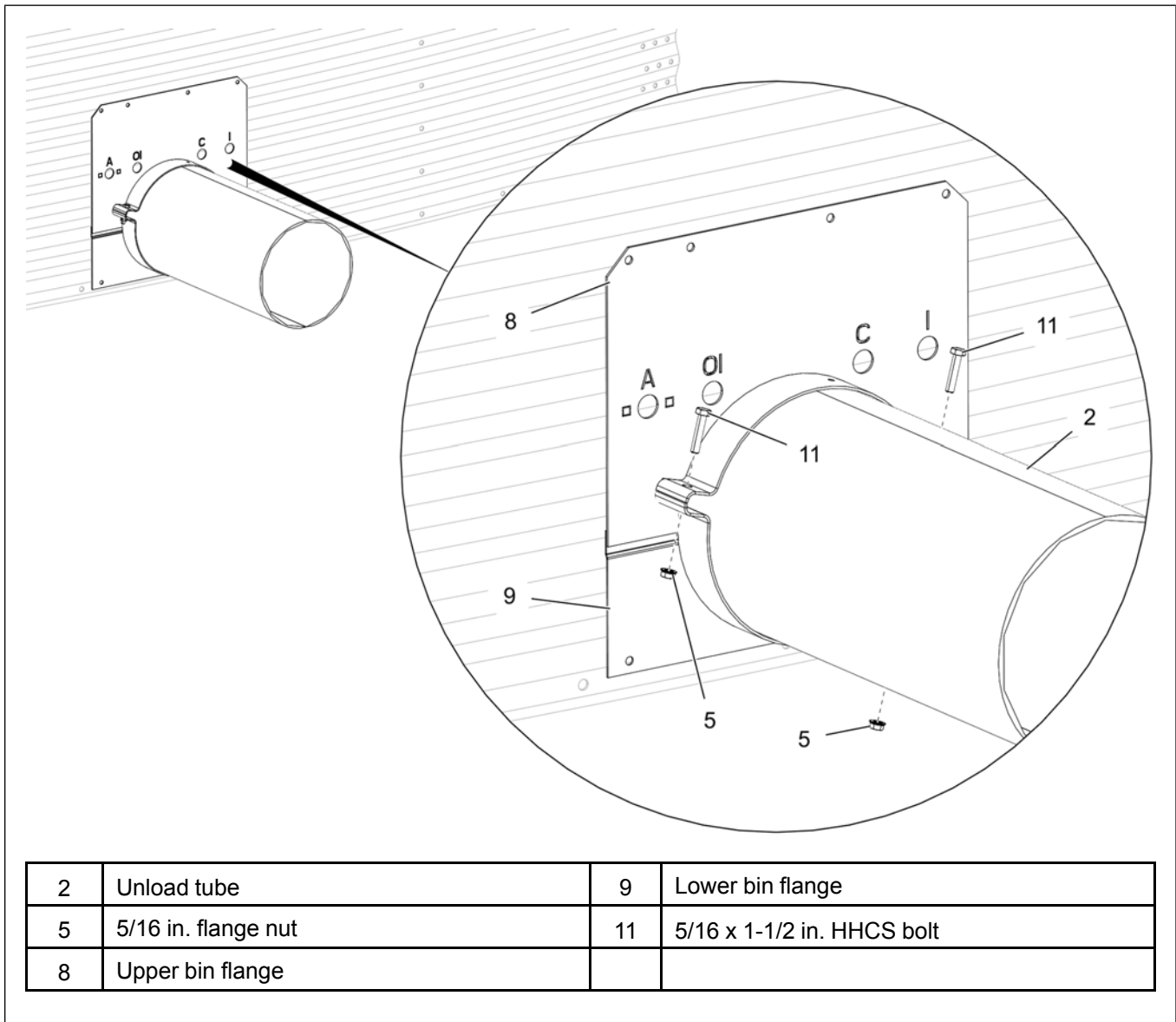
Figure 3-4 Installing the upper and lower bin flanges (gate side)
