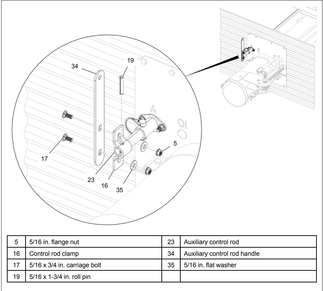
Figure 3-19 Installing the auxiliary control lever
