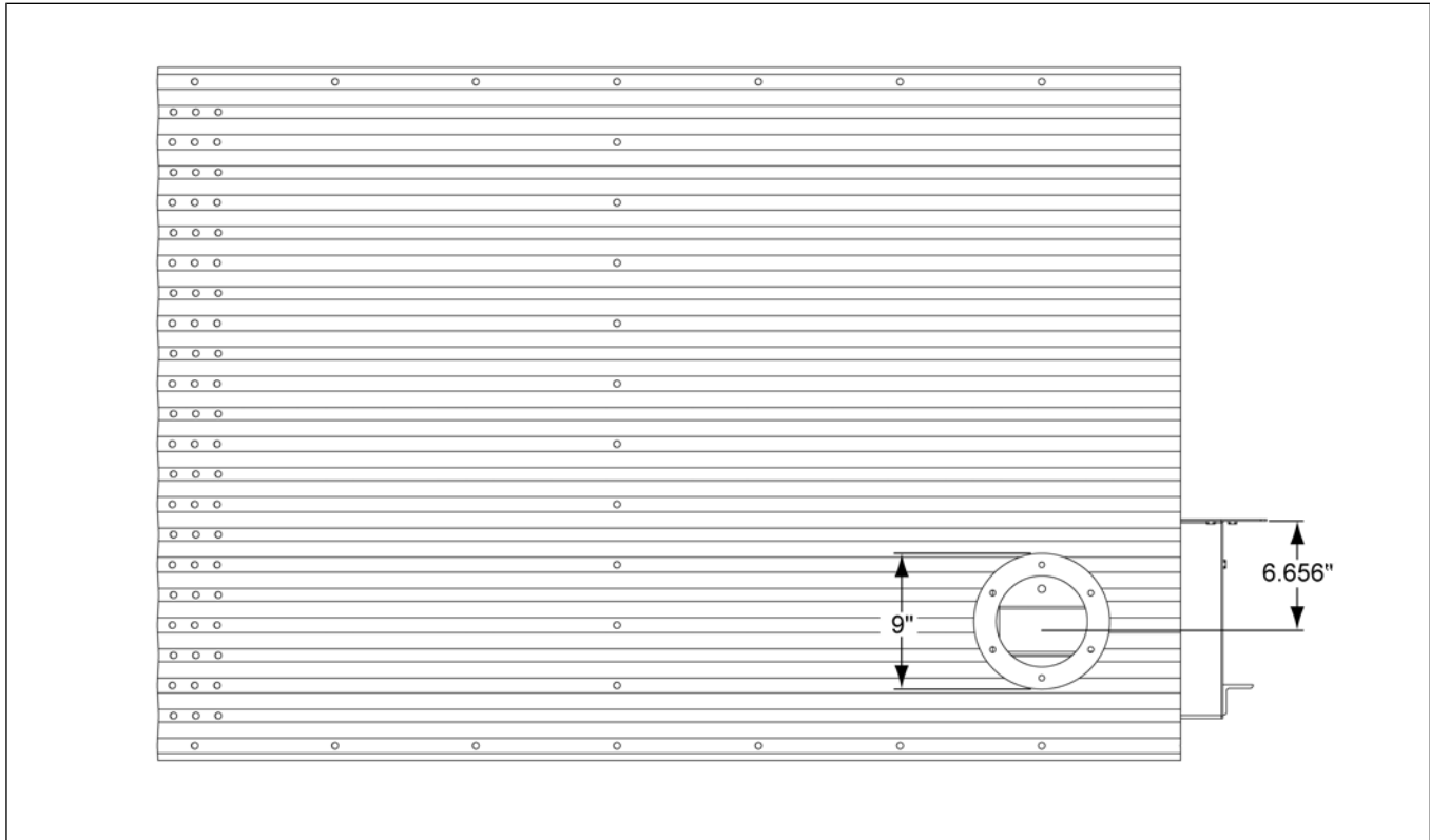
Figure 3-57 Sidewall opening details (power tube)
