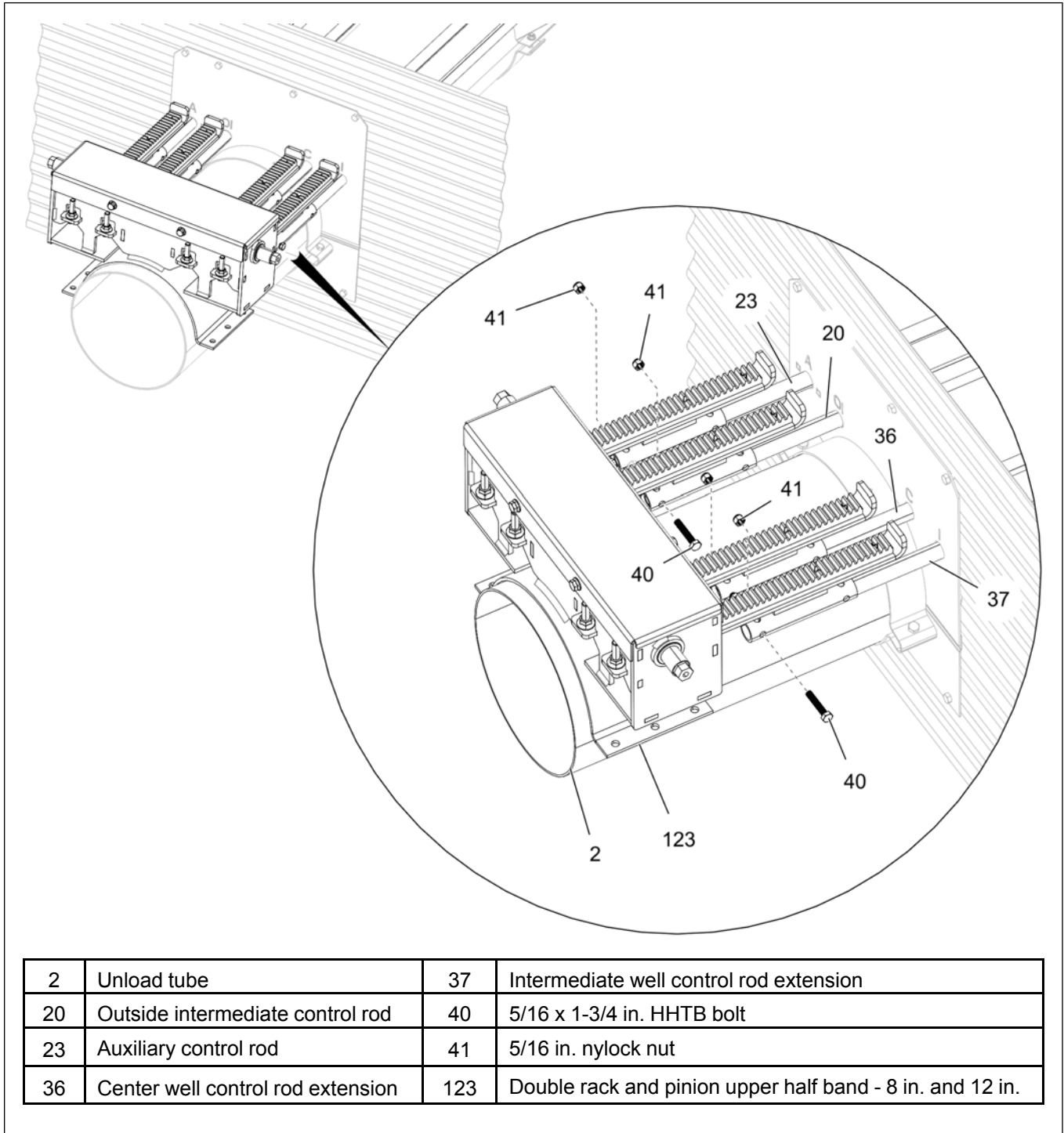
Figure 3-34 Installing the double rack and pinion - 8 in. and 12 in.
