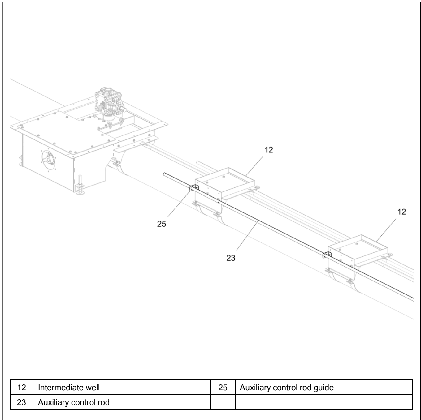
Figure 3-15 Sliding the auxiliary control rod through rod guide bracket
