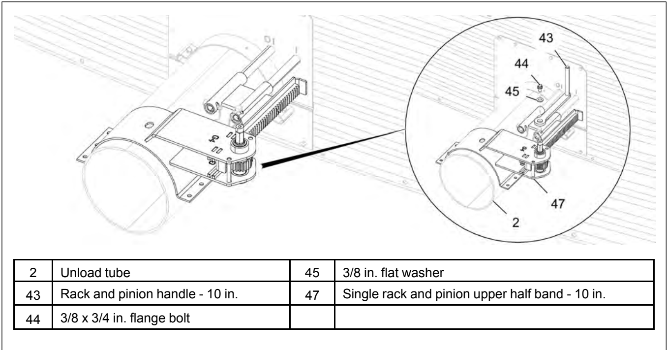
Figure 3-29 Installing the handle to rack and pinion - 10 in. (opposite side)
