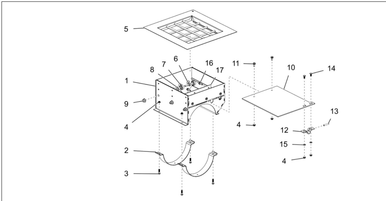
Figure 7-2 Intermediate well parts
