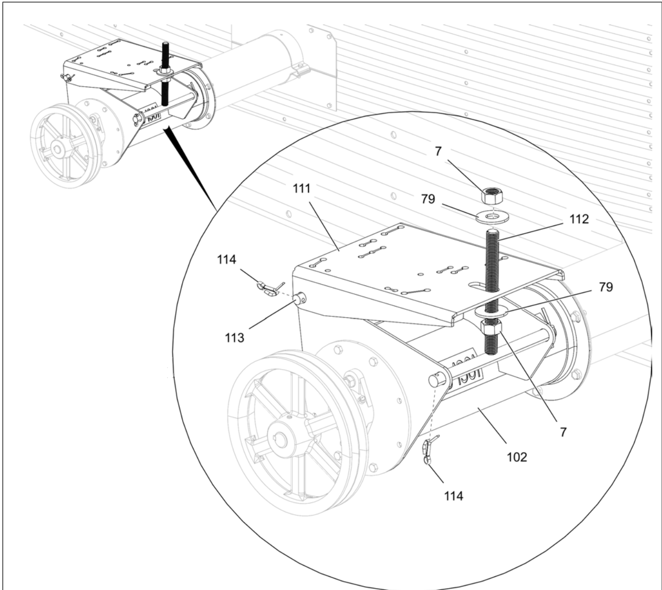
Figure 3-66 Installing the motor mount plate
