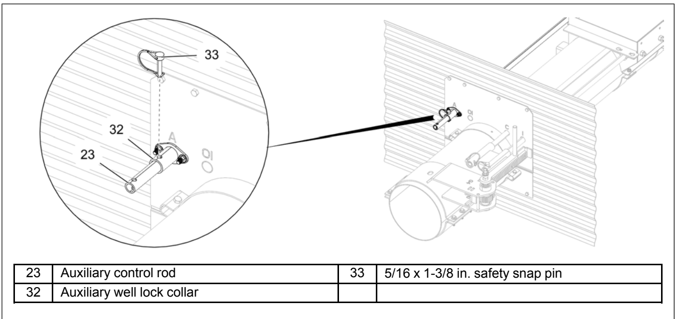
Figure 3-18 Installing the lock pin
