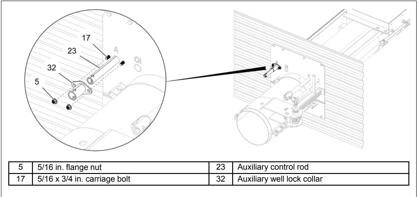
Figure 3-17 Installing the auxiliary well lock collar to bin flange
