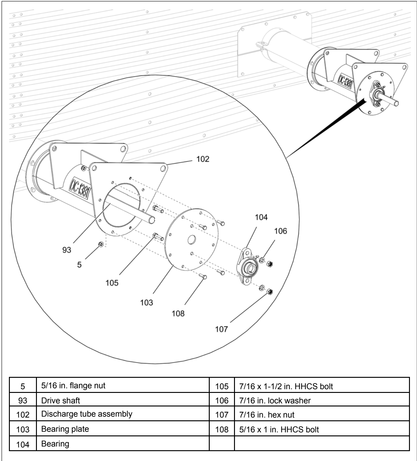
Figure 3-64 Assembling the bearing and bearing plate to the drive head tube
