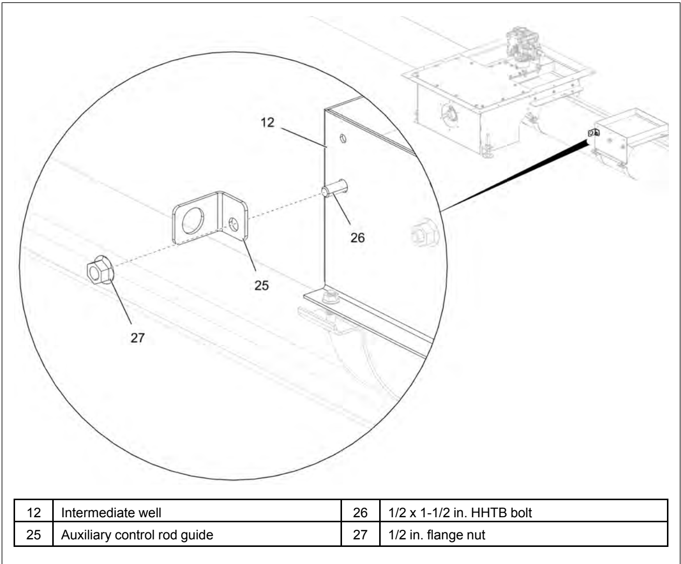
Figure 3-13 Installing the auxiliary rod guide to intermediate well
