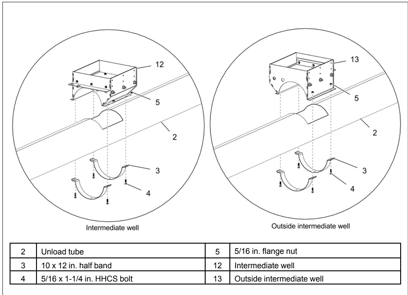
Figure 3-9 Installing the intermediate wells
