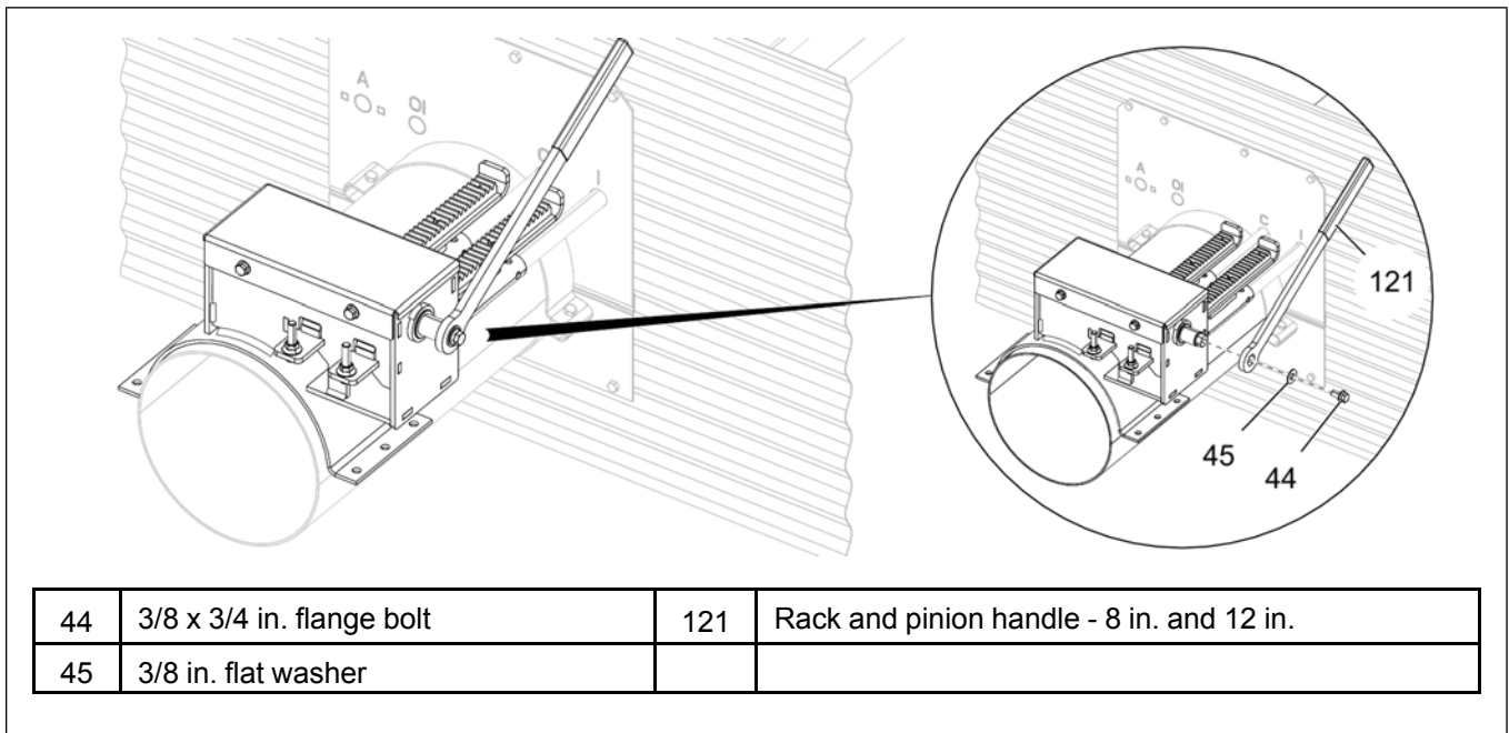
Figure 3-24 Installing the handle to rack and pinion - 8 in. and 12 in. (gate opening side)
