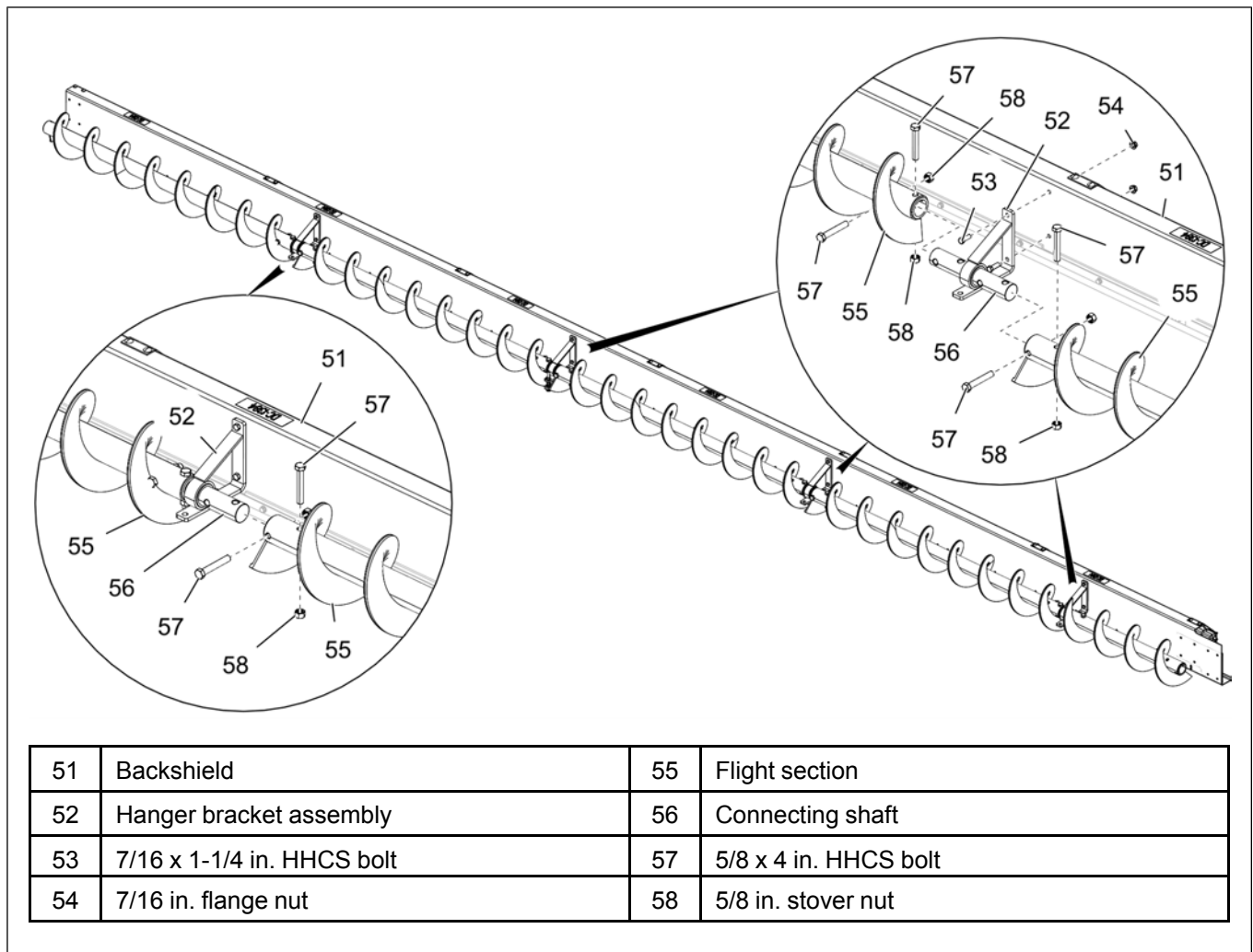
Figure 3-41 Attaching the second flight section with hanger bracket to the backshield
