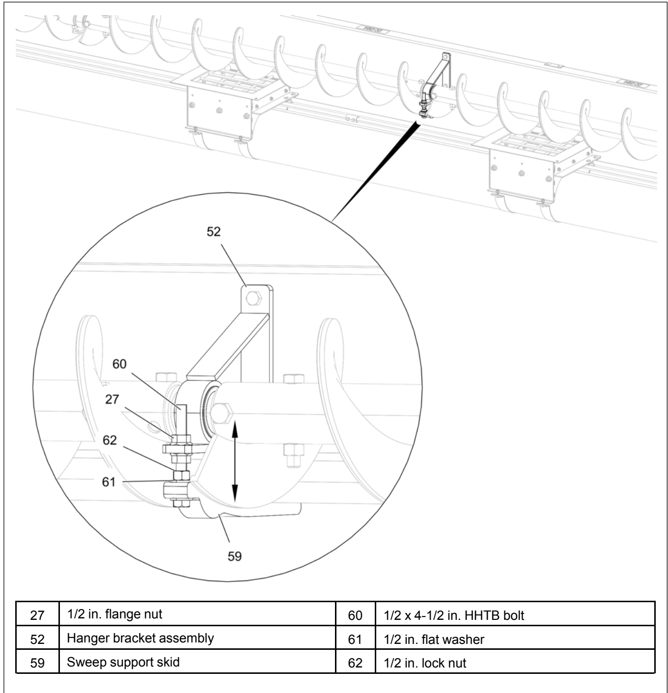
Figure 3-53 Adjusting the sweep support skid
