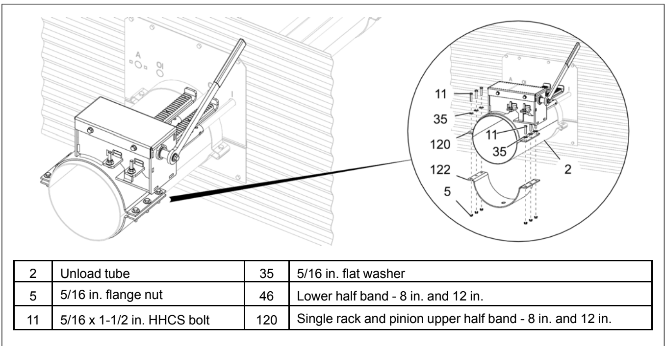
Figure 3-26 Installing the lower half band to rack and pinion - 8 in. and 12 in. (gate opening side)
