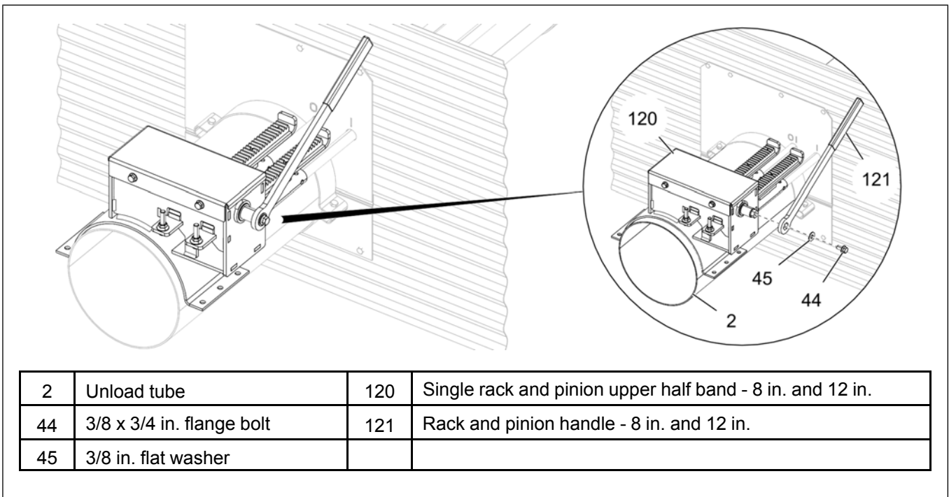
Figure 3-30 Installing the handle to rack and pinion - 8 in and 12 in. (opposite side)
