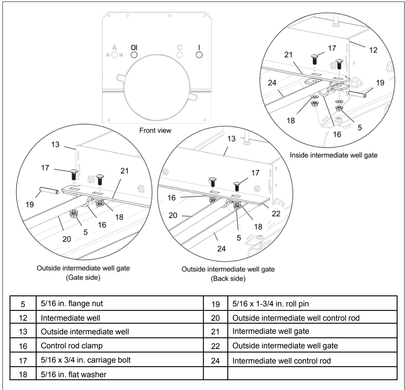
Figure 3-12 Intermediate well gate assembly
