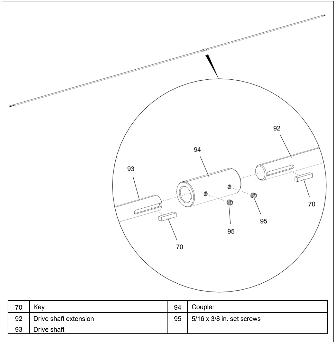
Figure 3-59 Assembling the drive shafts (42 ft - 72 ft only)
