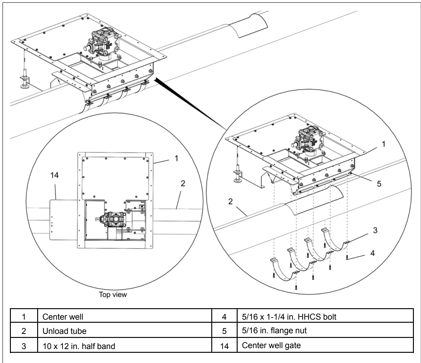
Figure 3-2 Attaching the center well to the unload tube
