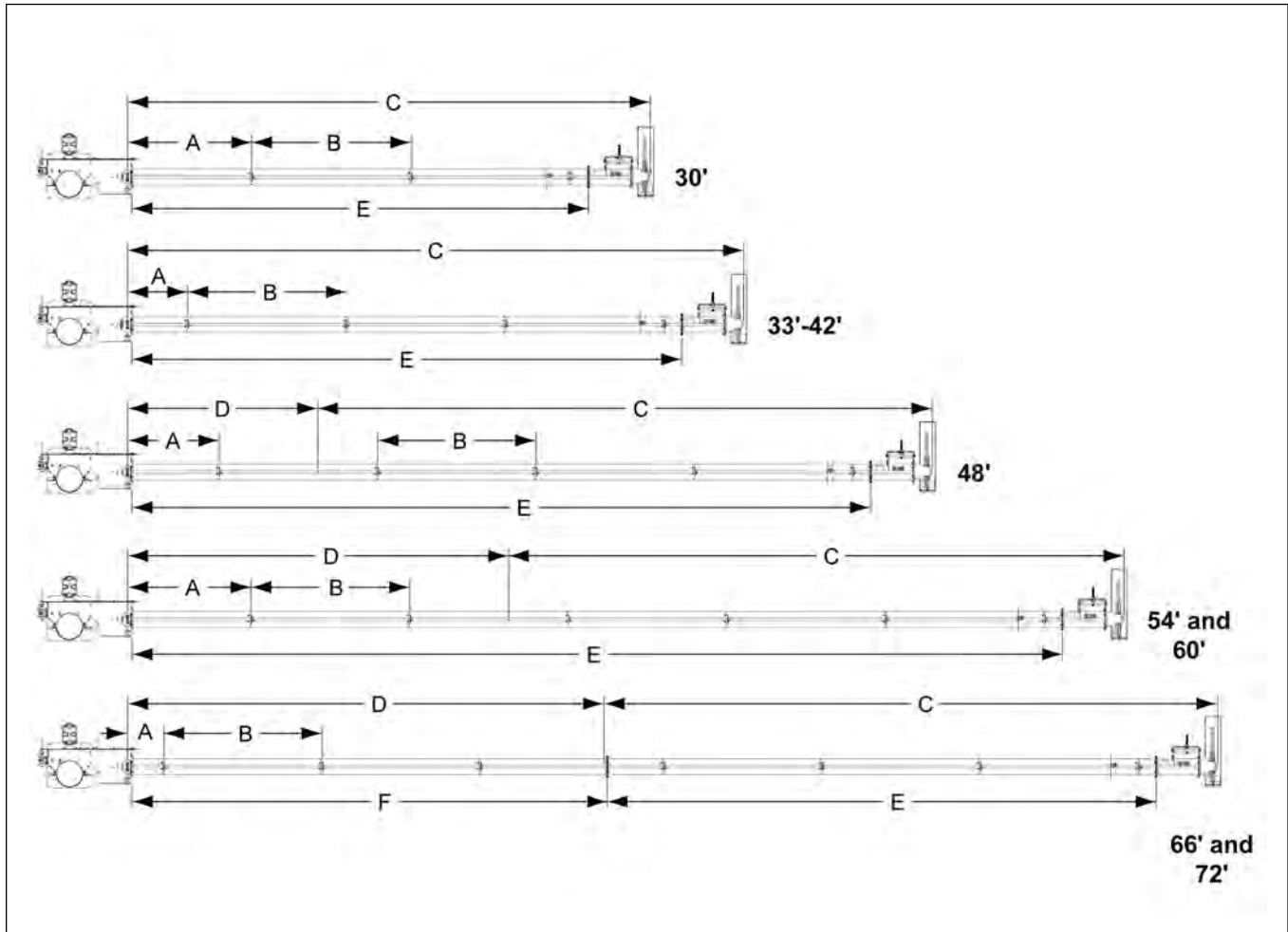
Figure 3-56 Drive assembly and power tube layout
