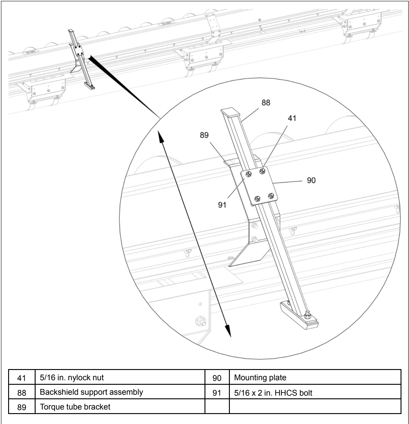
Figure 3-55 Adjusting the backshield assembly
