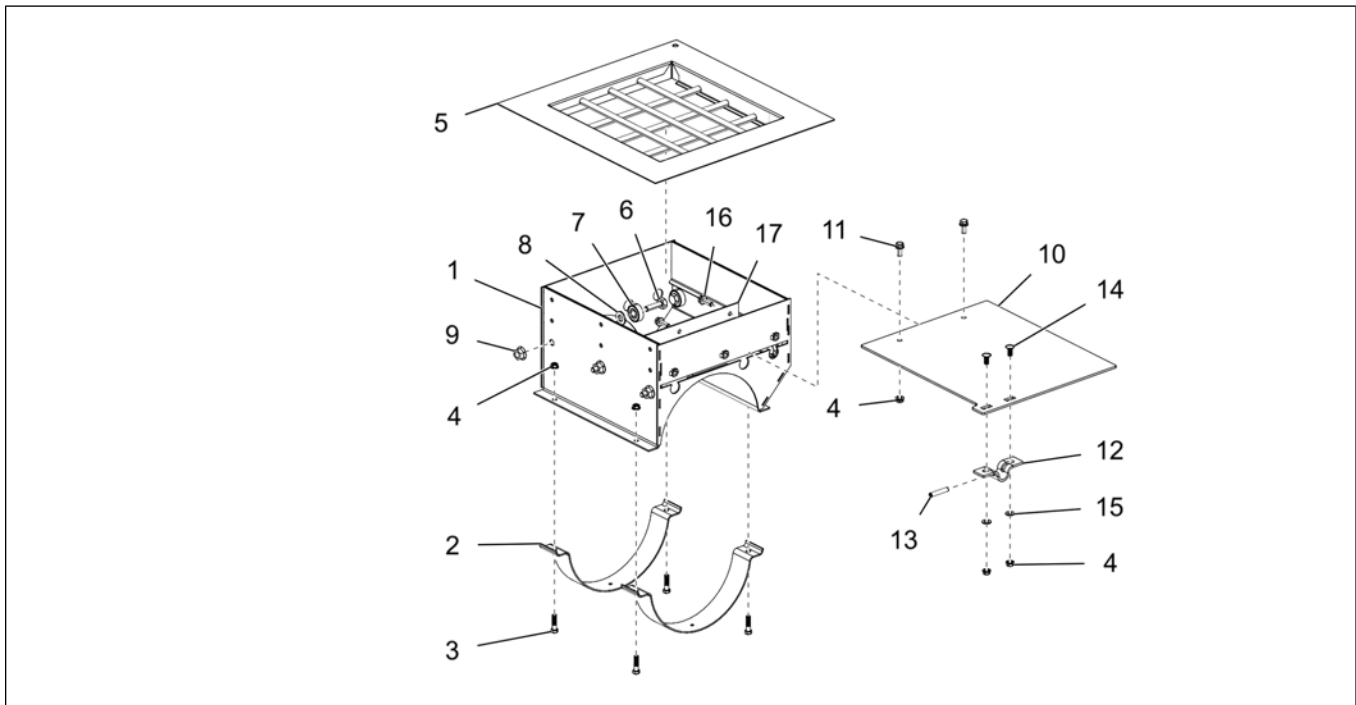
Figure 7-3 Outside intermediate well parts
