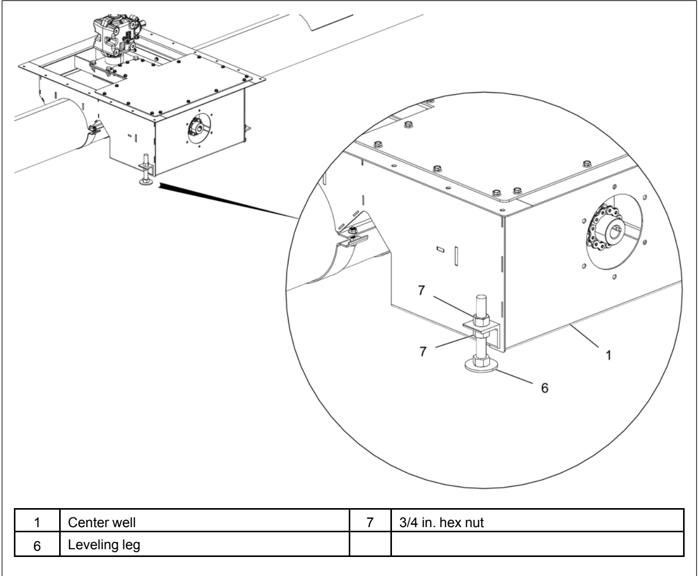
Figure 3-3 Leveling of center well
