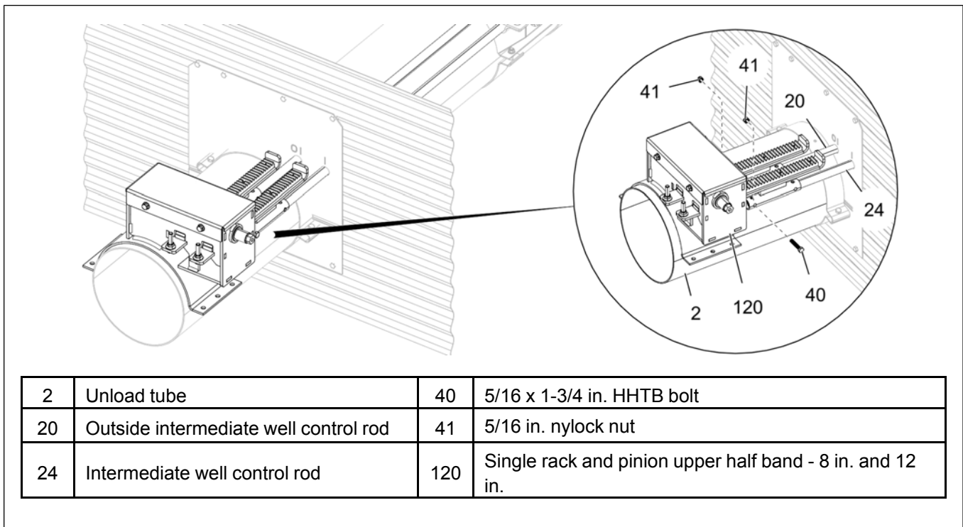
Figure 3-28 Installing the rack and pinion - 8 in. and 12 in. (opposite side)
