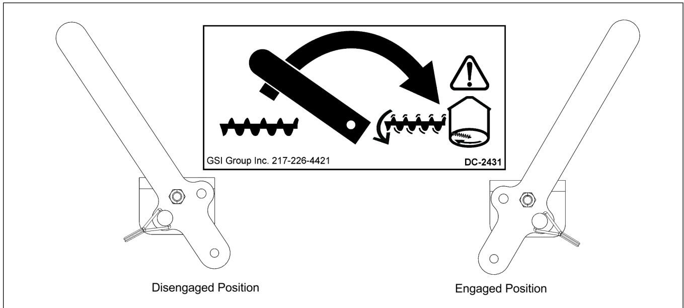
Figure 3-23 Clutch positions
