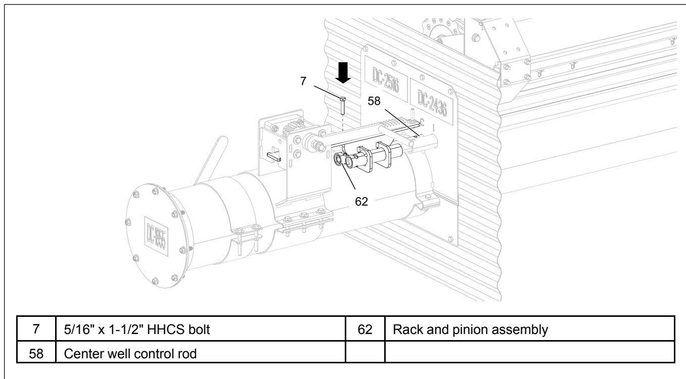
Figure 4-3 Opening the center well gate
